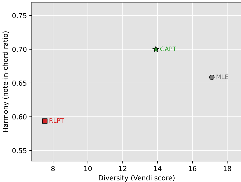
GAPT melody vs chord models unconditioned
