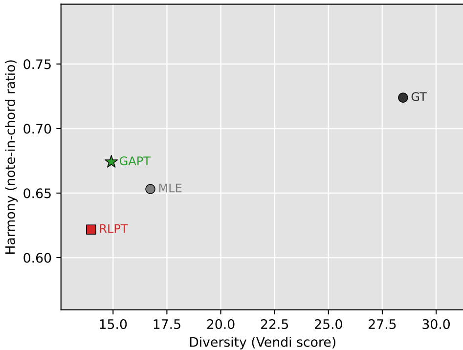
GAPT melody vs chord models with prompt
