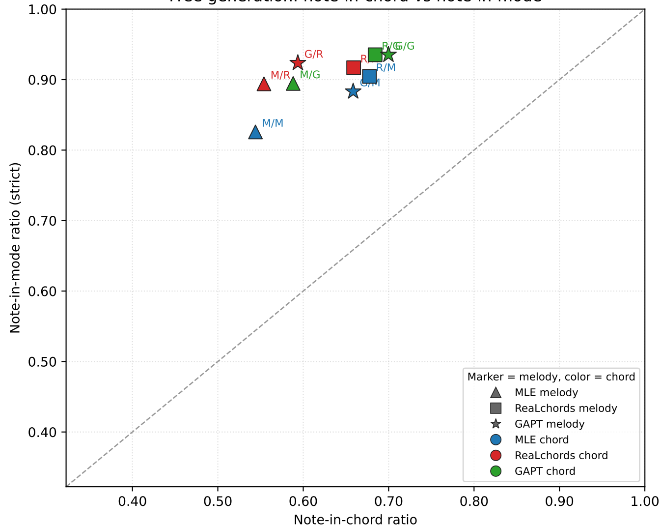
Free generation: note-in-chord vs note-in-mode
