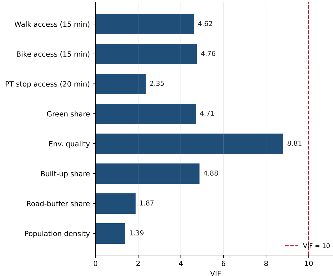
(b) Variance inflation factors (retained GMM features)
