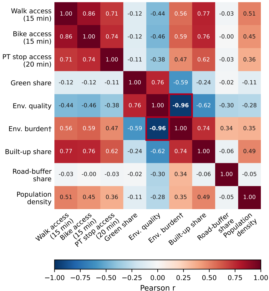
(a) Pearson correlation matrix (candidate GMM features)
