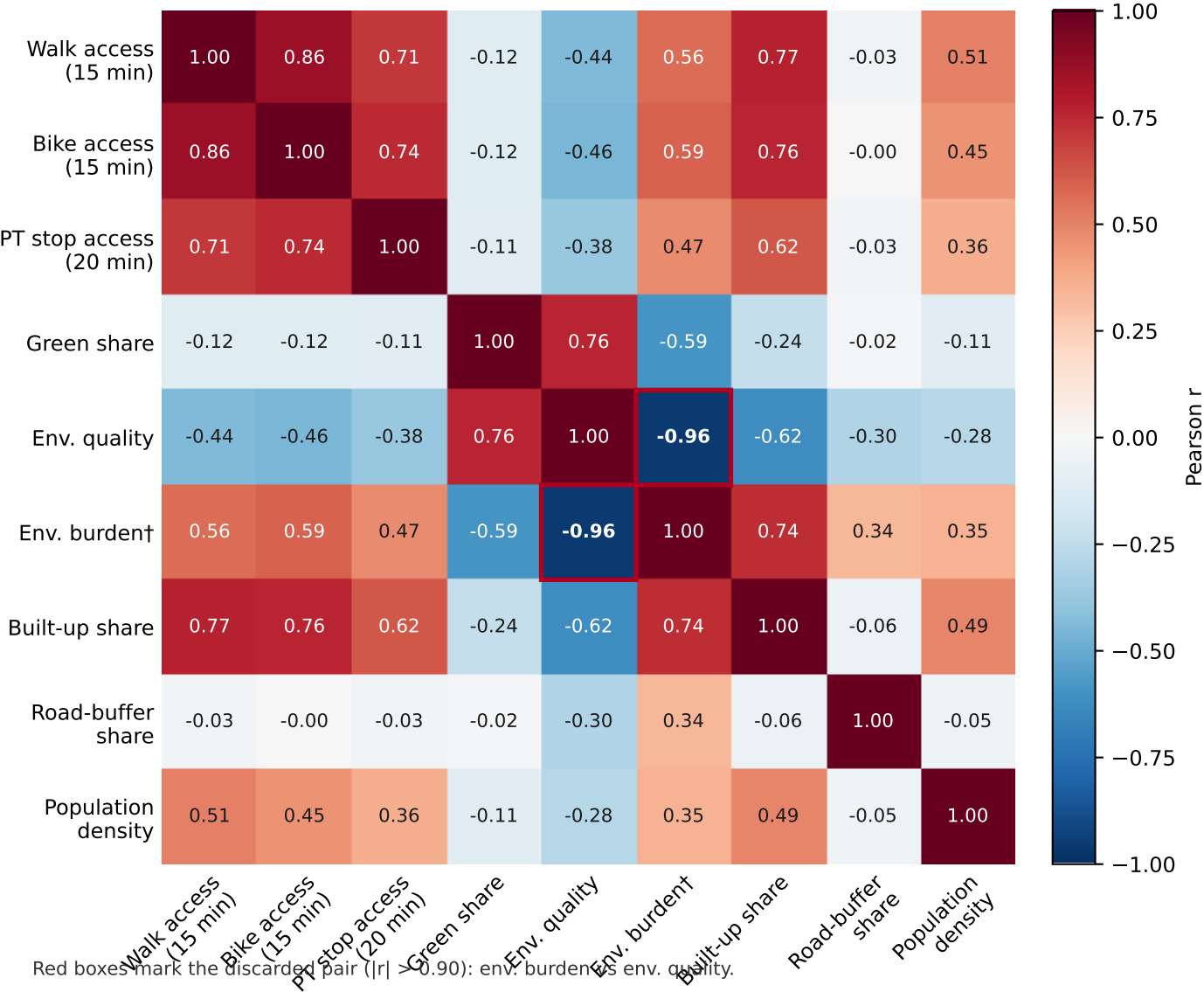
Pearson correlation matrix of candidate GMM features
