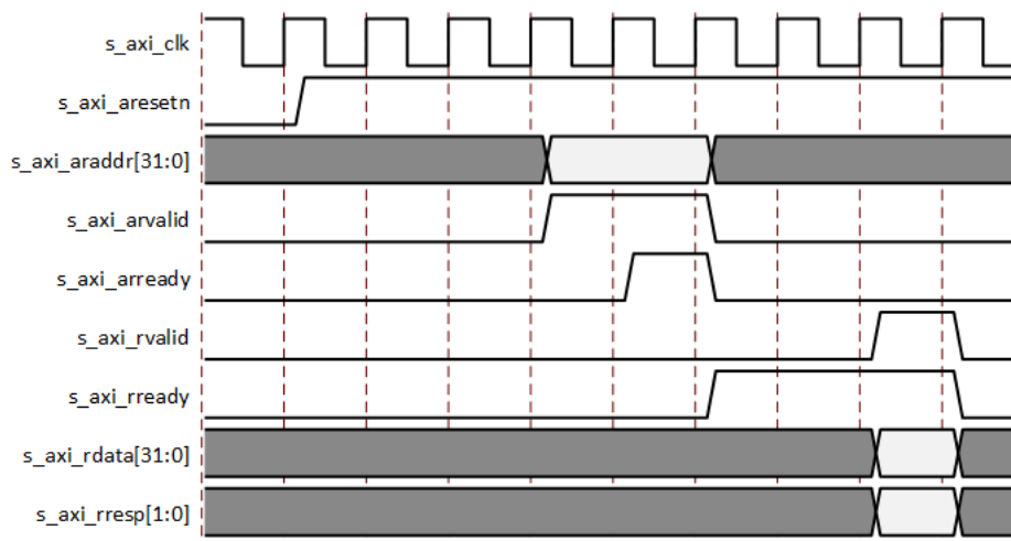
Figure 42: AXI4-Lite Read Timing Diagram
