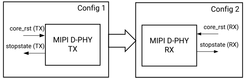
Figure 26: MIPI D-PHY TX and RX System
