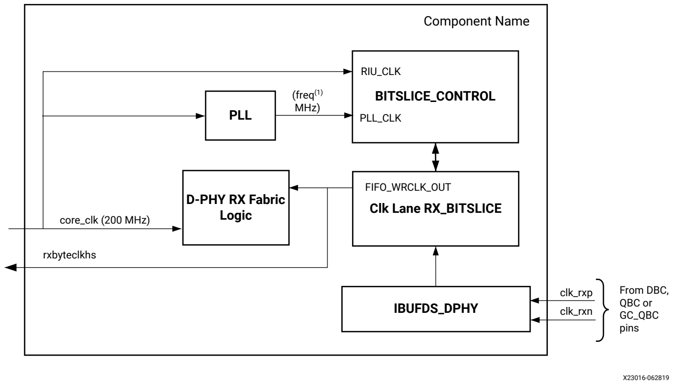
Figure 21: MIPI D-PHY Core RX Clocking for UltraScale+ and Versal Adaptive SoC where Line Rates \leq 1500 Mb/s
