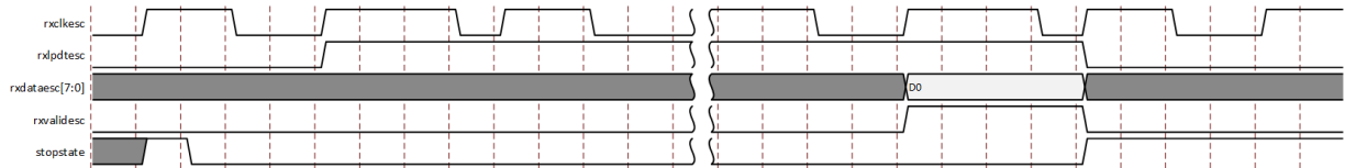
Figure 36: Low-Power Data Reception at the D-PHY RX (Slave)
