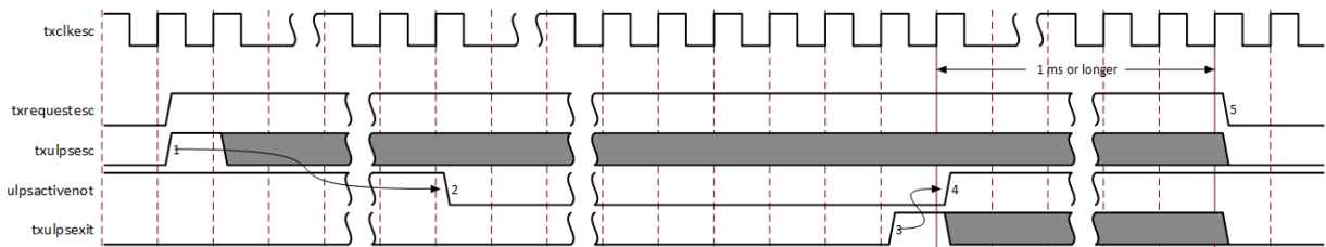
Figure 31: D-PHY TX (Master) ULPS Mode Operation for Data Lane
