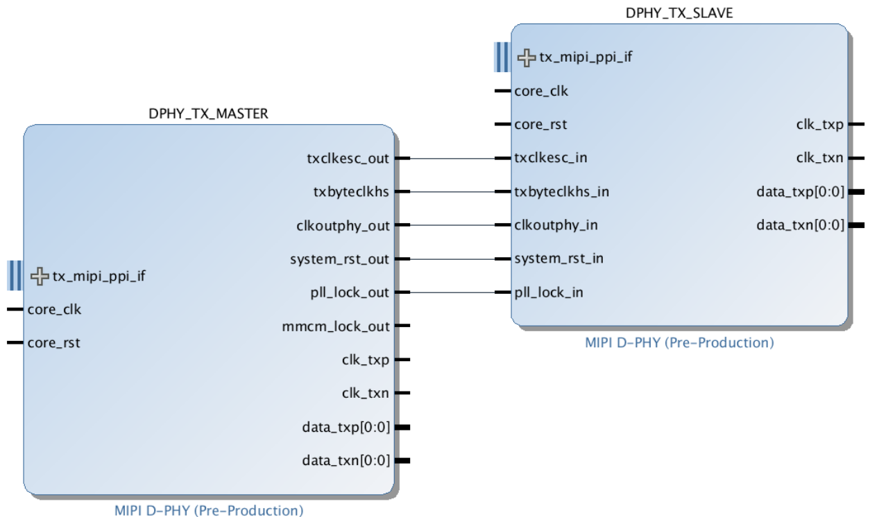
Figure 13: Shared Logic Example for MIPI D-PHY TX Core (Line Rate above 600 Mb/s)
