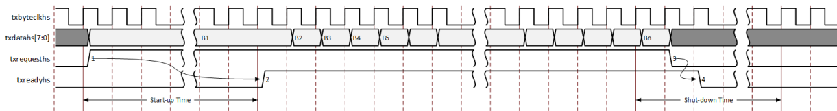
Figure 28: High-Speed Mode Data Transfer from D-PHY TX (Master)
