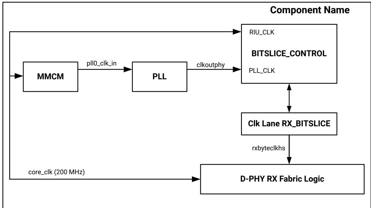
Figure 22: MIPI D-PHY Core RX Clocking for UltraScale+ and Versal Adaptive SoC where Line Rates >1500 Mb/s
