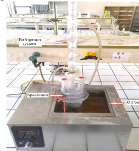
(e) pre-corrosion immersion setup
