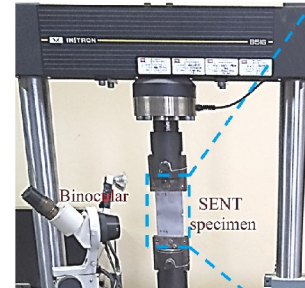
(c) fatigue machine
