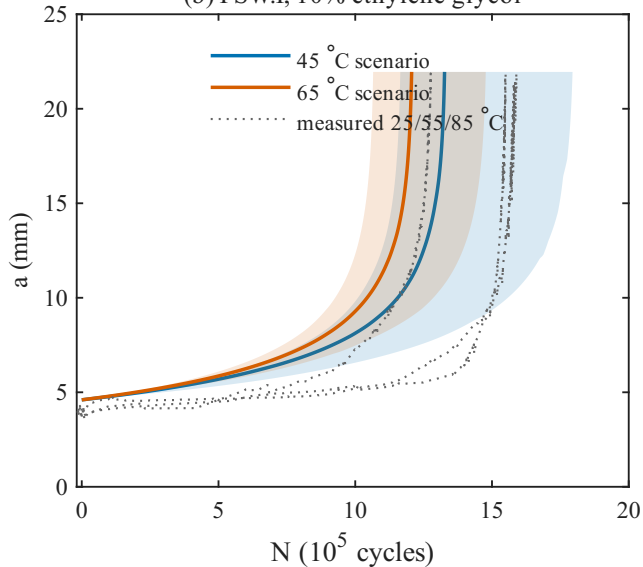
(b) FSW.I, 10% ethylene glycol
