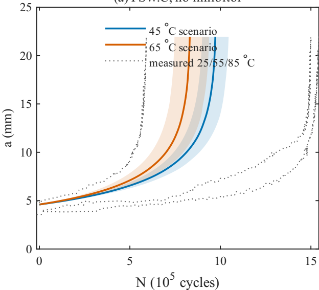
(a) FSW.C, no inhibitor
