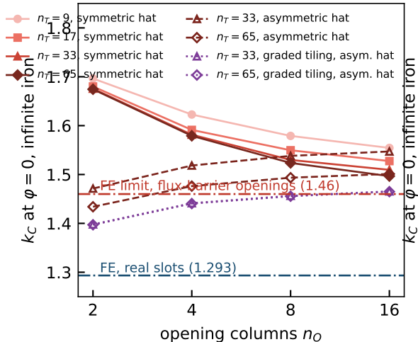
(a) operator with \Phi_O = 0
