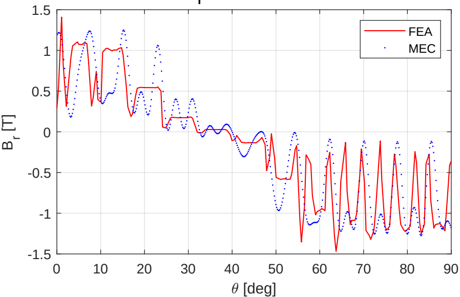
(a) B_r at mid-gap, no load
