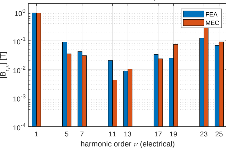
(c) Spatial spectrum of B_r (no load)
