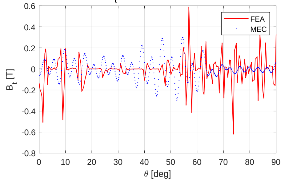
(b) B_t at mid-gap, no load (P1)
