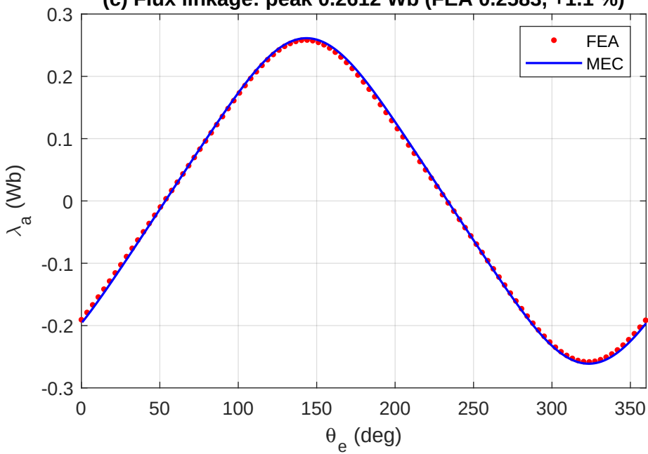
(c) Flux linkage: peak 0.2612 Wb (FEA 0.2583, +1.1 %)
