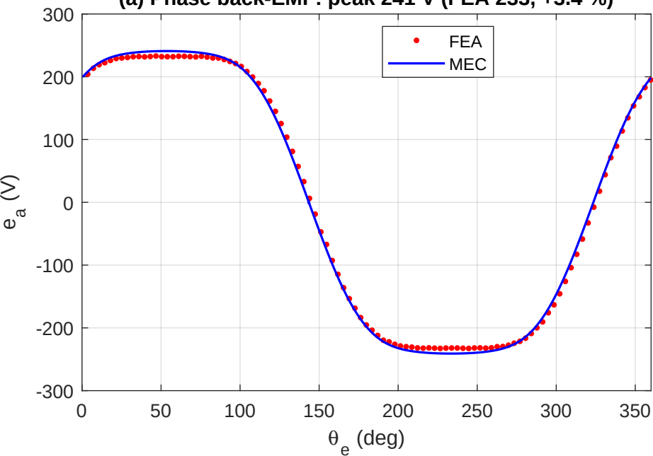
(a) Phase back-EMF: peak 241 V (FEA 233, +3.4 %)
