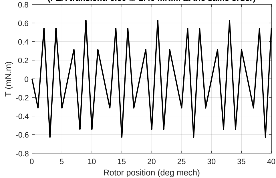
(d) Physical cogging only: 1.26 mN.m p-p, order 210 (FEA transient: 0.60 \pm 1.40 mN.m at the same order)
