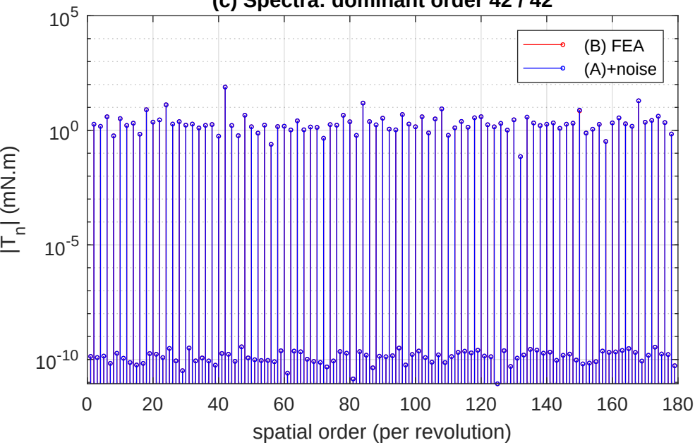
(c) Spectra: dominant order 42 / 42
