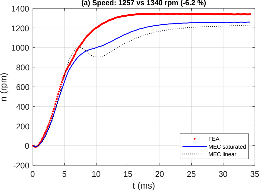
(a) Speed: 1257 vs 1340 rpm (-6.2 %)
