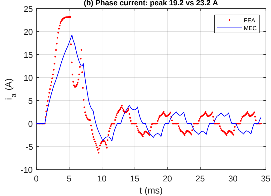
(b) Phase current: peak 19.2 vs 23.2 A
