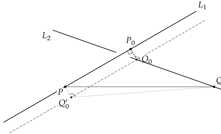
Figura 6.5: Rette sghembe
