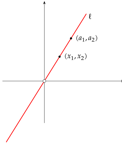
Figura 7.1: Coordinate omogenee
