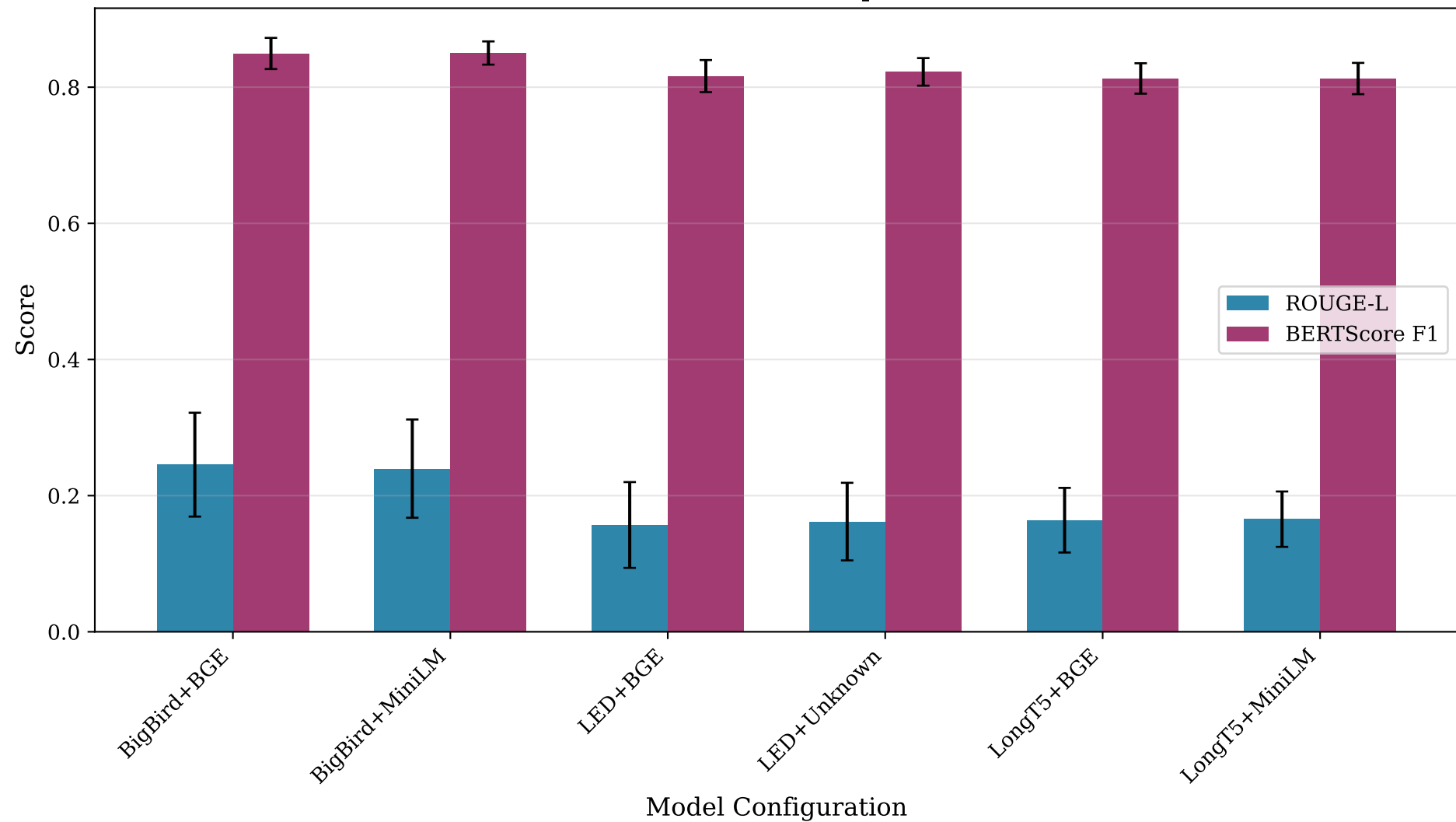
Chunk Retrieval Model Comparison - ARXIV
