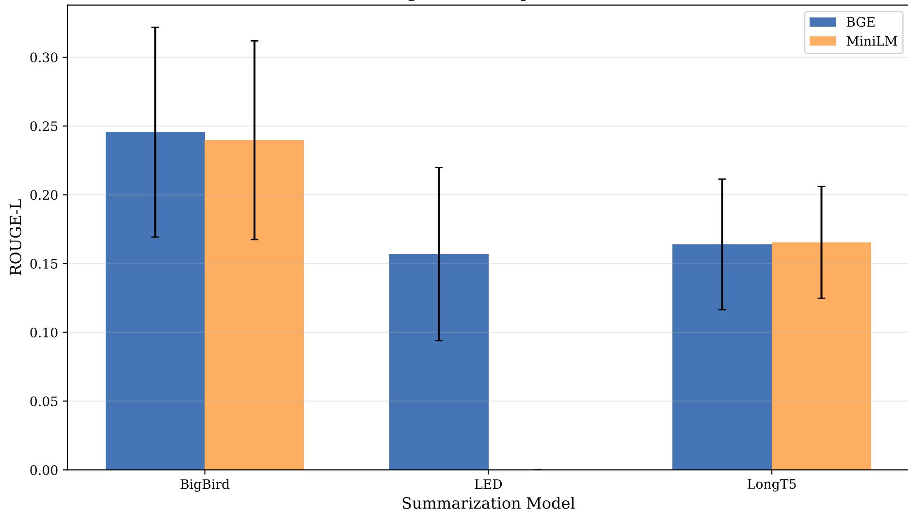
Embedding Model Comparison - ARXIV
