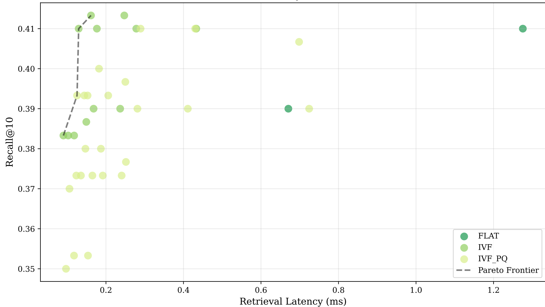
FAISS Recall-Latency Trade-off - ARXIV
