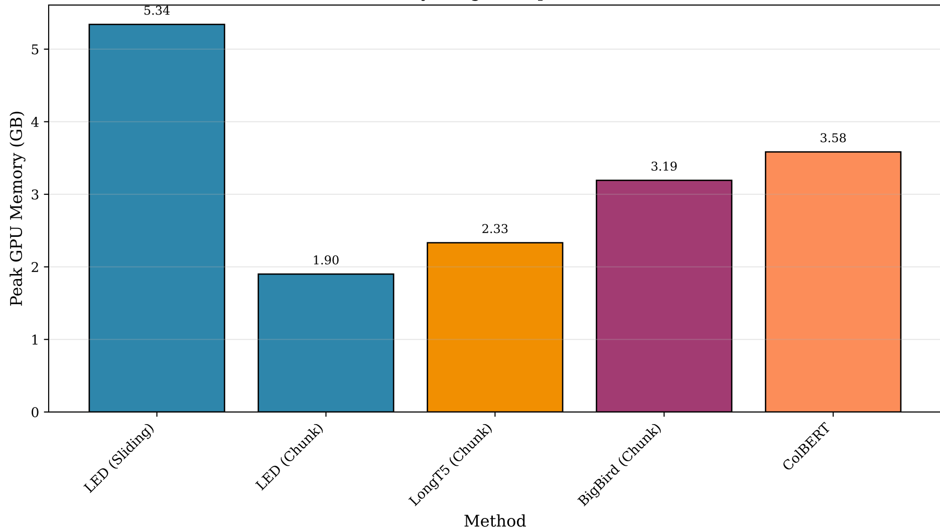
GPU Memory Usage Comparison - ARXIV
