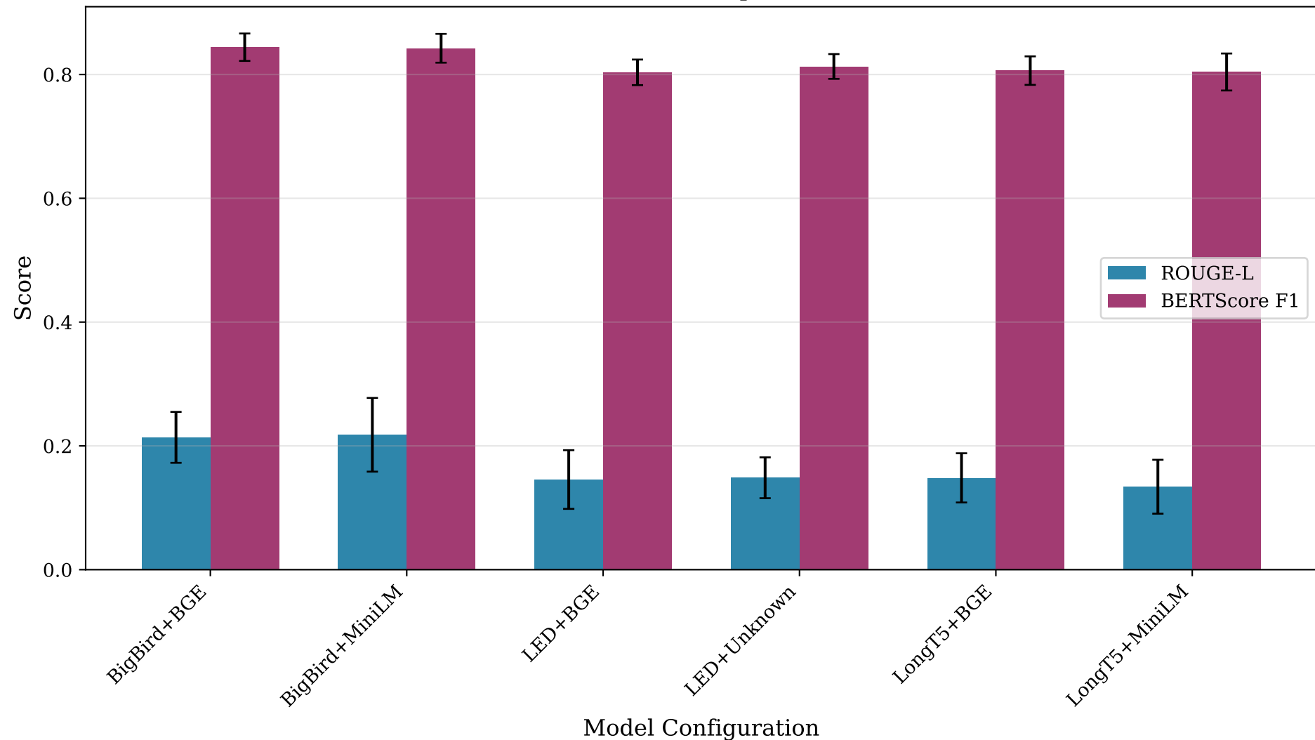
Chunk Retrieval Model Comparison - LONGFORM
