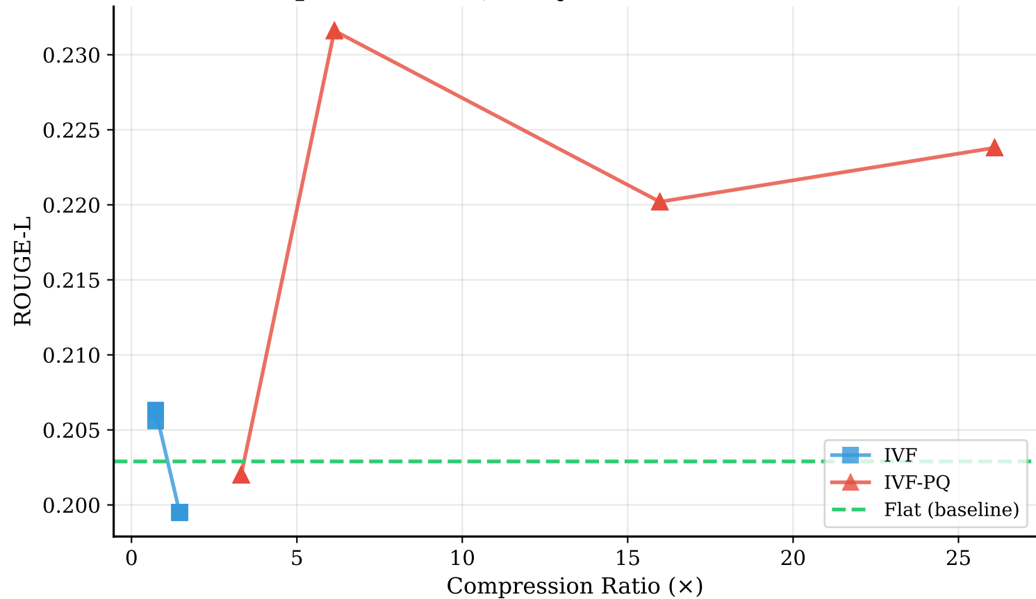
Compression vs Quality Trade-off - LONGFORM
