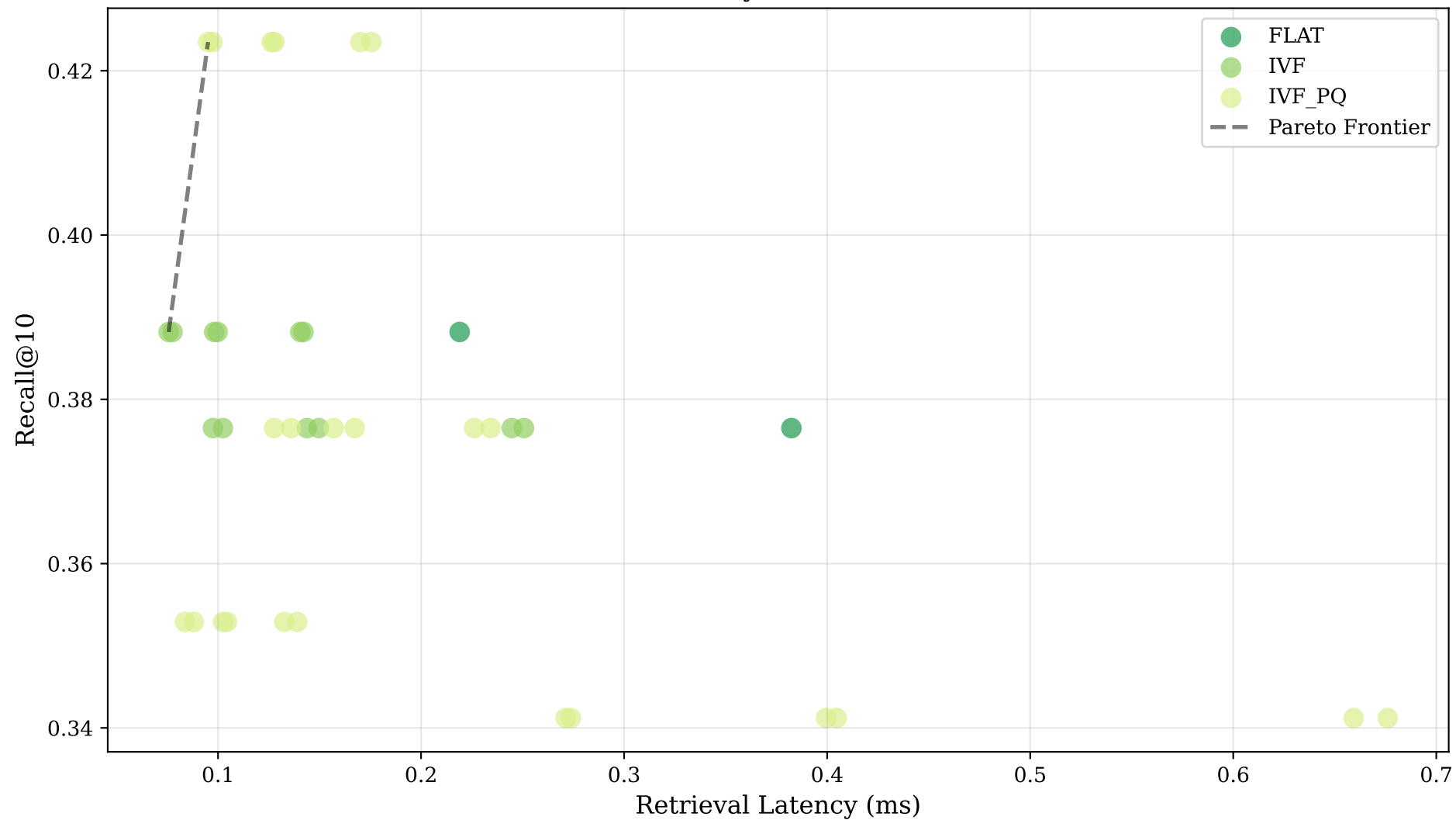
FAISS Recall-Latency Trade-off - LONGFORM
