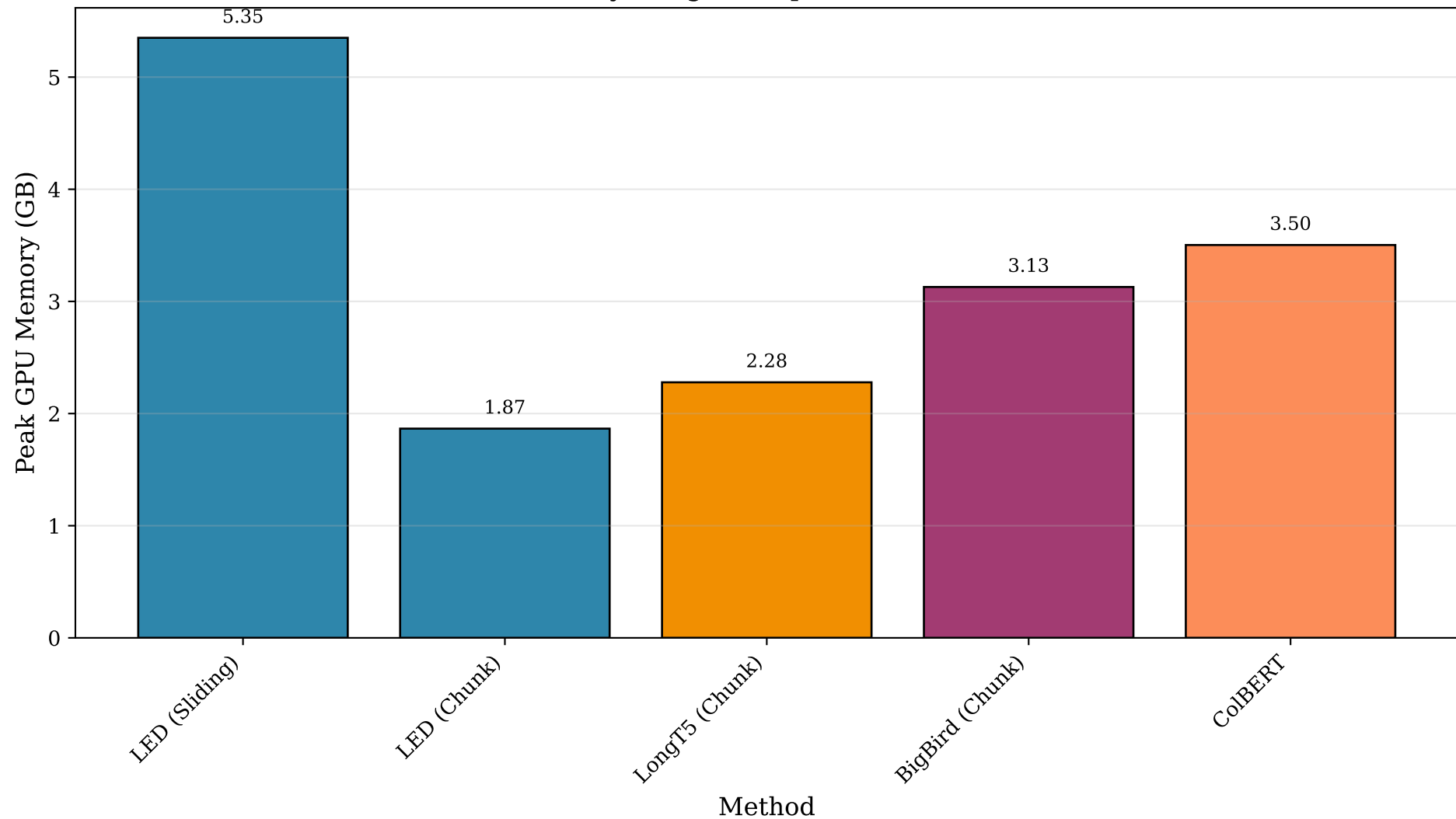
GPU Memory Usage Comparison - LONGFORM
