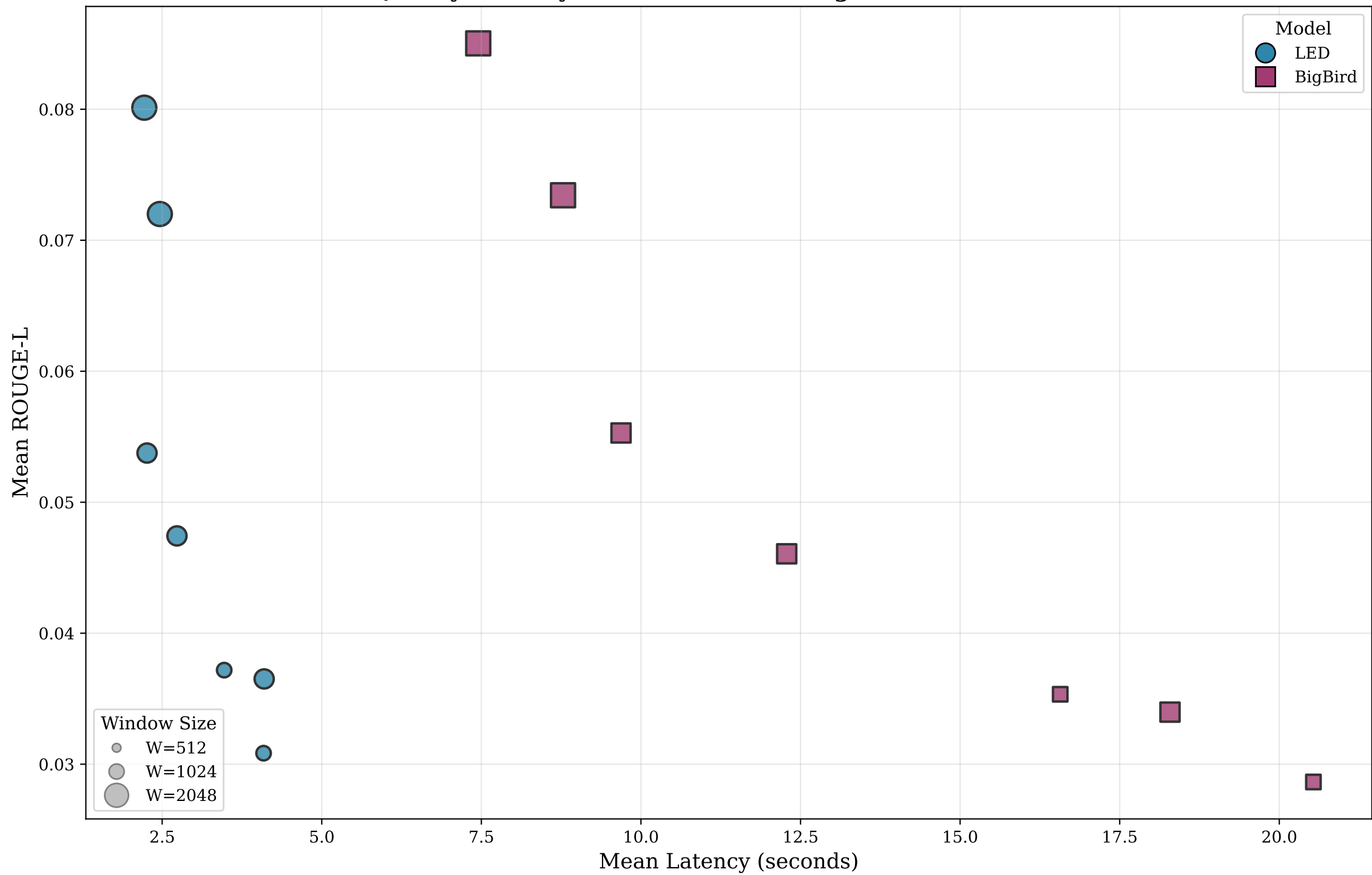
Quality-Latency Trade-off: LED vs BigBird - LONGFORM
