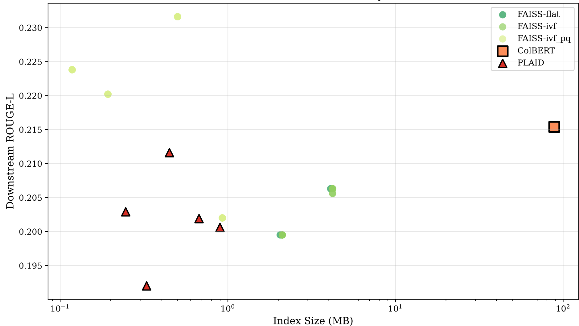
Retrieval Methods: Index Size vs Quality - LONGFORM
