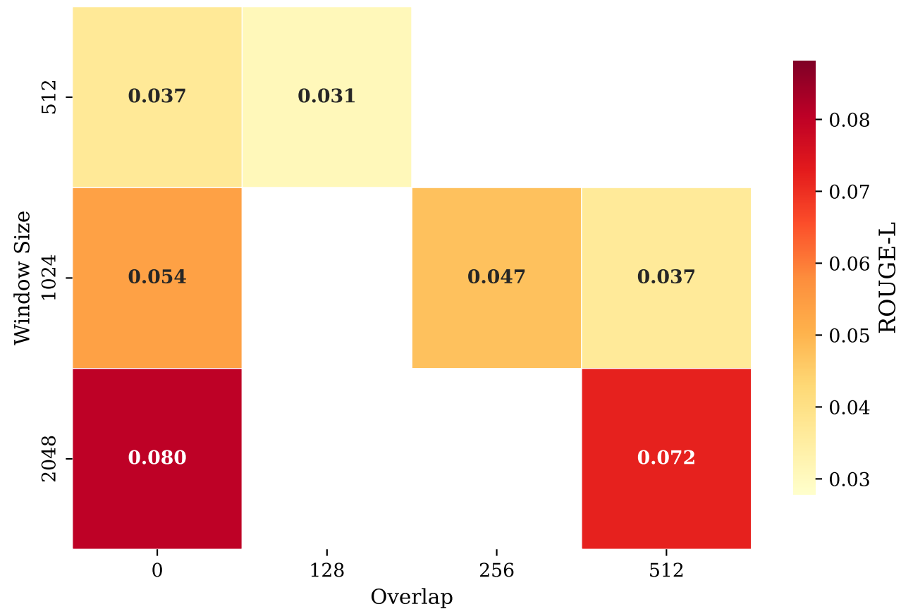
LED - LONGFORM
