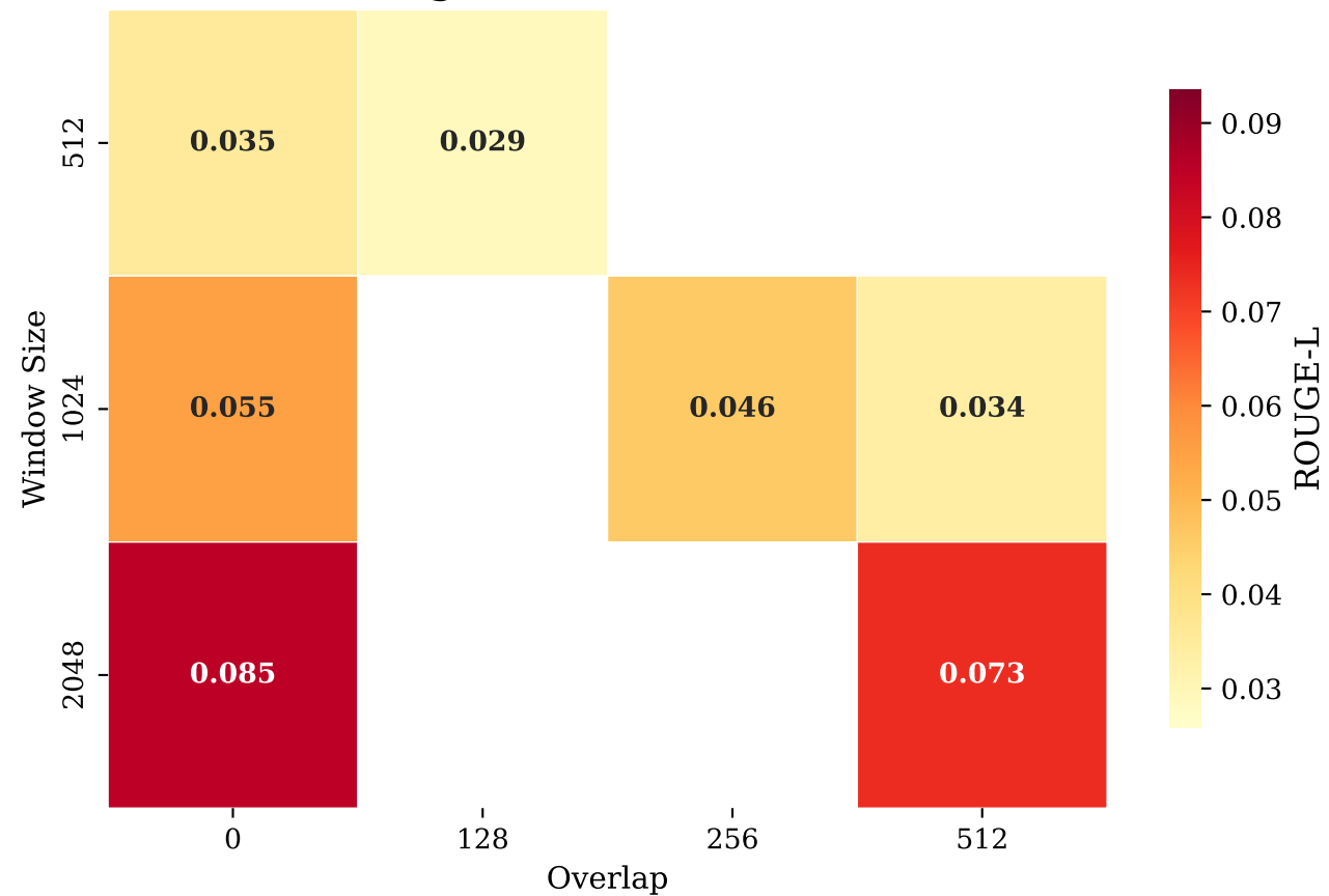
BigBird - LONGFORM
