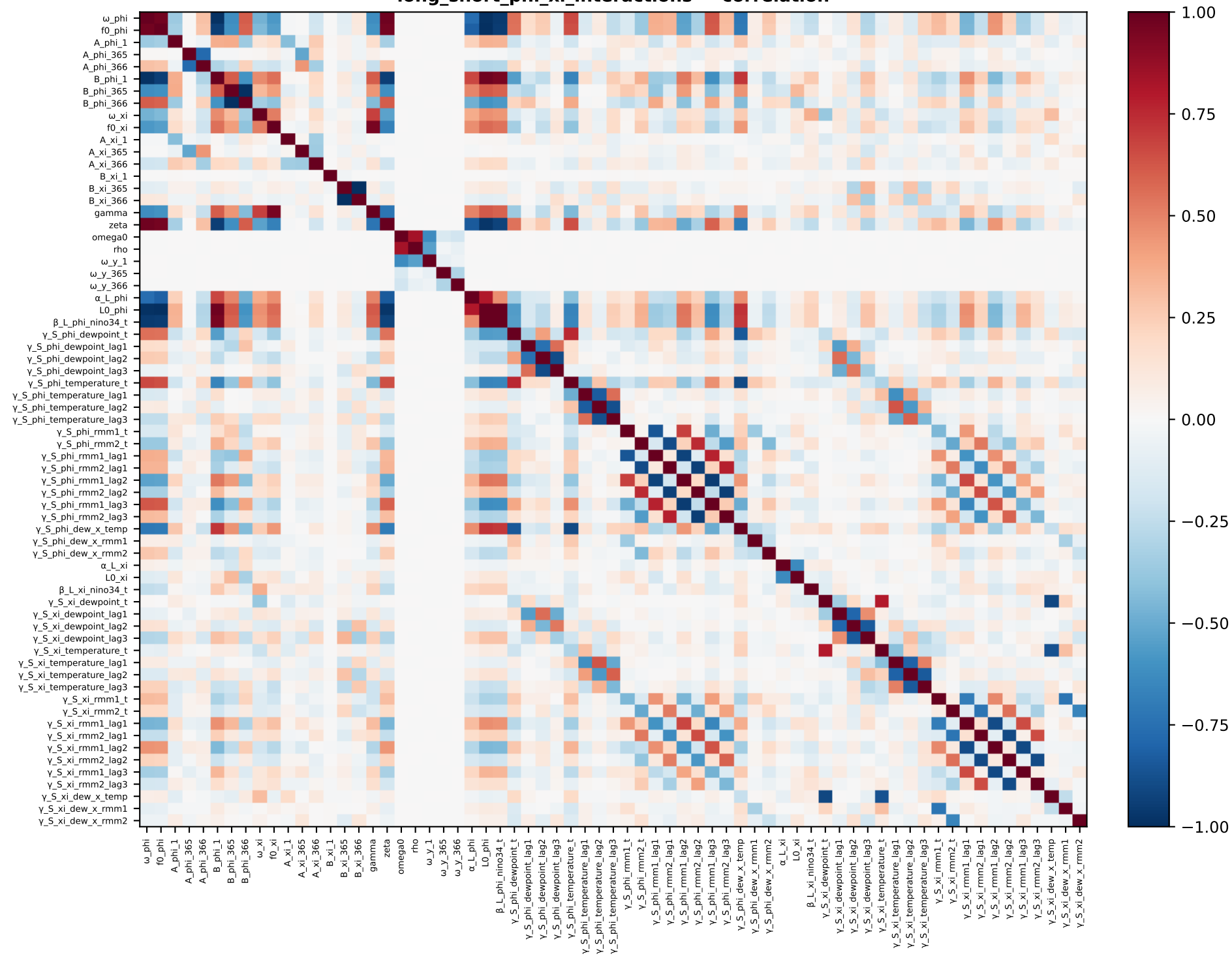
long_short_phi_xi_interactions — correlation
