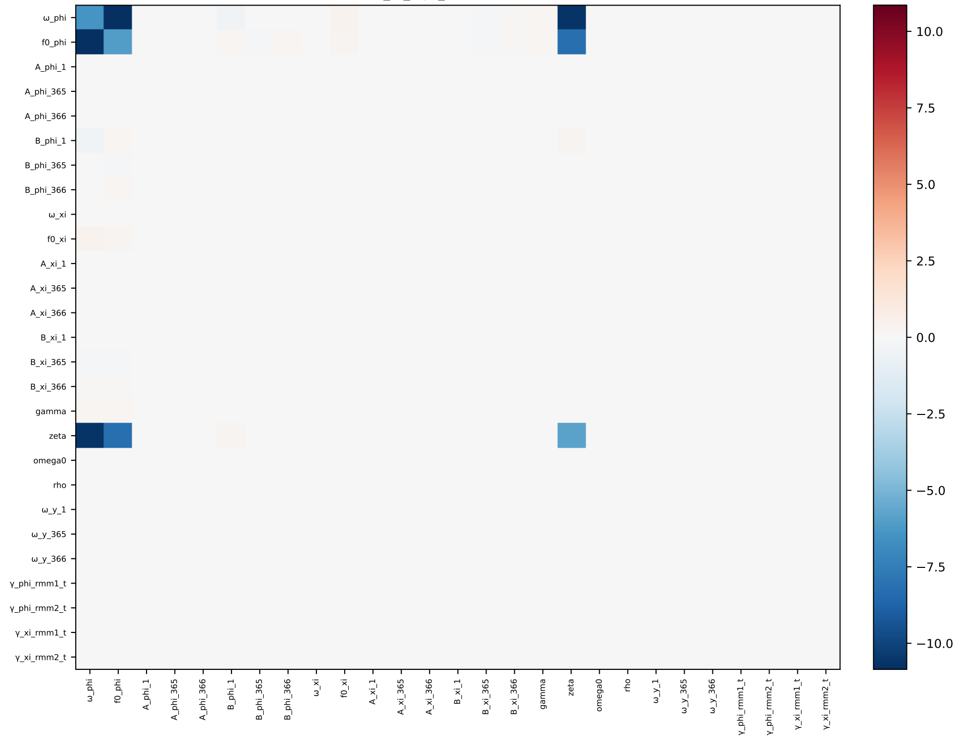
phi xi mjo t — covariance
