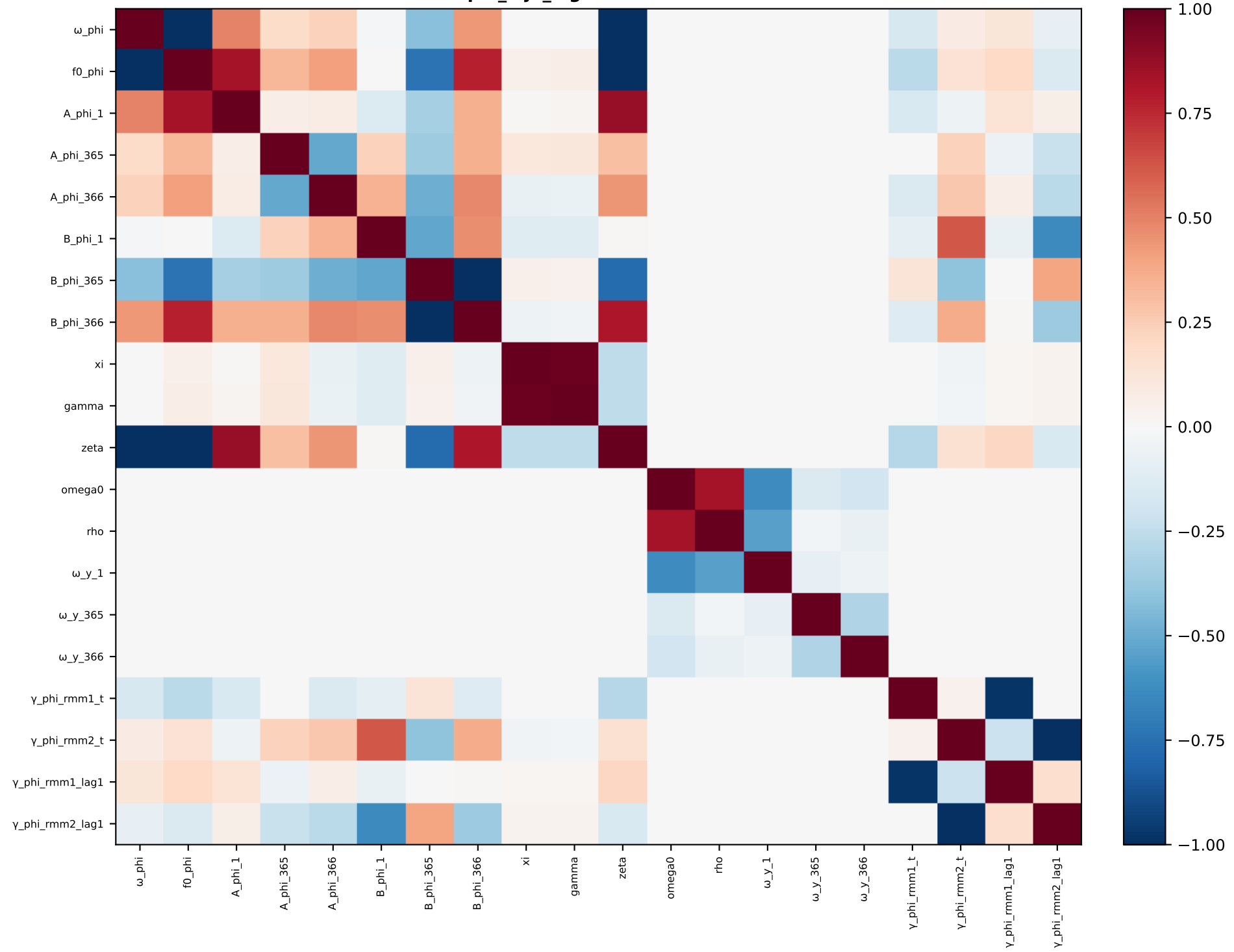
phi_mjo_lag1 — correlation
