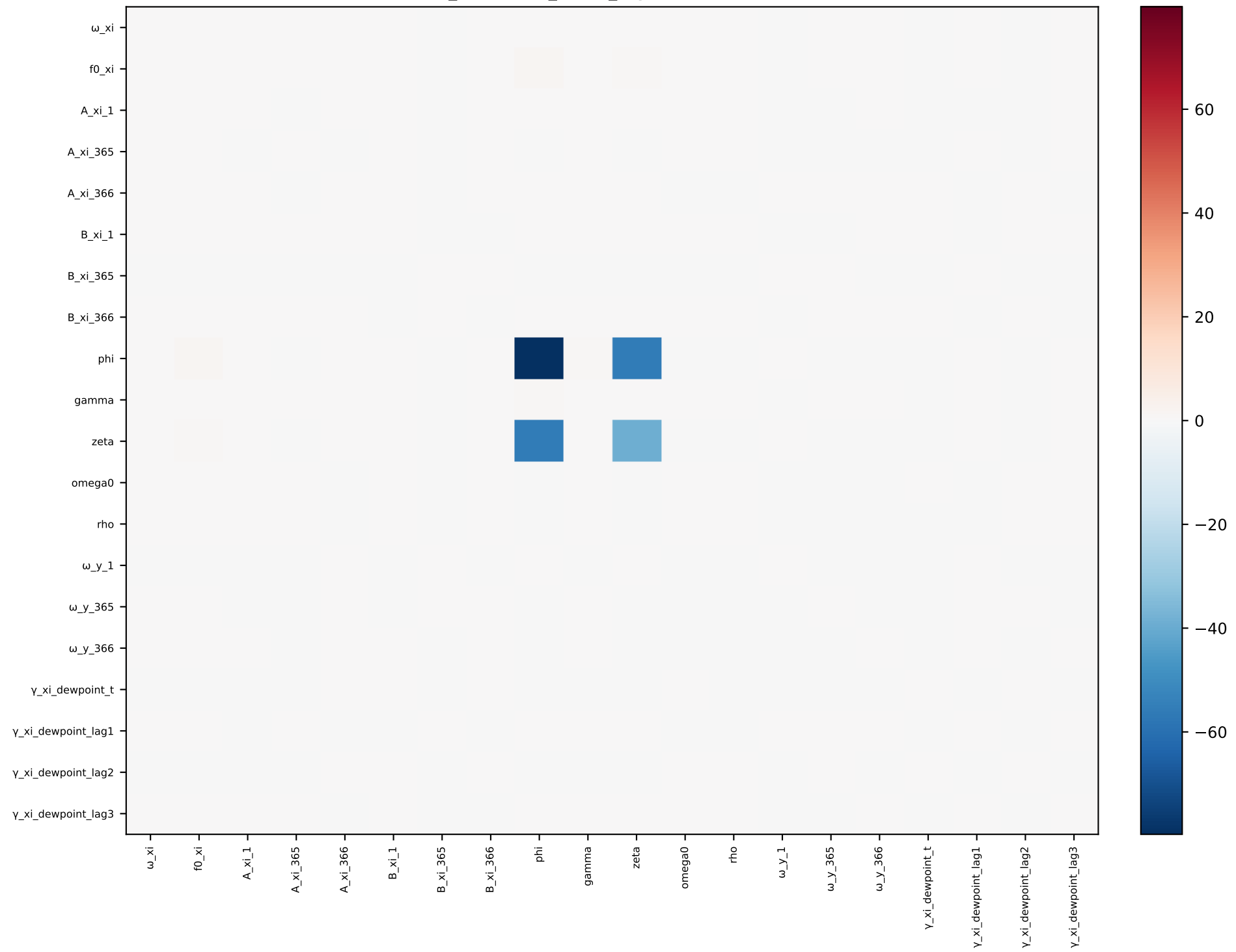
xi_dewpoint_short_lags — covariance
