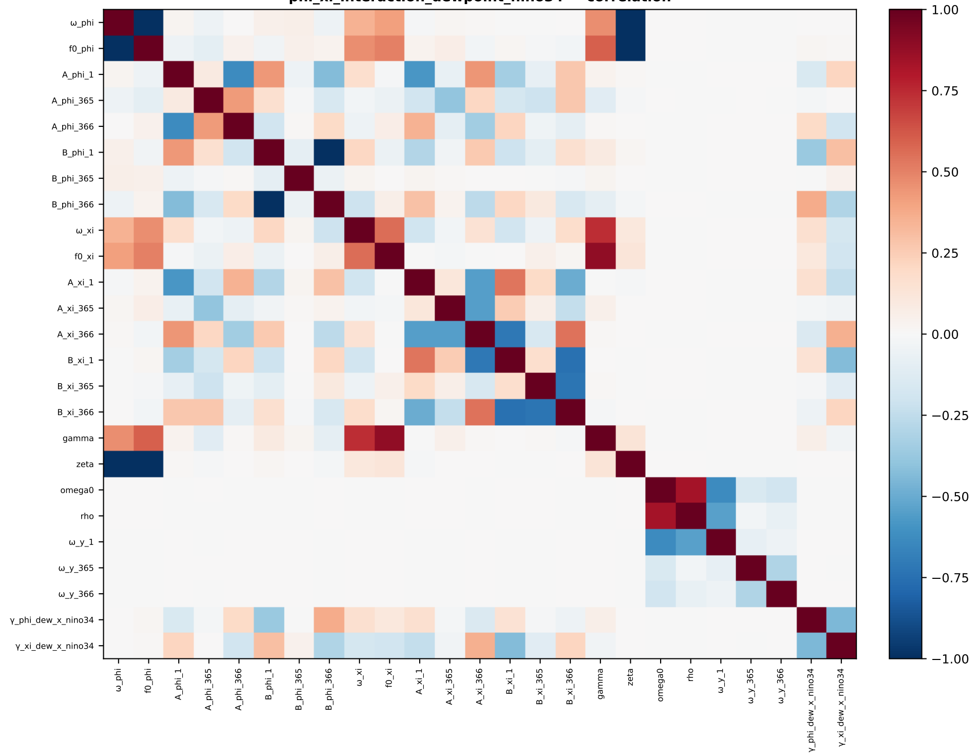
phi_xi_interaction_dewpoint_nino34 — correlation
