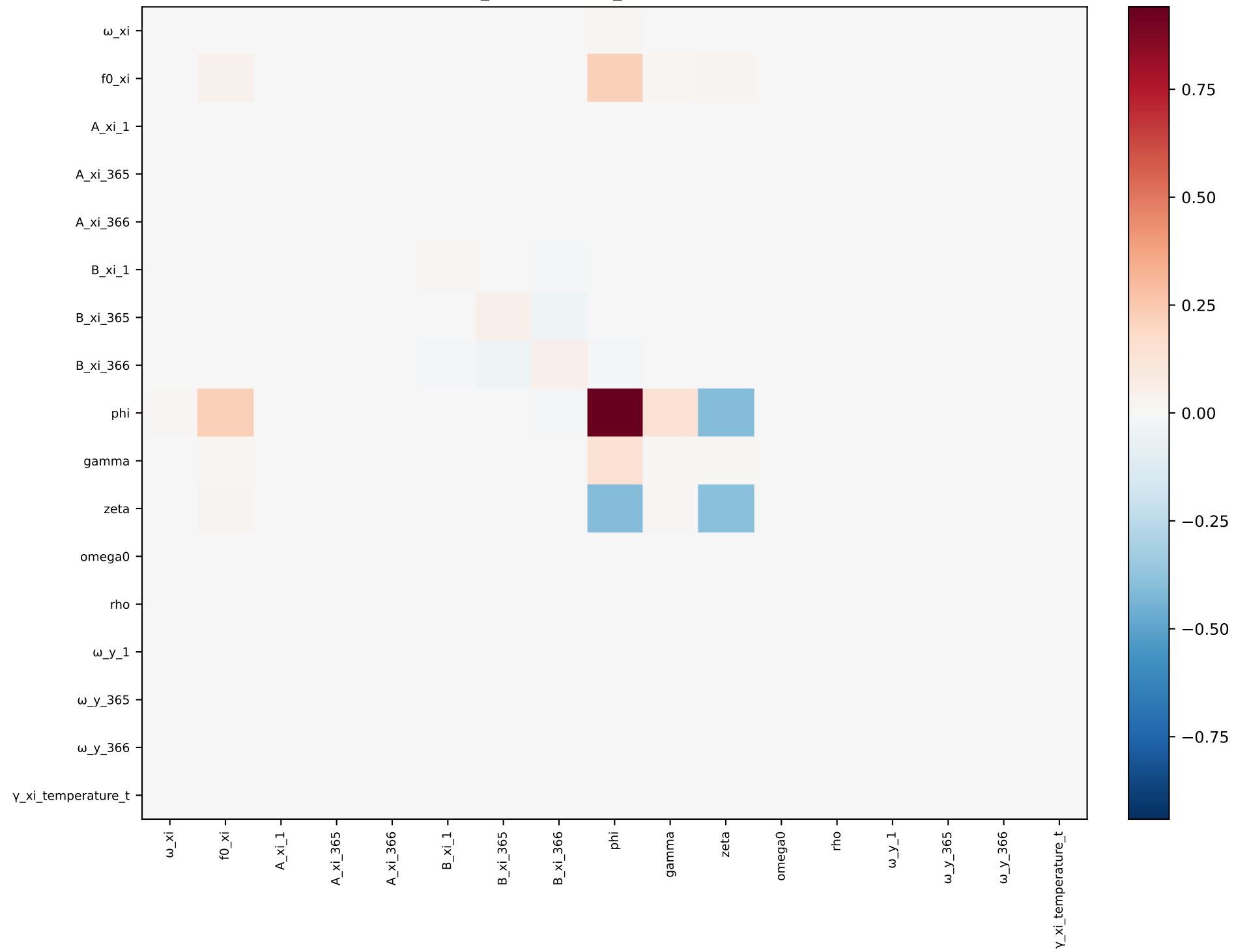
xi_temperature_t — covariance
