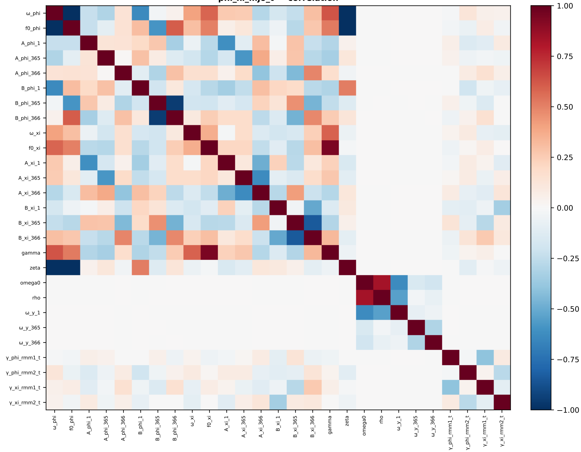
phi_xi_mjo_t — correlation
