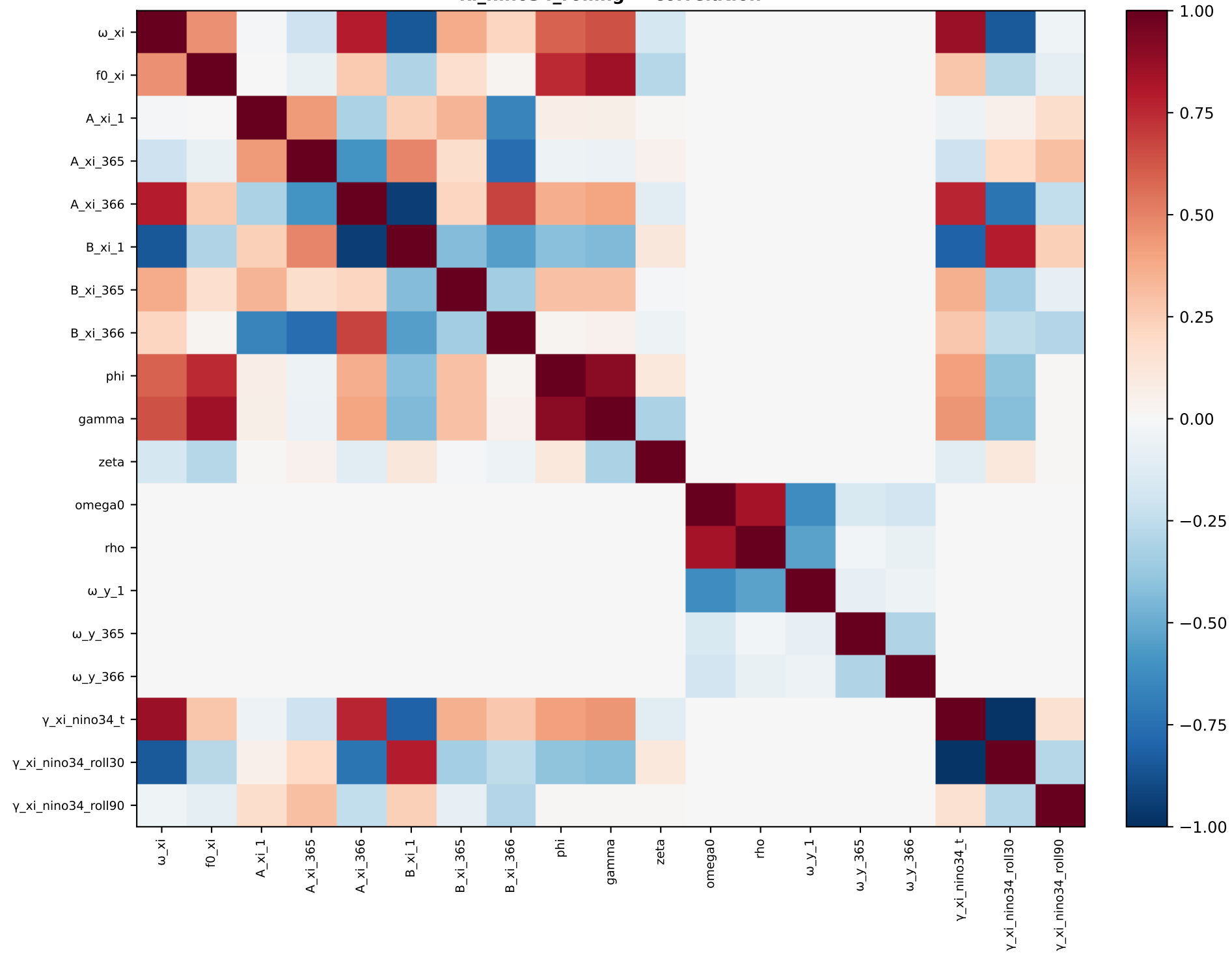
xi_nino34_rolling — correlation
