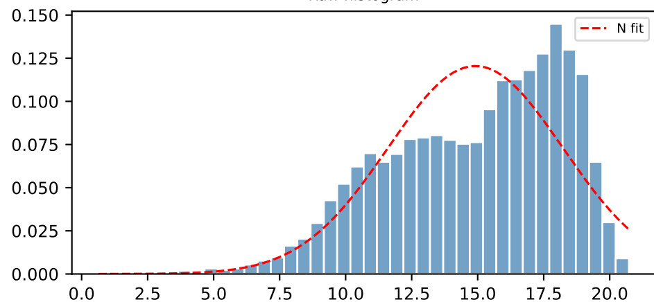
Raw histogram
