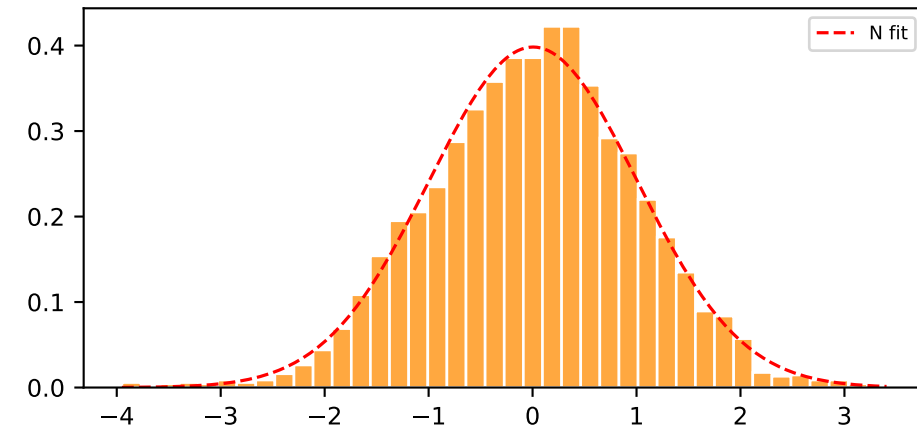
Normalised histogram
