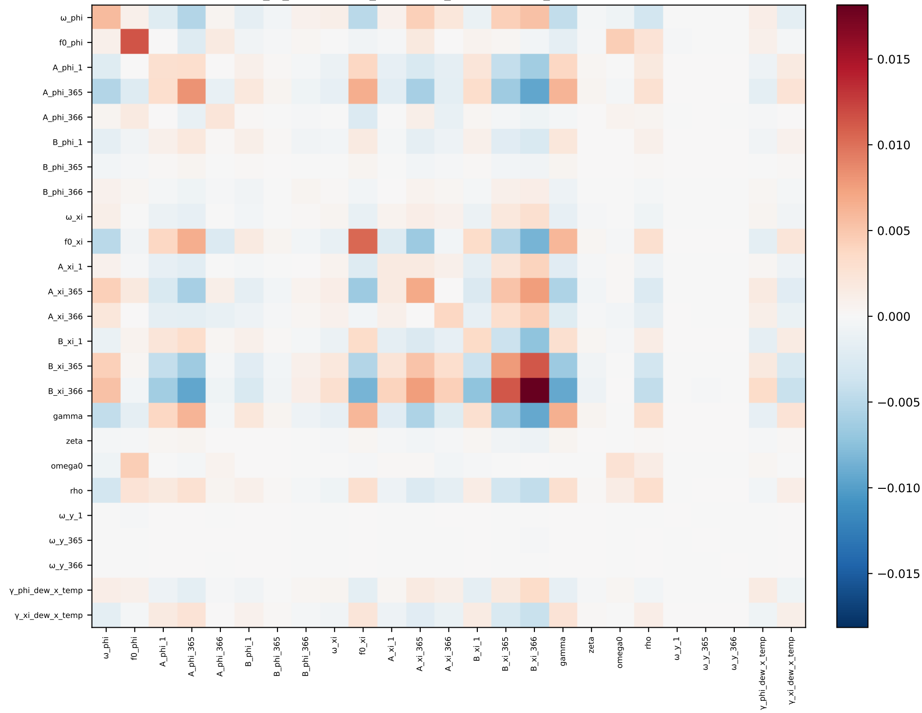
phi_xi_interaction_dewpoint_temperature_t — covariance
