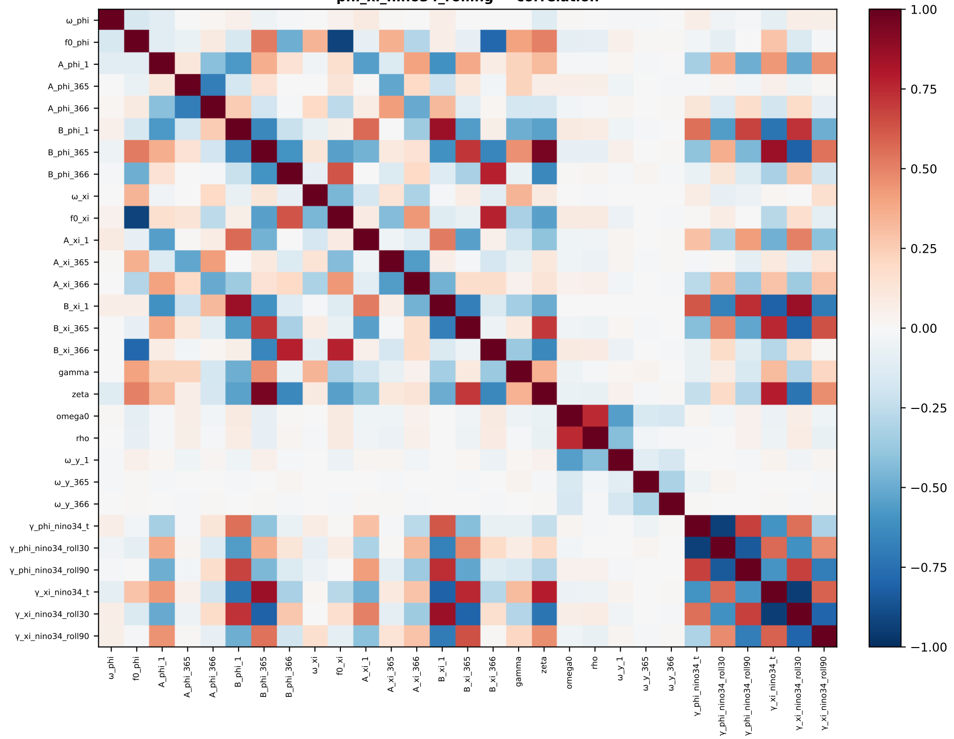
phi_xi_nino34_rolling — correlation
