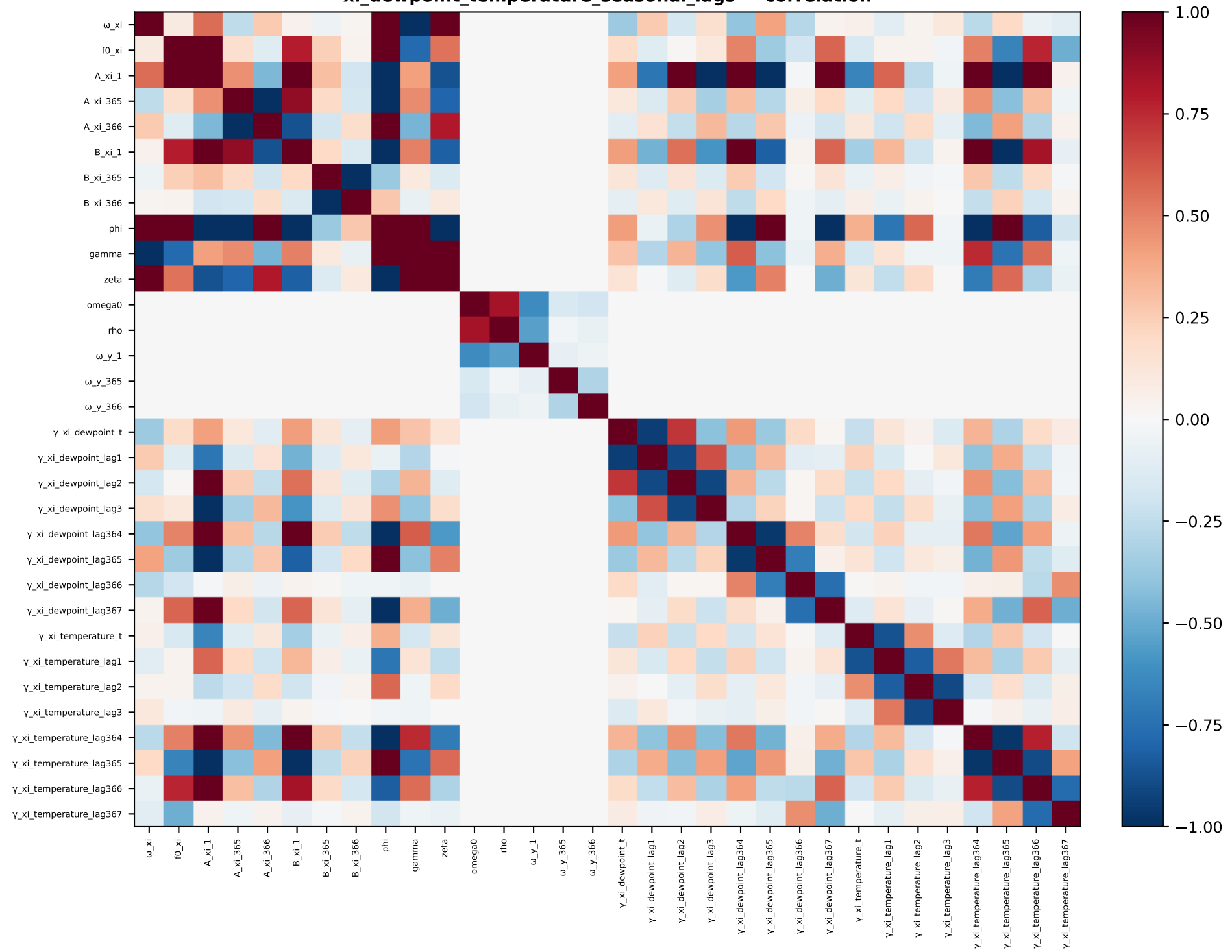
xi_dewpoint_temperature_seasonal_lags — correlation
