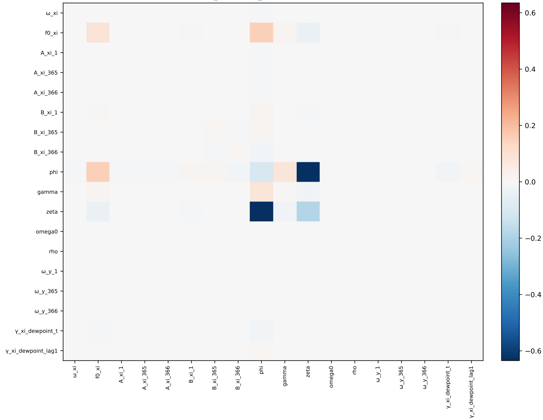
xi_dewpoint_lag1 — covariance
