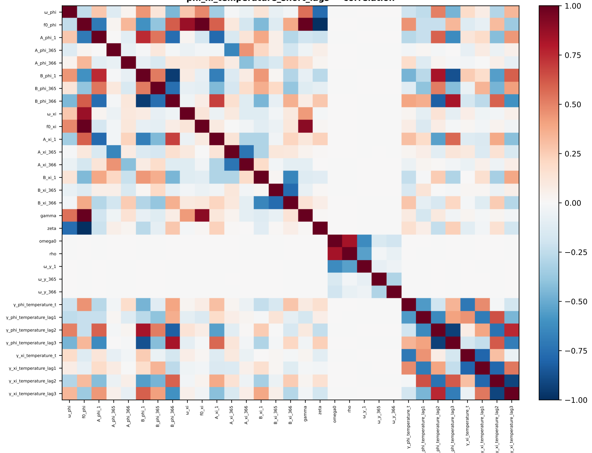
phi_xi_temperature_short_lags — correlation
