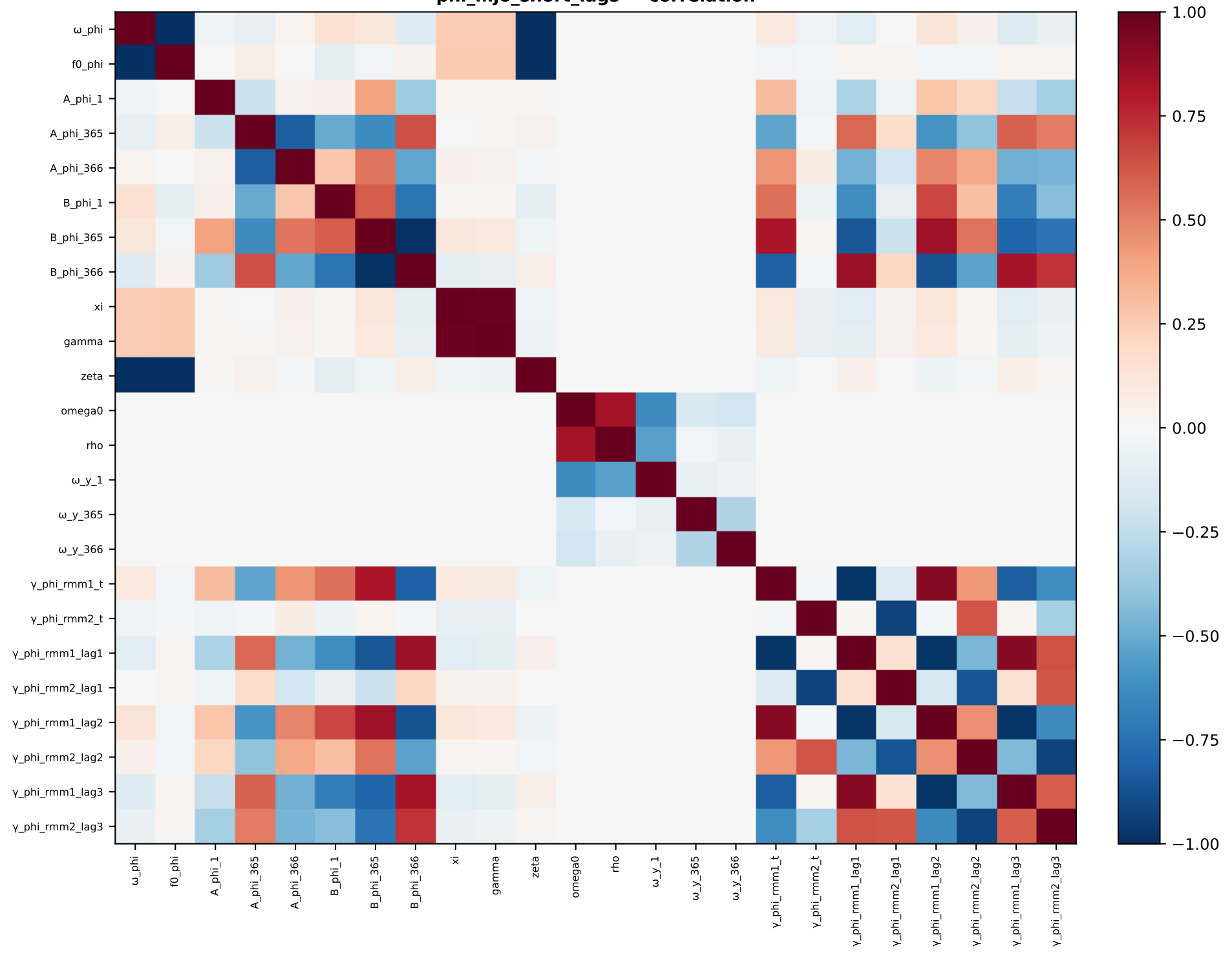
phi_mjo_short_lags — correlation
