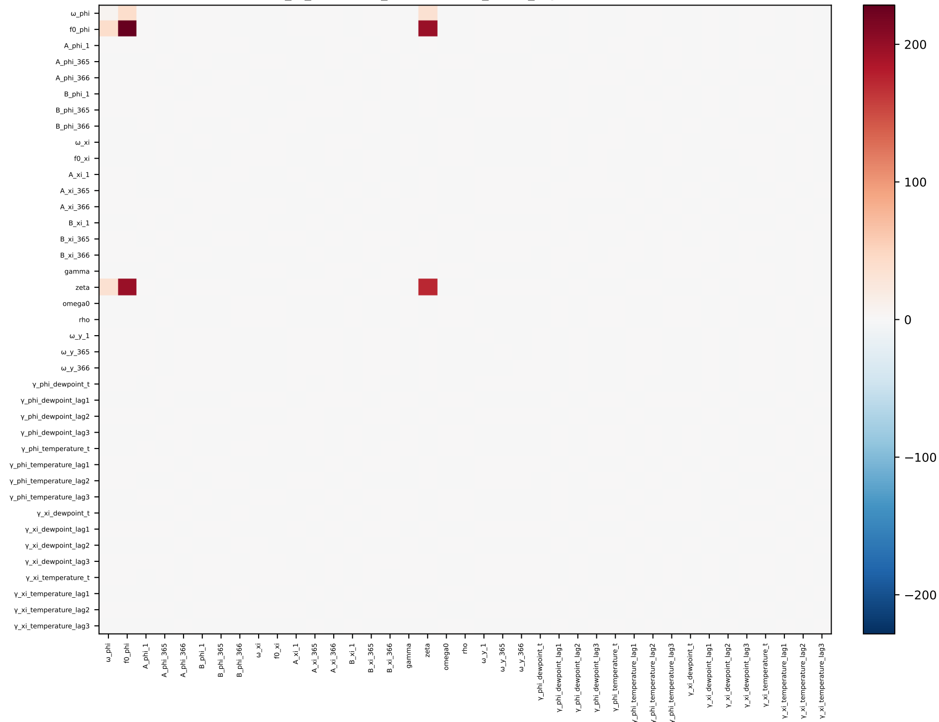
phi_xi_dewpoint_temperature_short_lags — covariance
