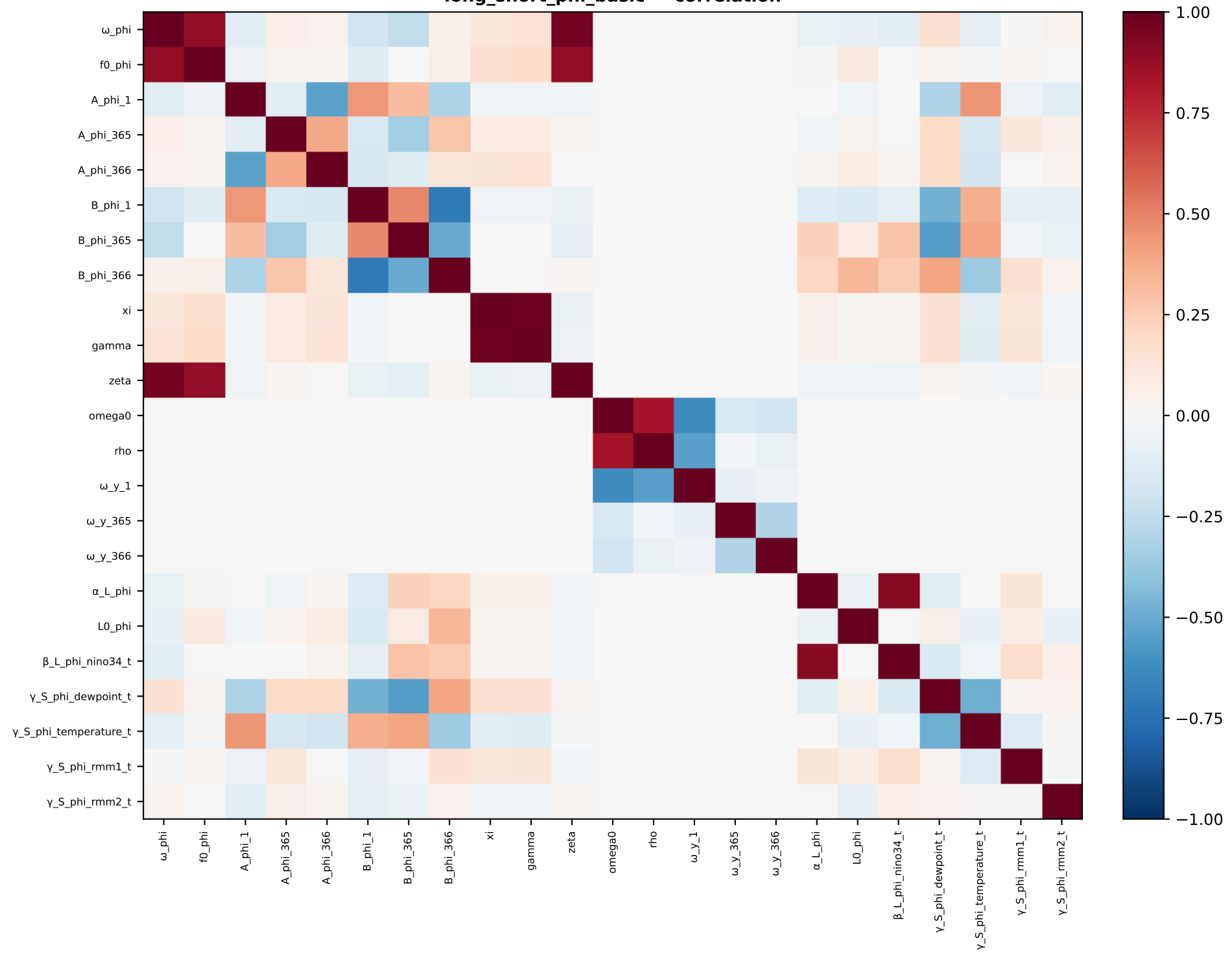
long_short_phi_basic — correlation
