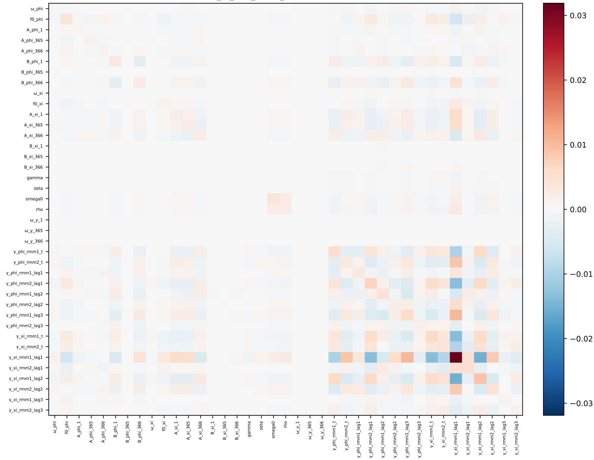
phi_xi_mjo_short_lags — covariance
