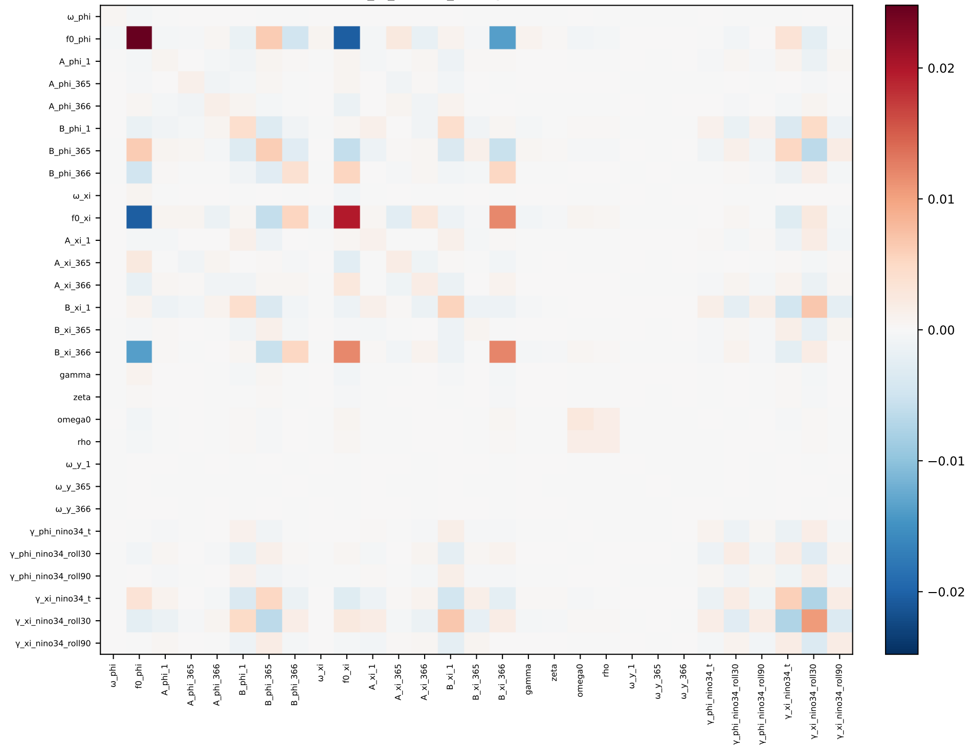
phi_xi_nino34_rolling — covariance
