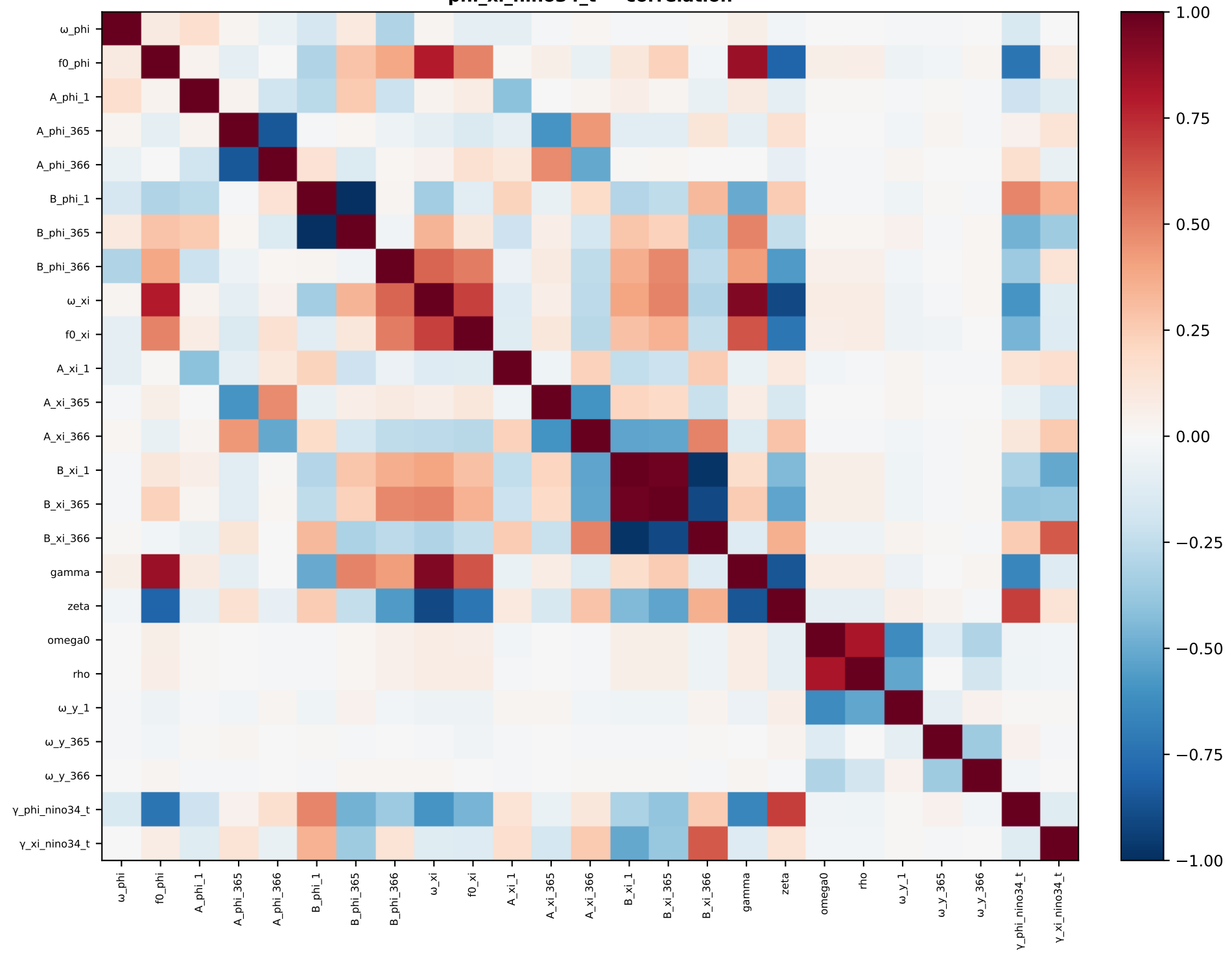
phi_xi_nino34_t — correlation
