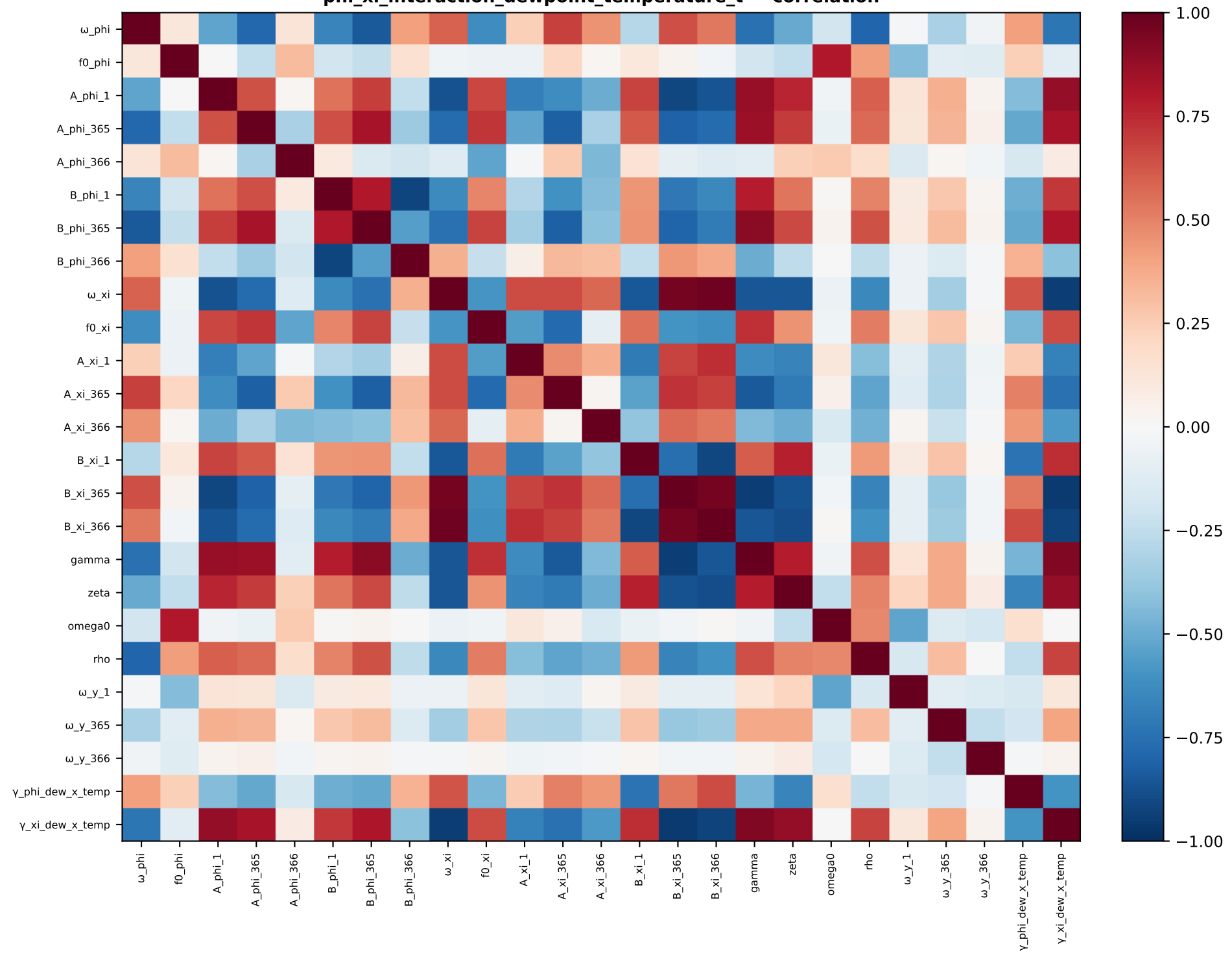
phi_xi_interaction_dewpoint_temperature_t — correlation
