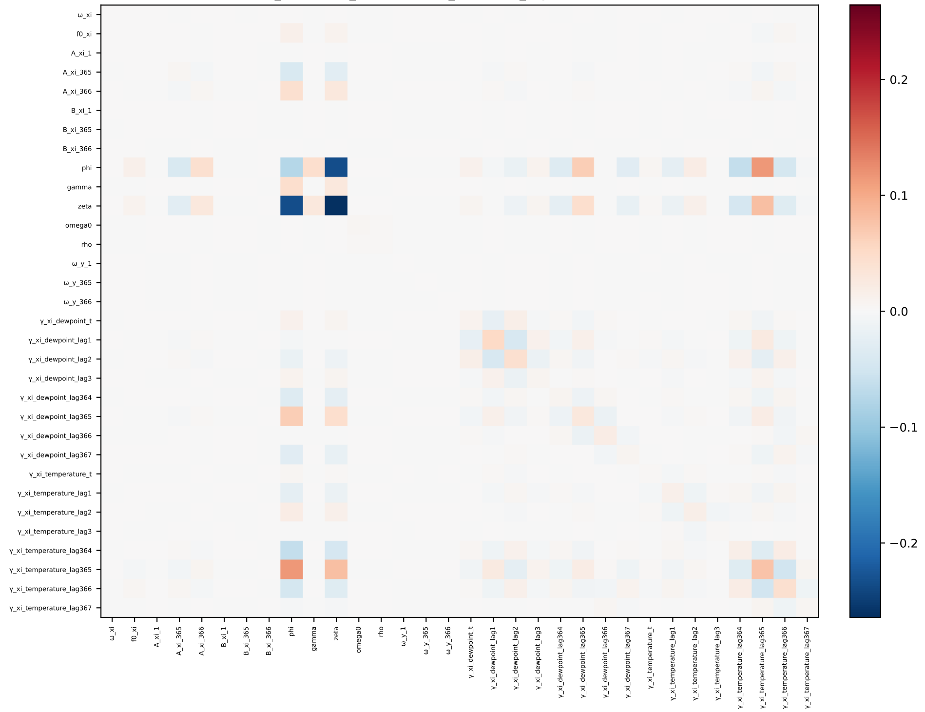
xi_dewpoint_temperature_seasonal_lags — covariance
