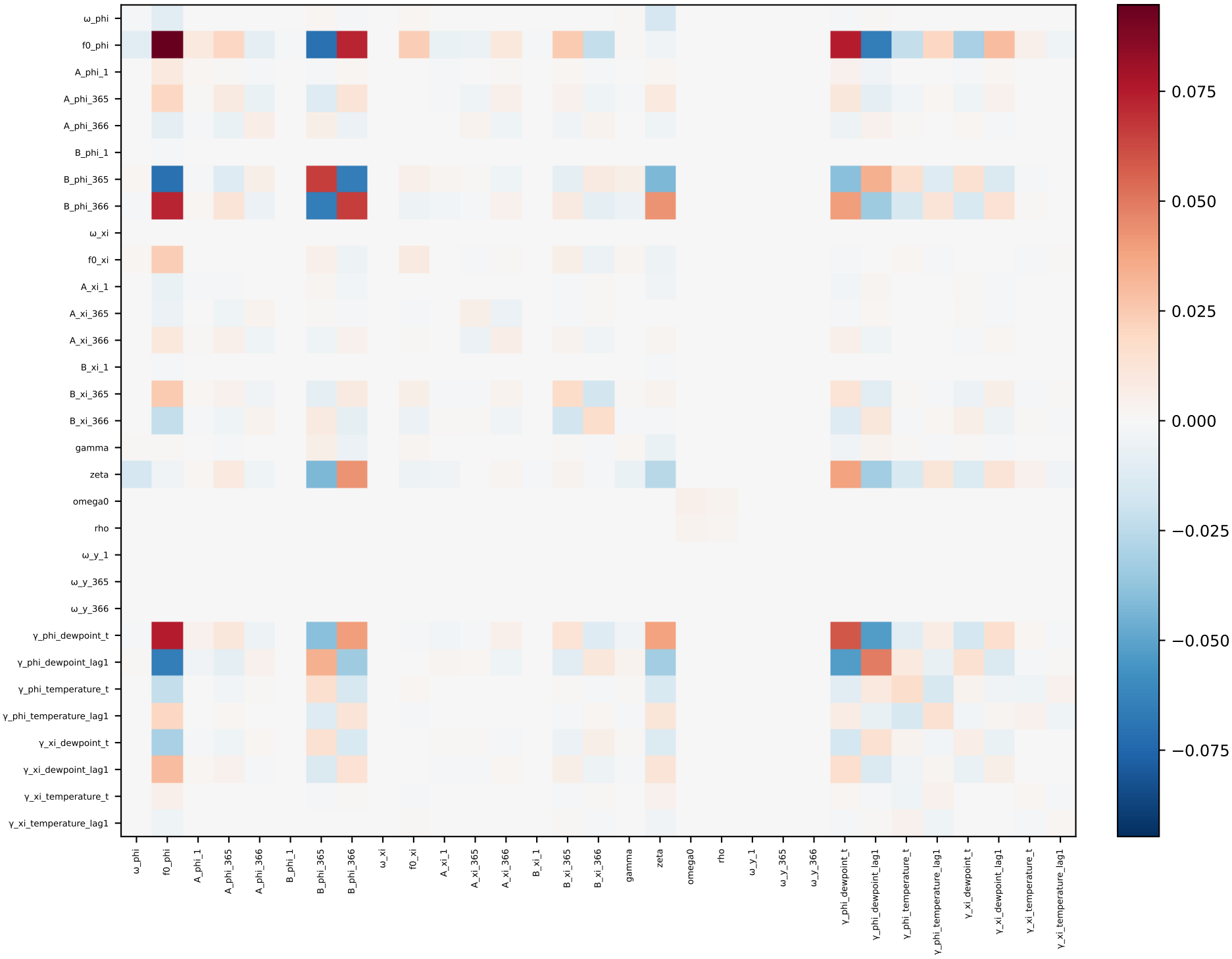
phi_xi_dewpoint_temperature_lag1 — covariance
