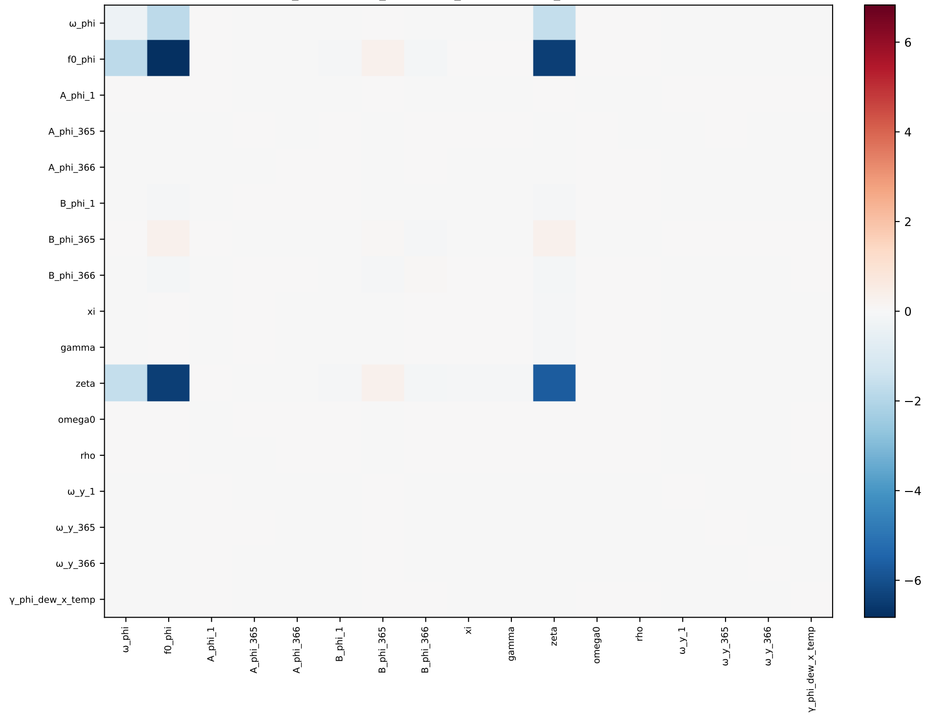
phi_interaction_dewpoint_temperature_t — covariance
