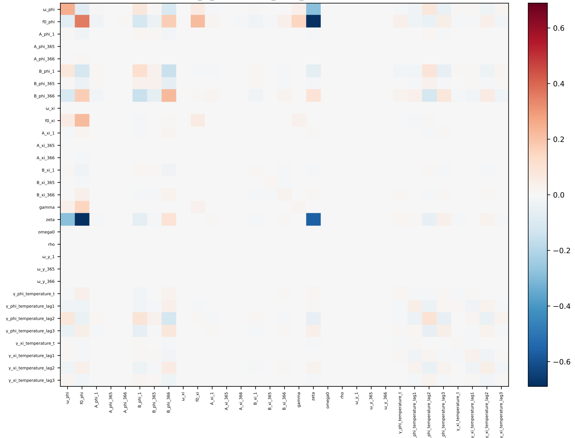
phi_xi_temperature_short_lags — covariance
