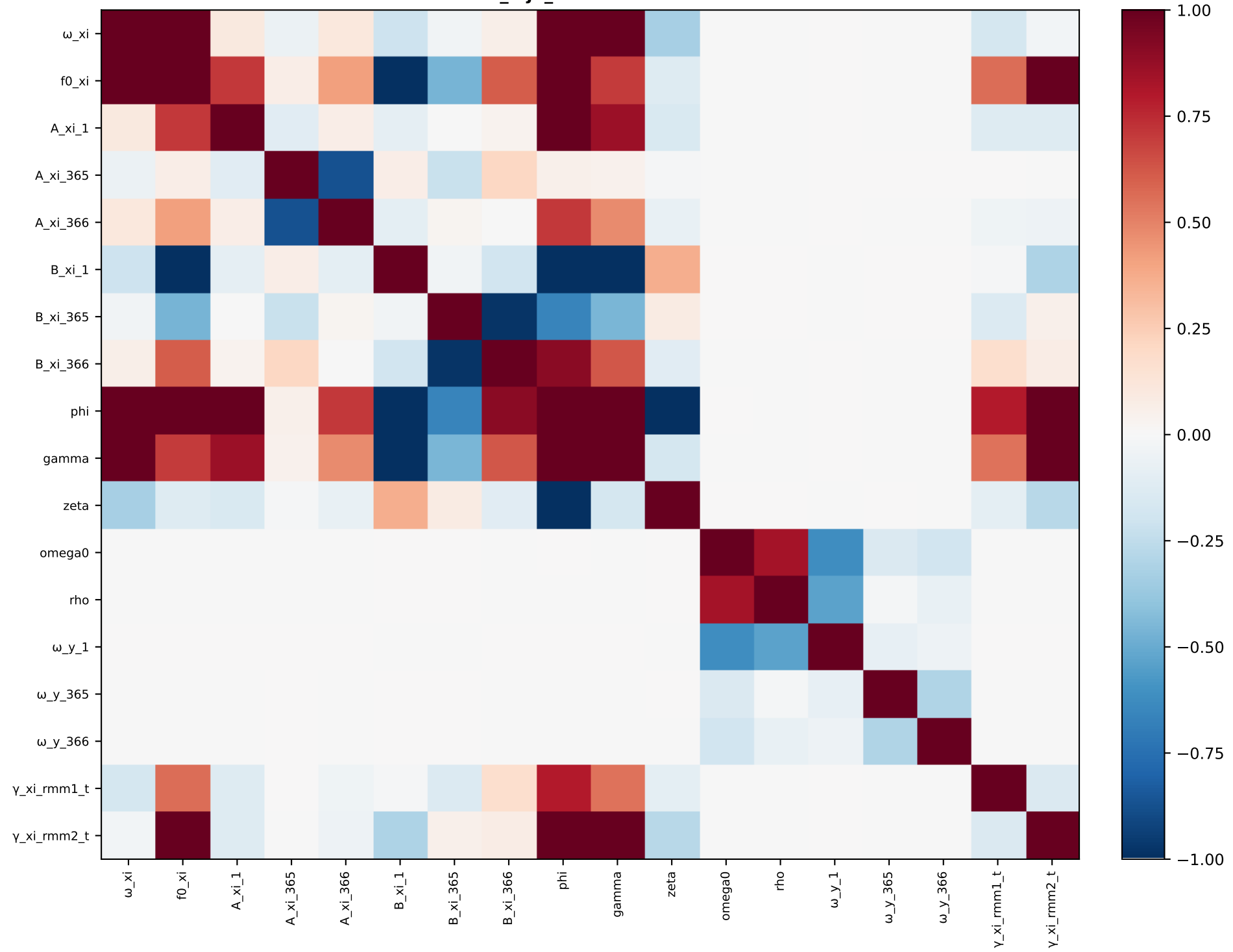
xi_mjo_t — correlation
