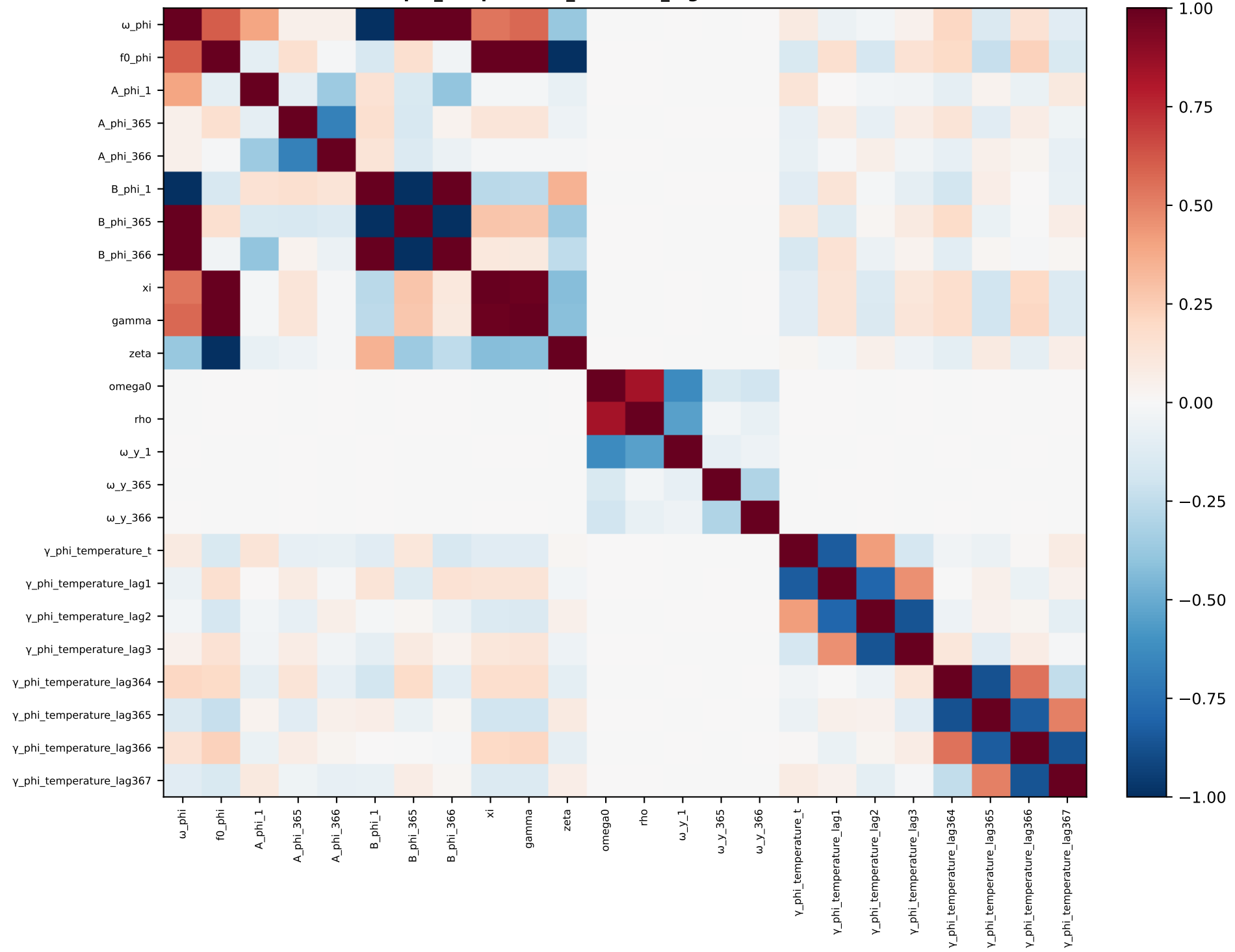
phi_temperature_seasonal_lags — correlation
