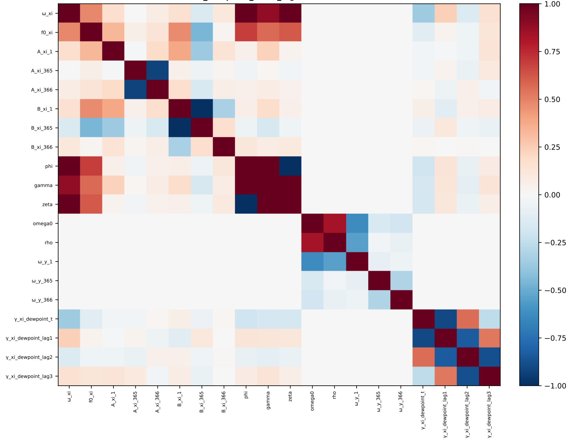
xi_dewpoint_short_lags — correlation
