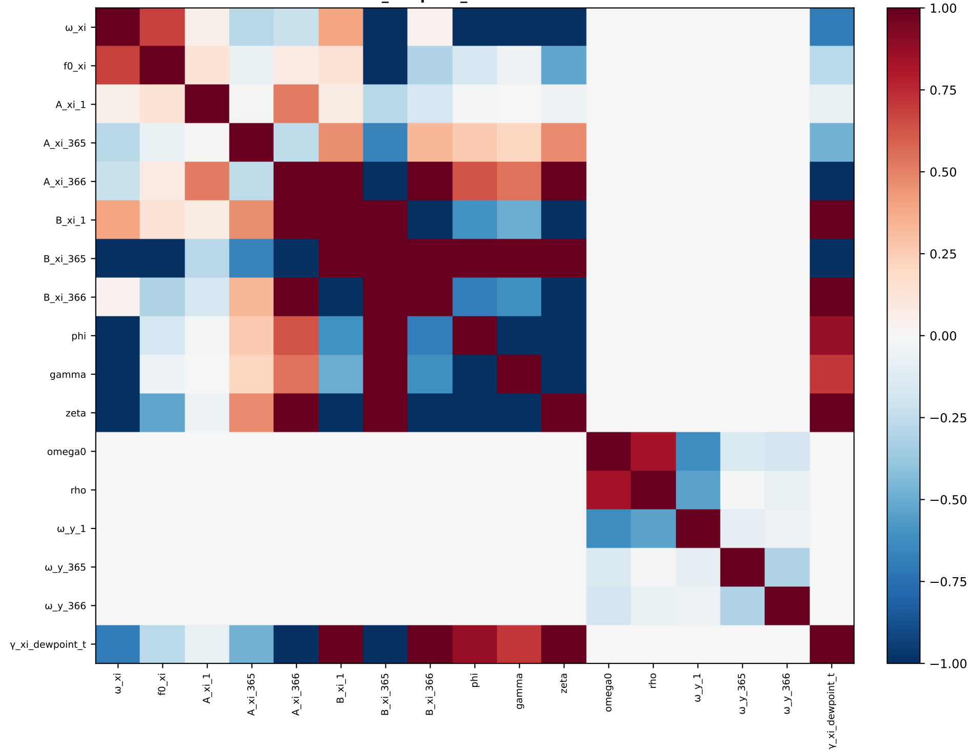
xi_dewpoint_t — correlation
