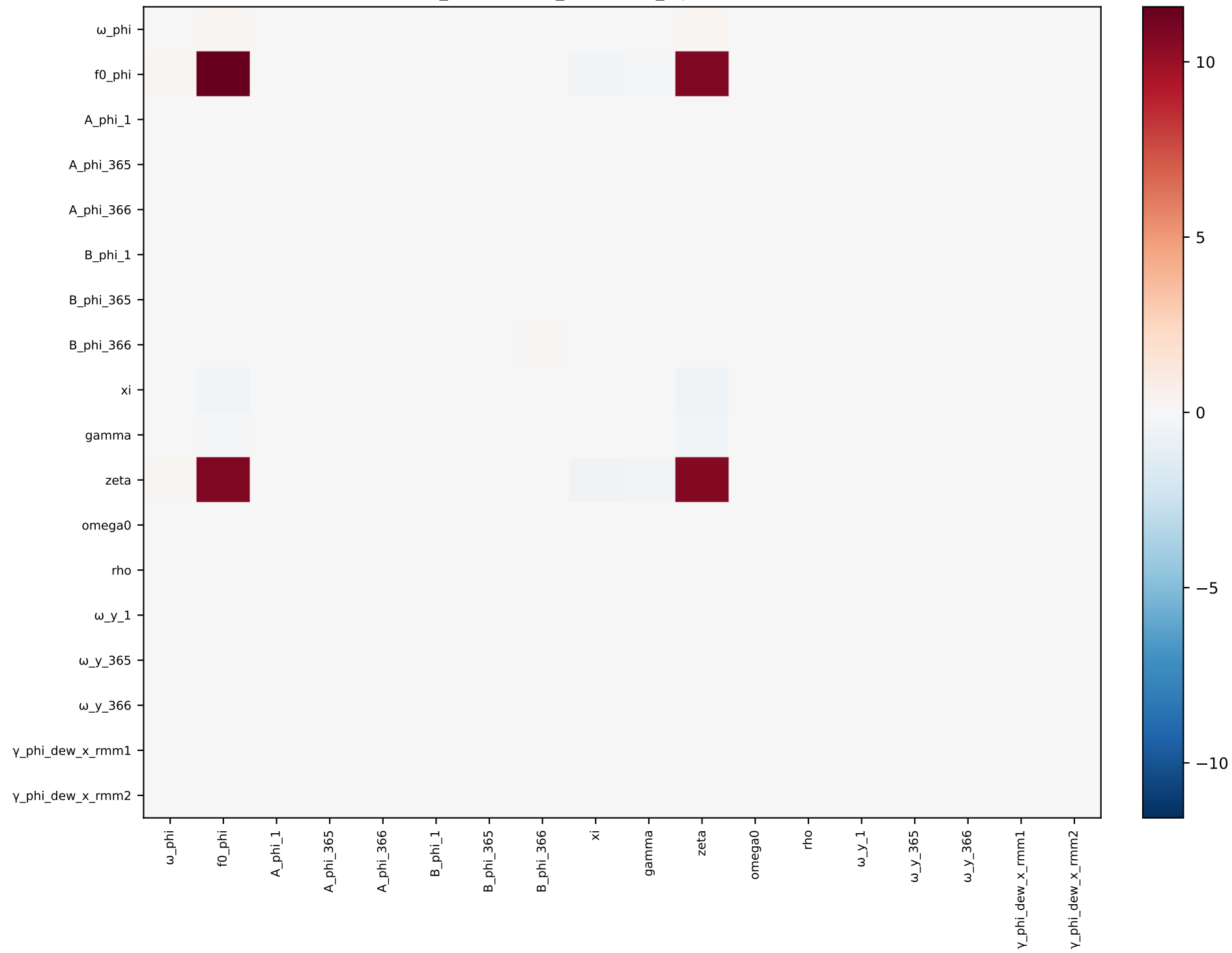
phi_interaction_dewpoint_mjo — covariance
