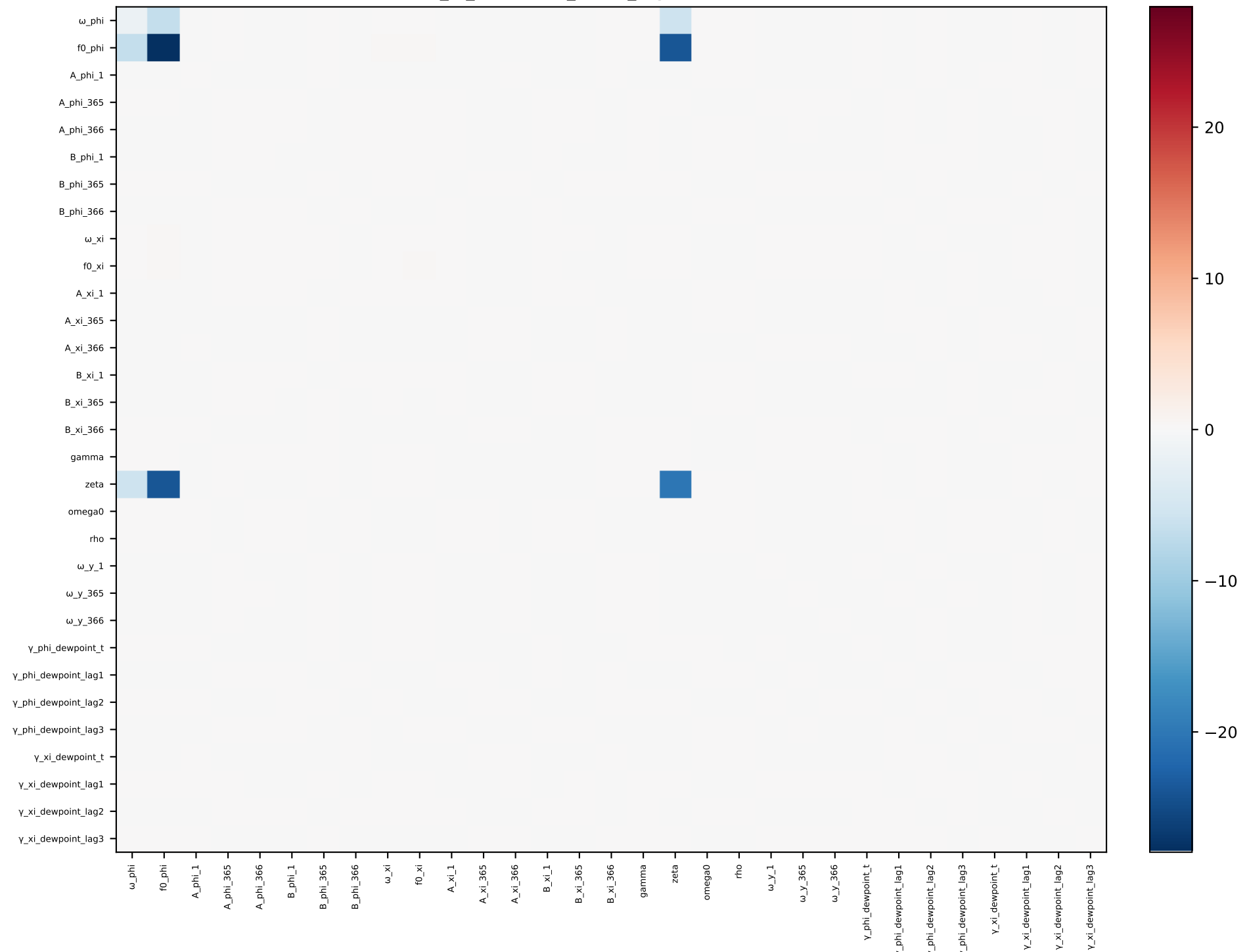
phi_xi_dewpoint_short_lags – covariance
