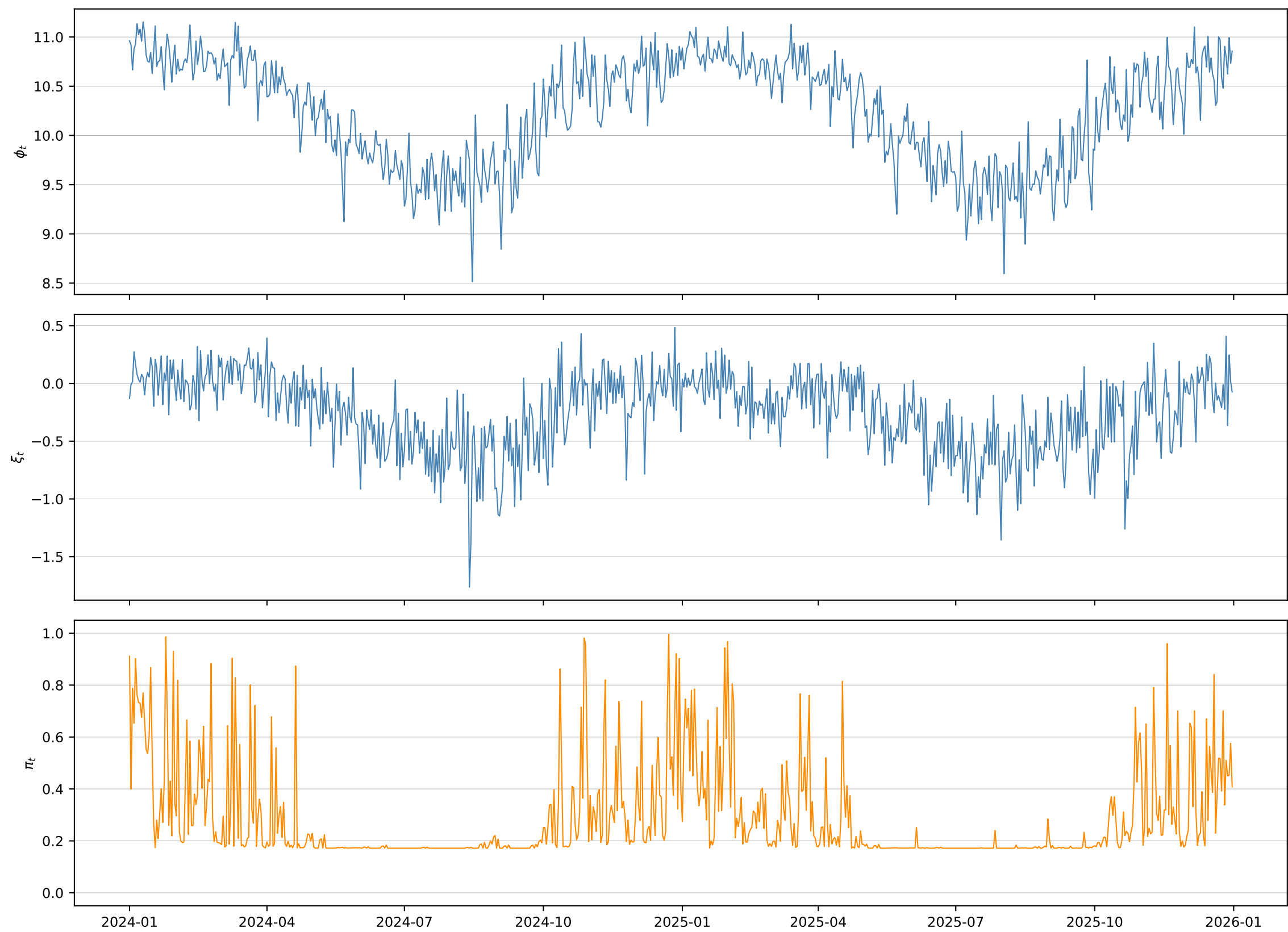
phi_xi_dewpoint_short_lags — filtered states (OOS)
