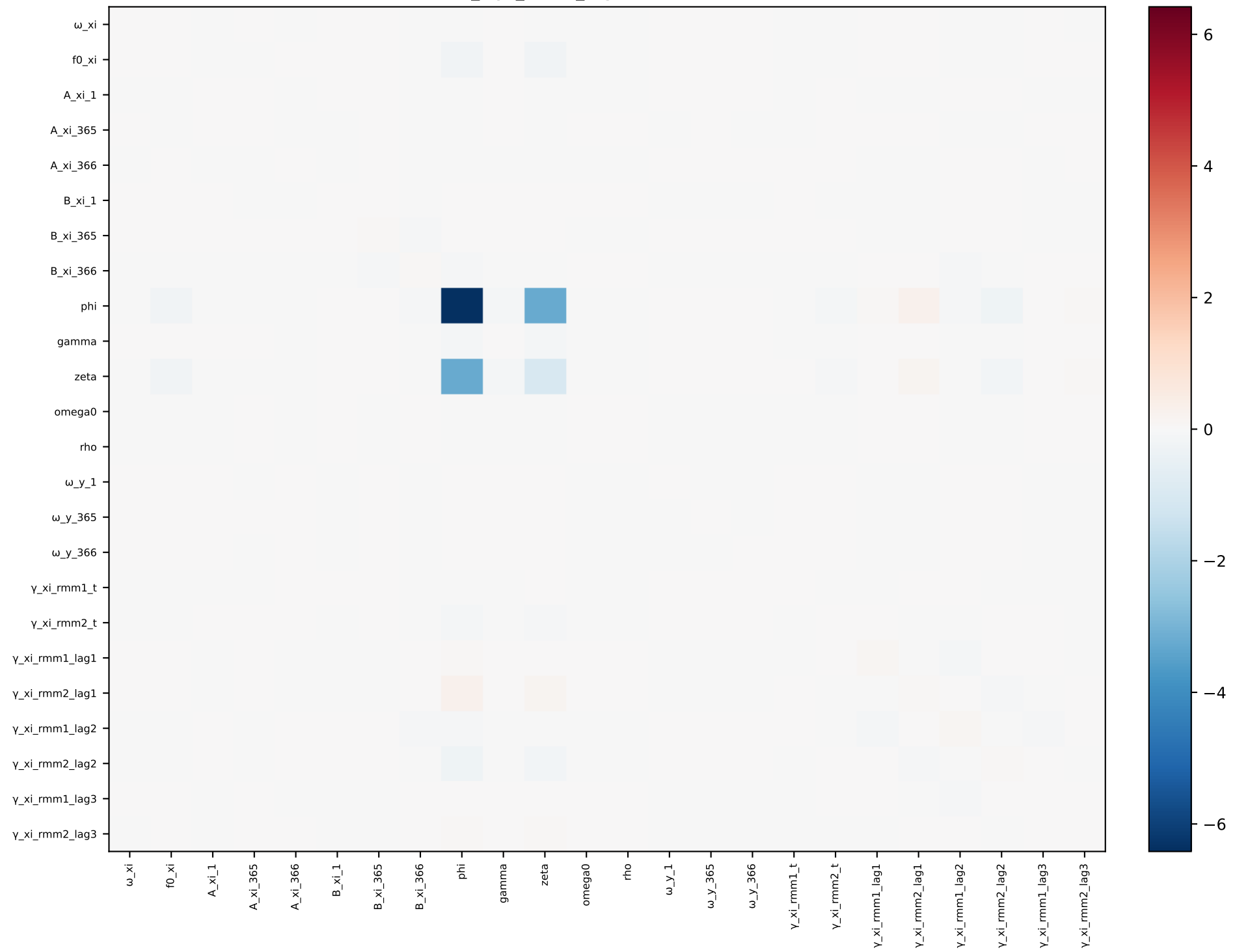
xi_mjo_short_lags — covariance
