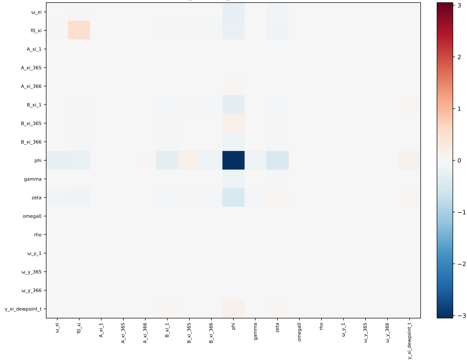
xi_dewpoint_t — covariance
