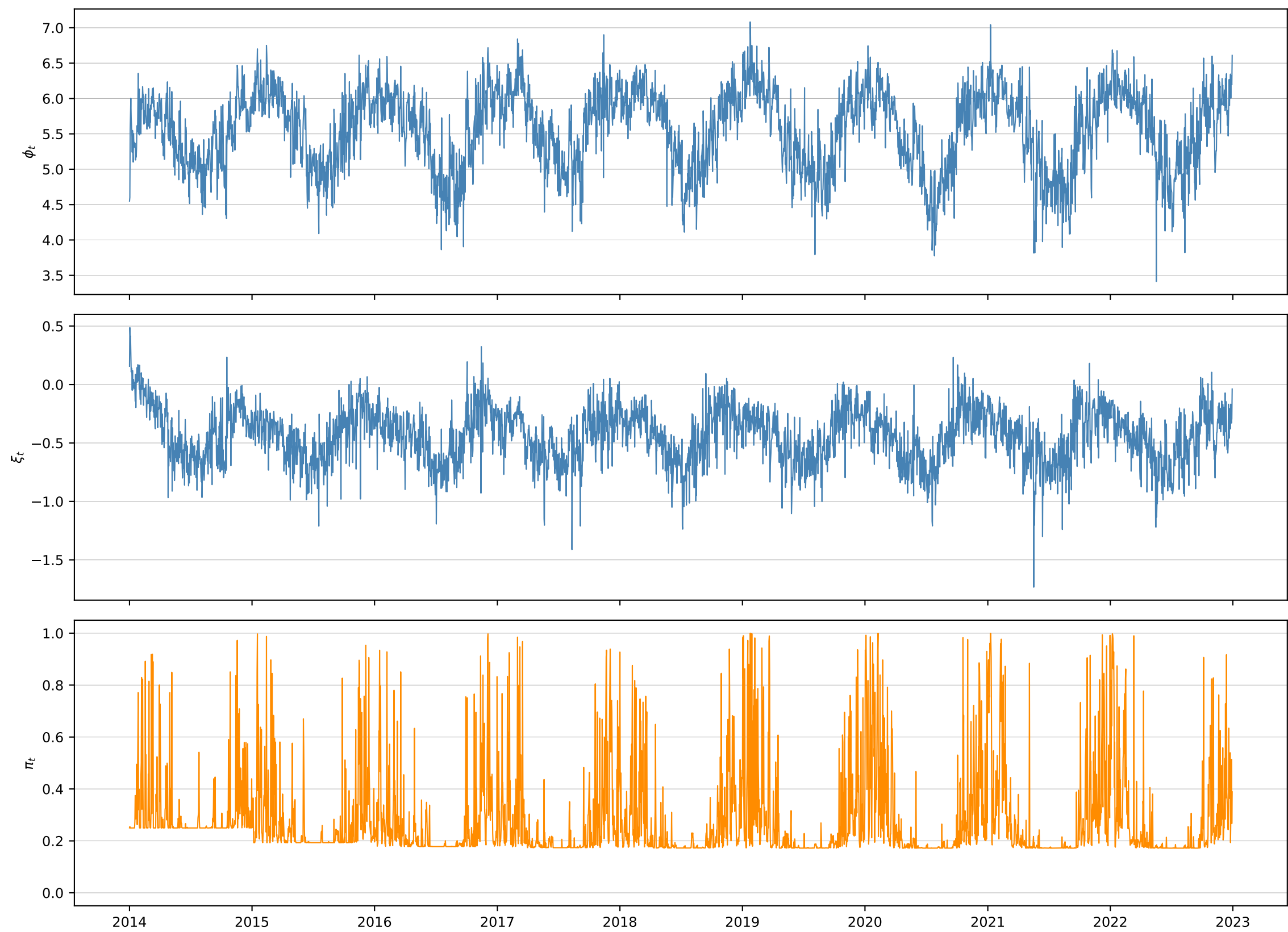
phi_xi_dewpoint_seasonal_lags — filtered states (IS)
