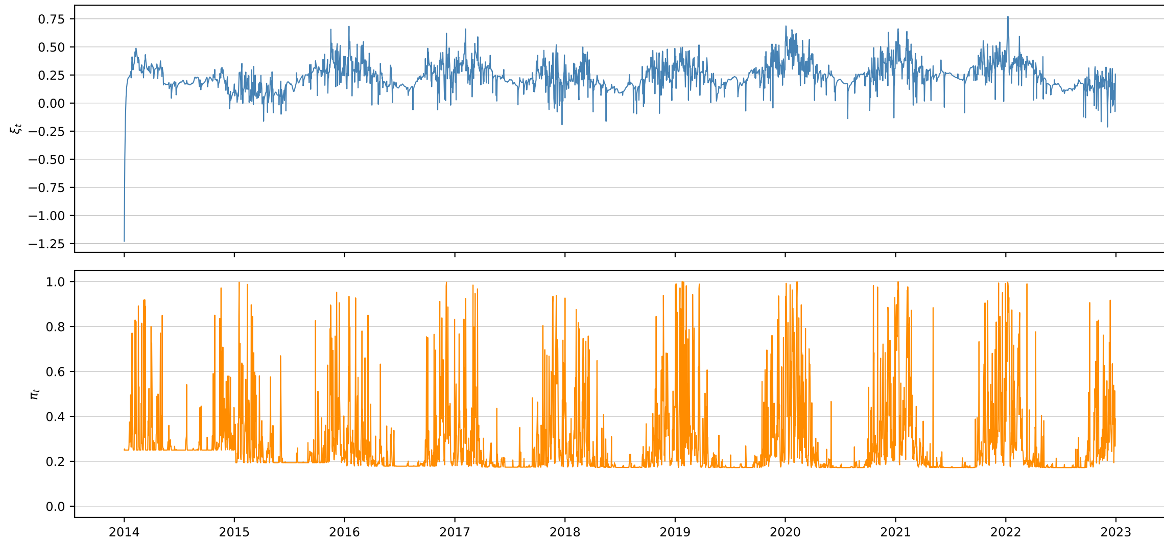
xi_nino34_lags — filtered states (IS)
