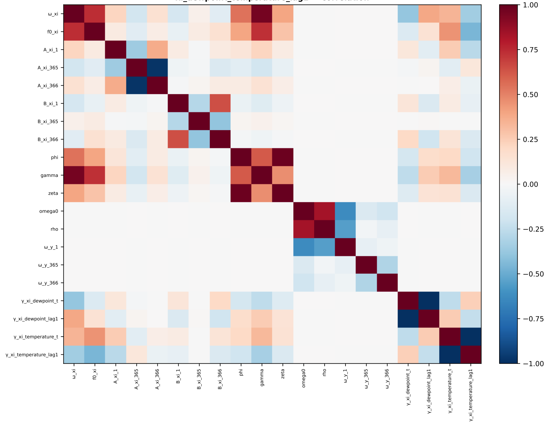
xi_dewpoint_temperature_lag1 — correlation
