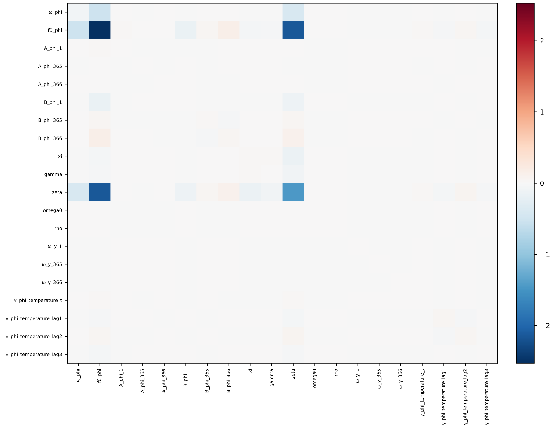
phi_temperature_short_lags — covariance
