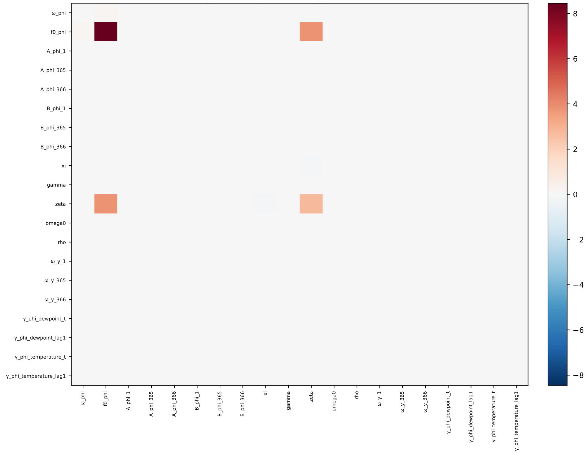
phi_dewpoint_temperature_lag1 — covariance
