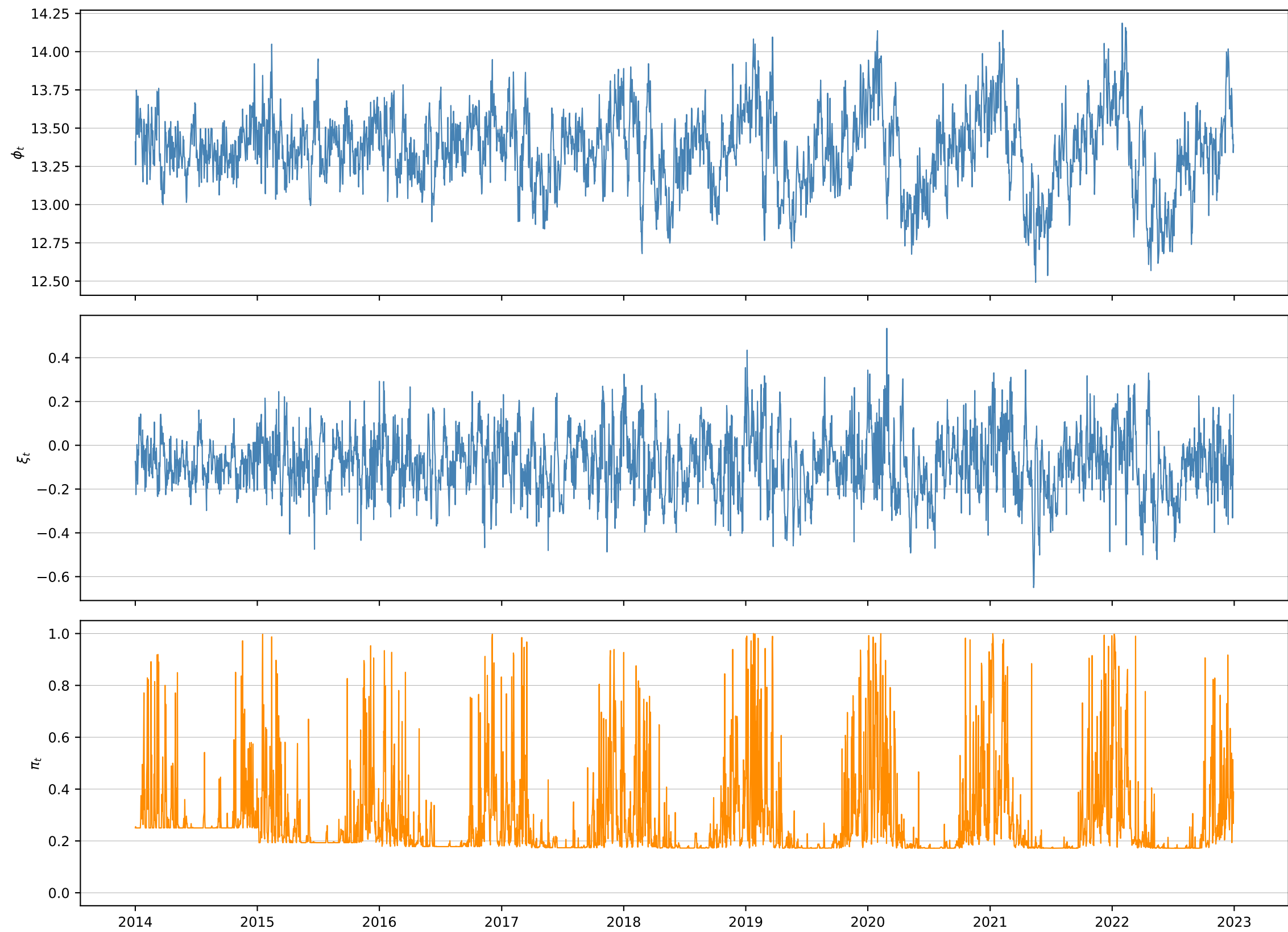
phi_xi_mjo_short_lags — filtered states (IS)
