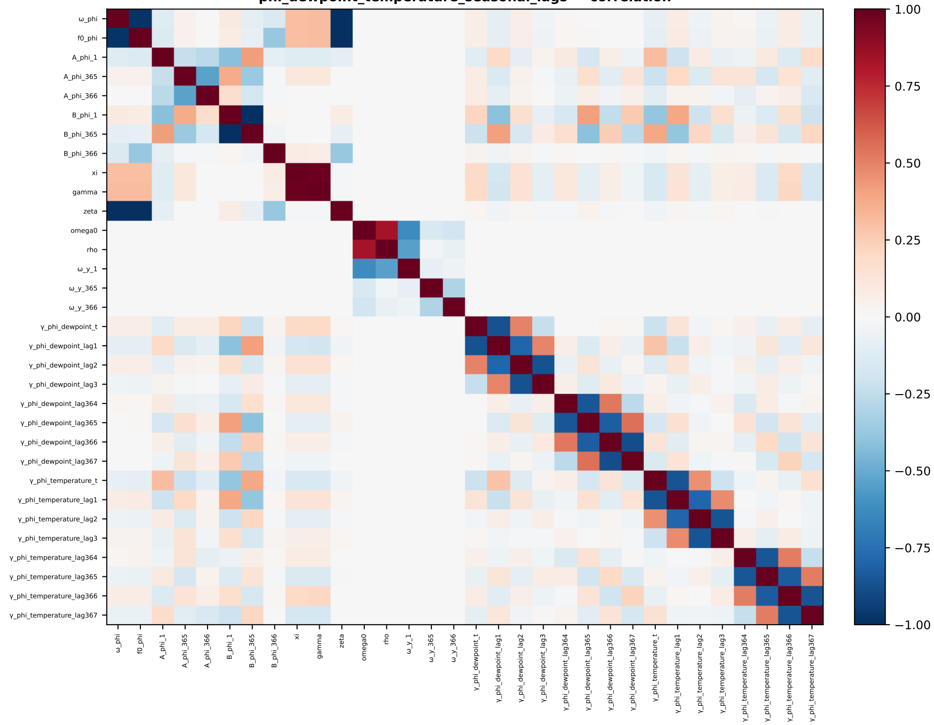
phi_dewpoint_temperature_seasonal_lags — correlation
