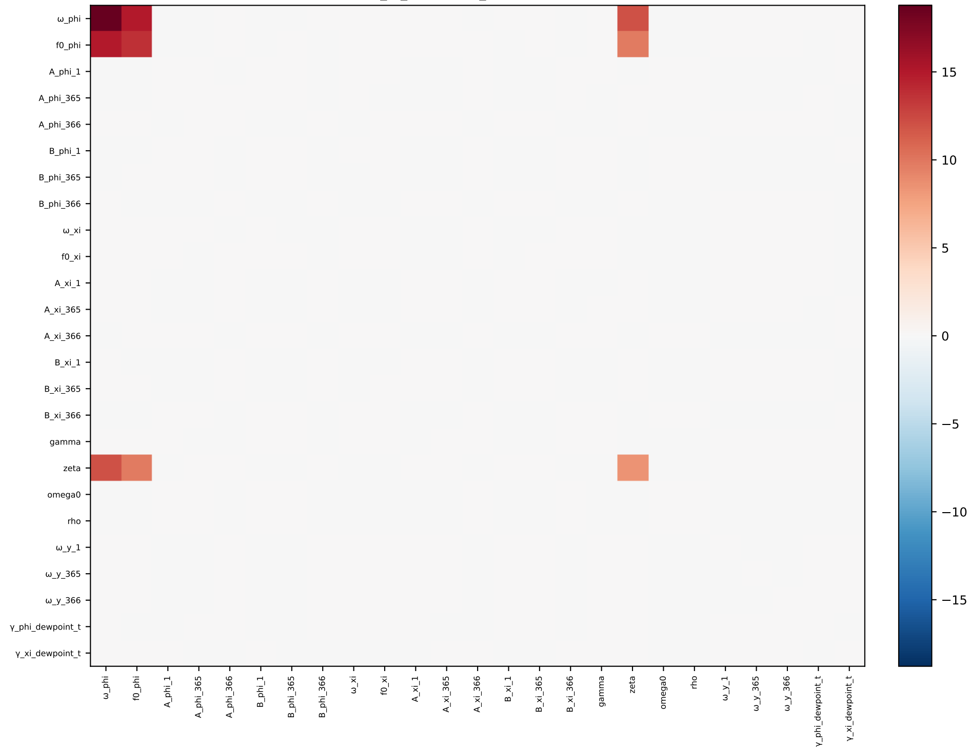
phi_xi_dewpoint_t — covariance
