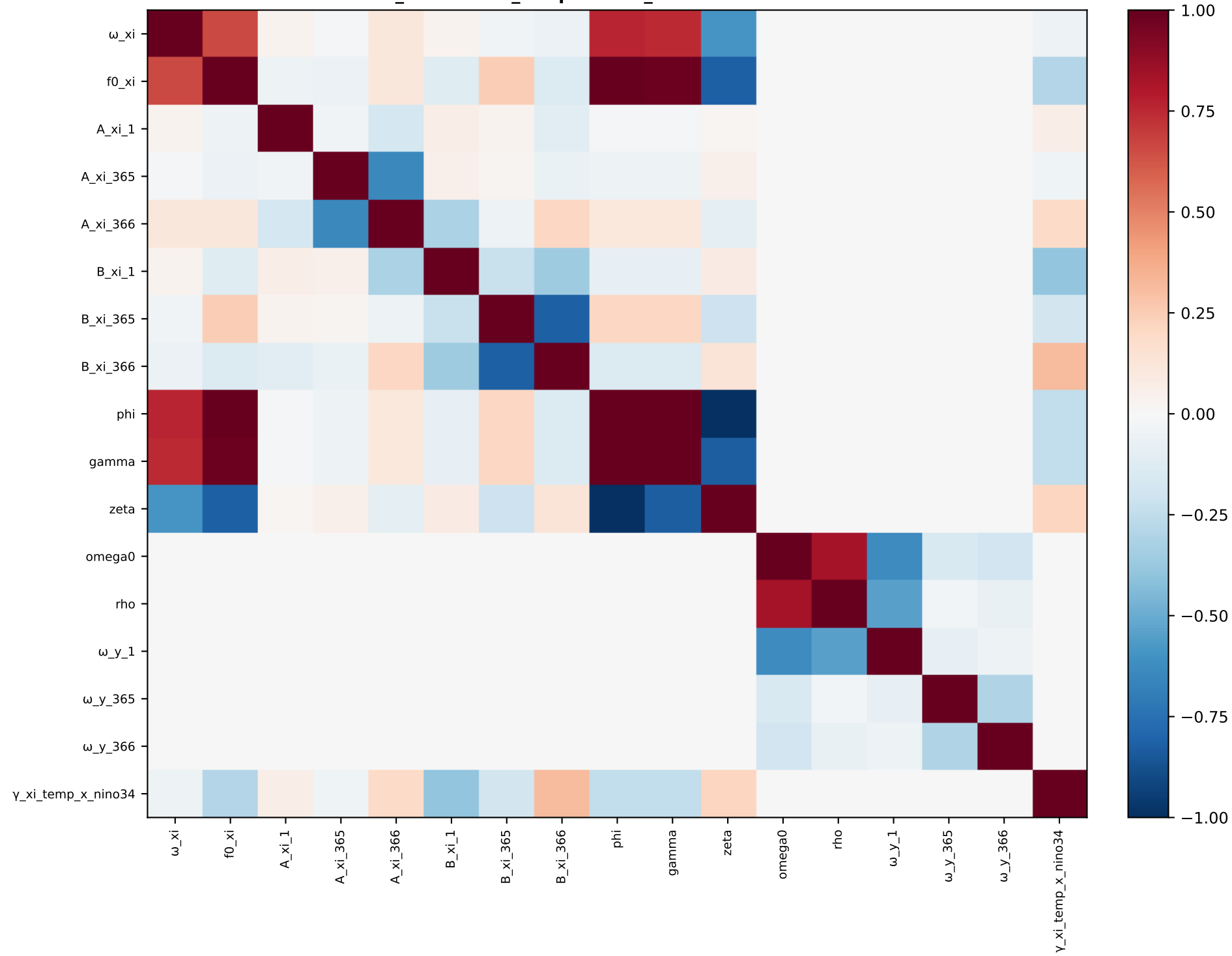
xi_interaction_temperature_nino34 — correlation
