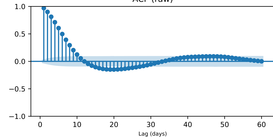
ACF (raw)
