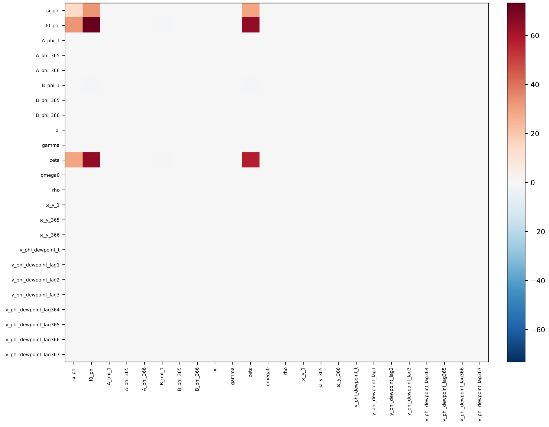
phi_dewpoint_seasonal_lags — covariance
