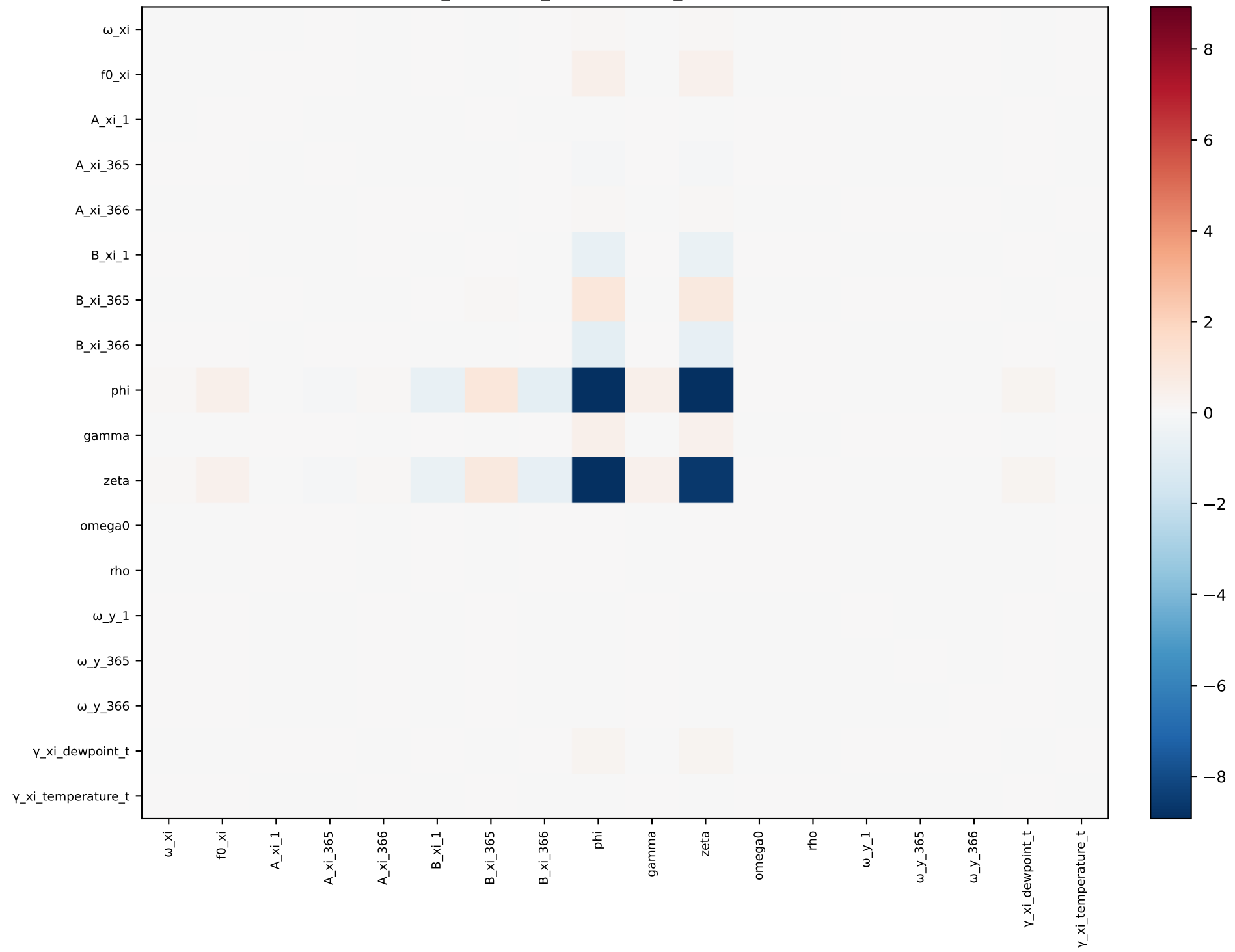
xi_dewpoint_temperature_t — covariance
