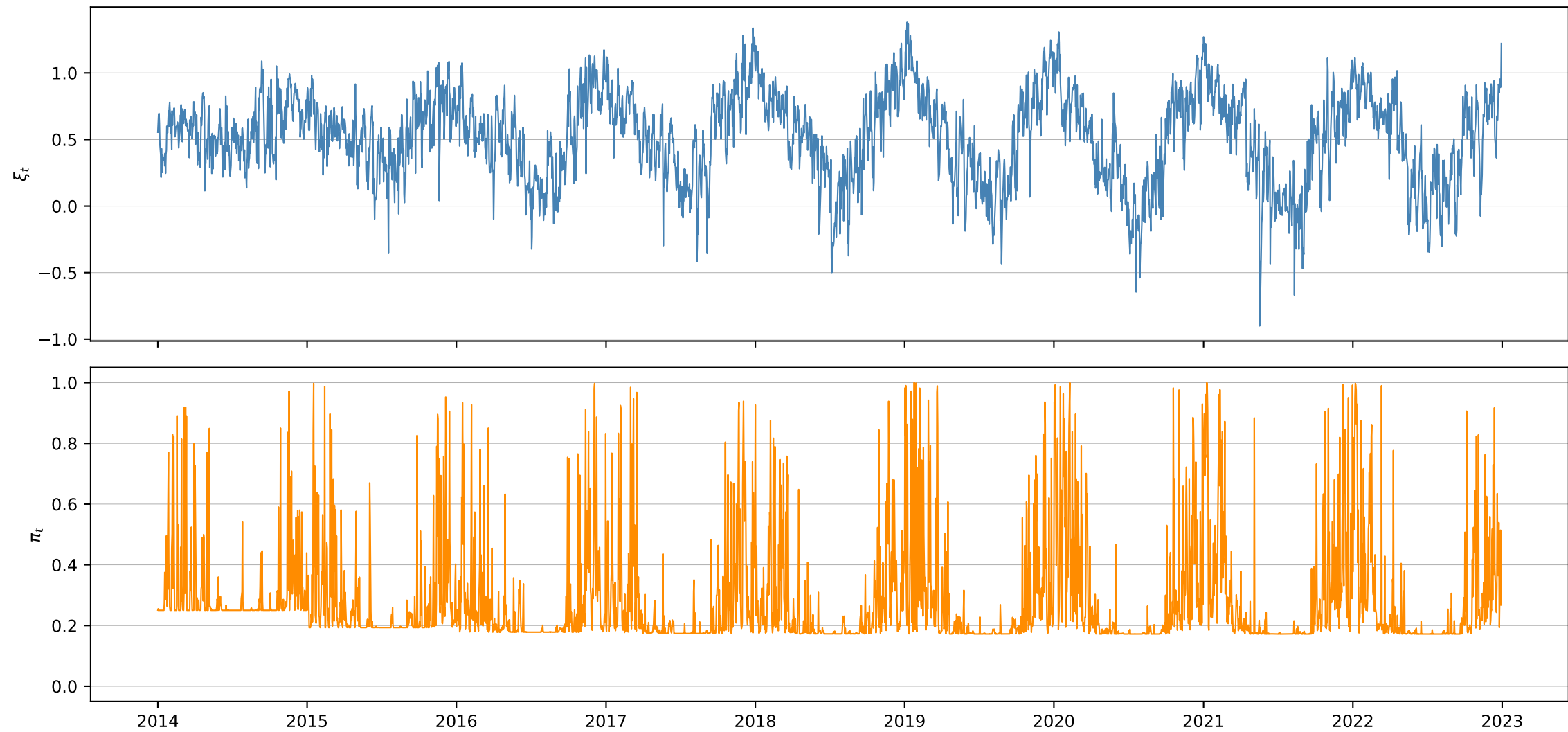
xi_dewpoint_seasonal_lags — filtered states (IS)
