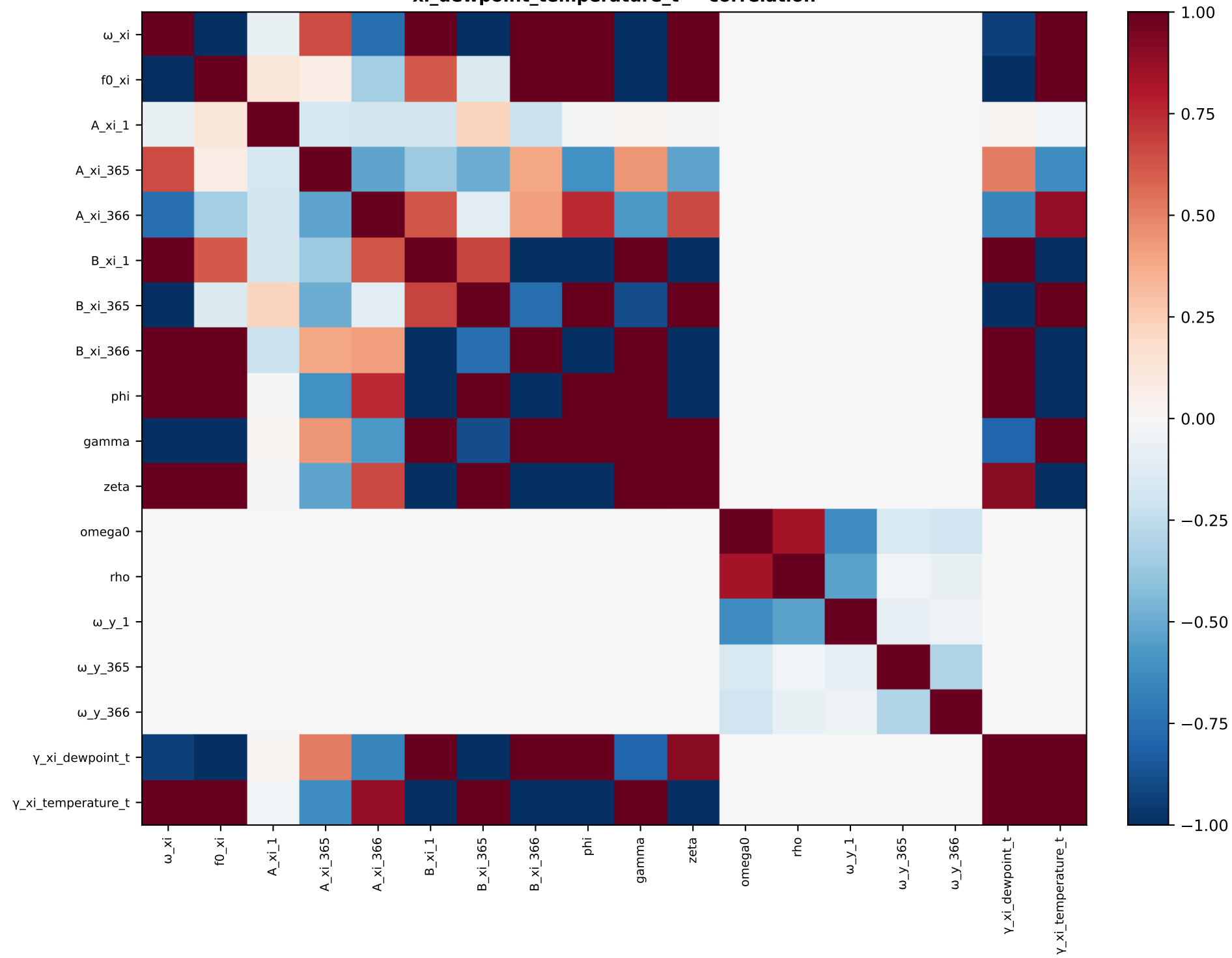
xi_dewpoint_temperature_t — correlation
