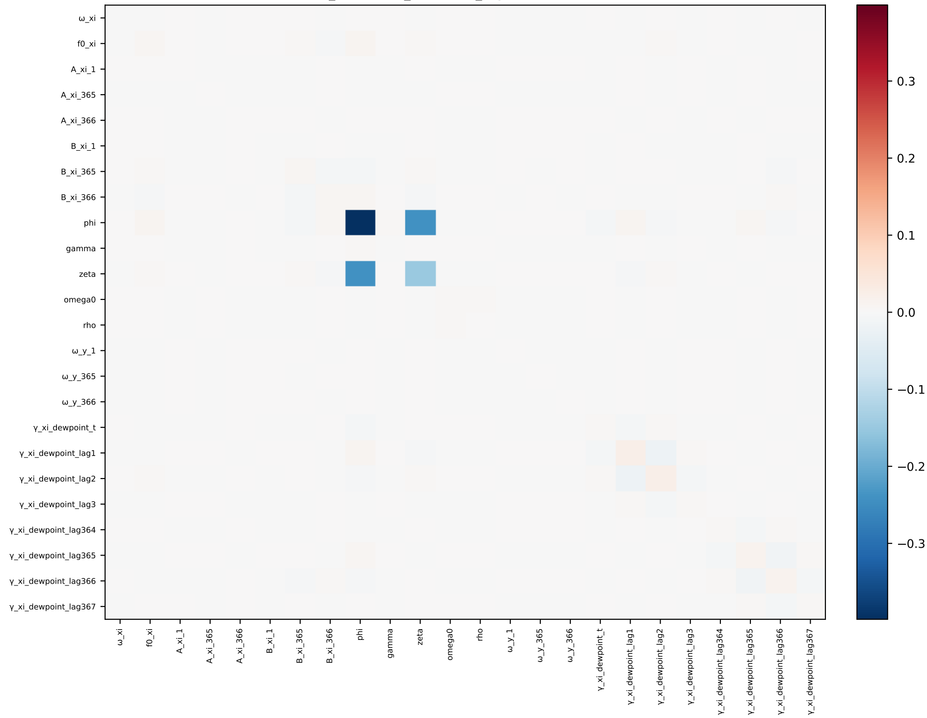
xi_dewpoint_seasonal_lags — covariance
