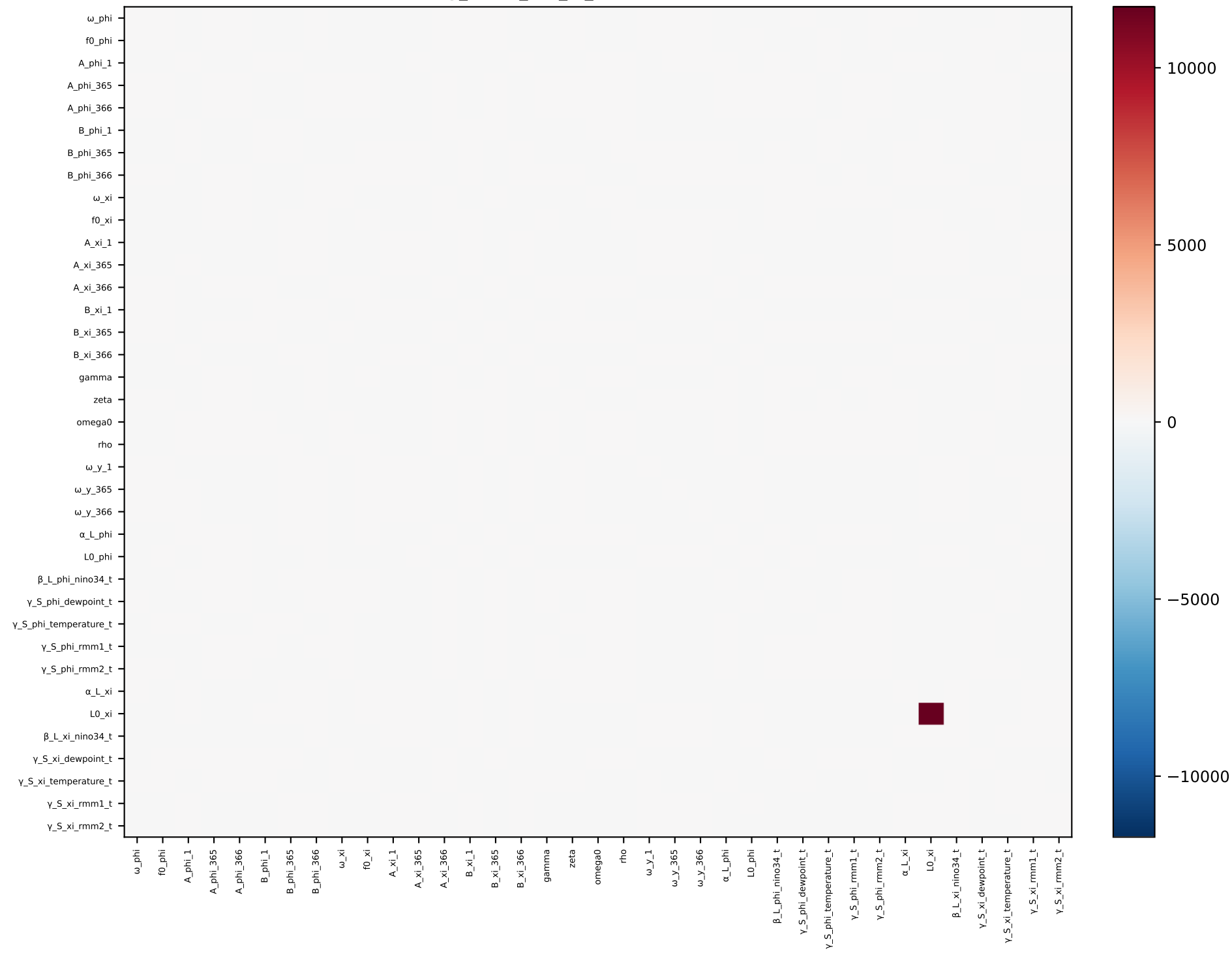
long_short_phi_xi_basic — covariance
