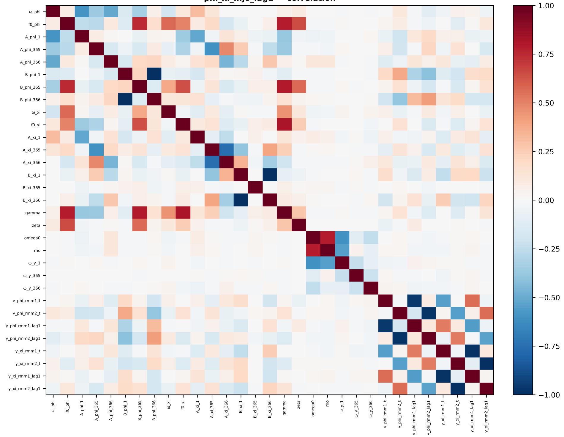
phi_xi_mjo_lag1 — correlation
