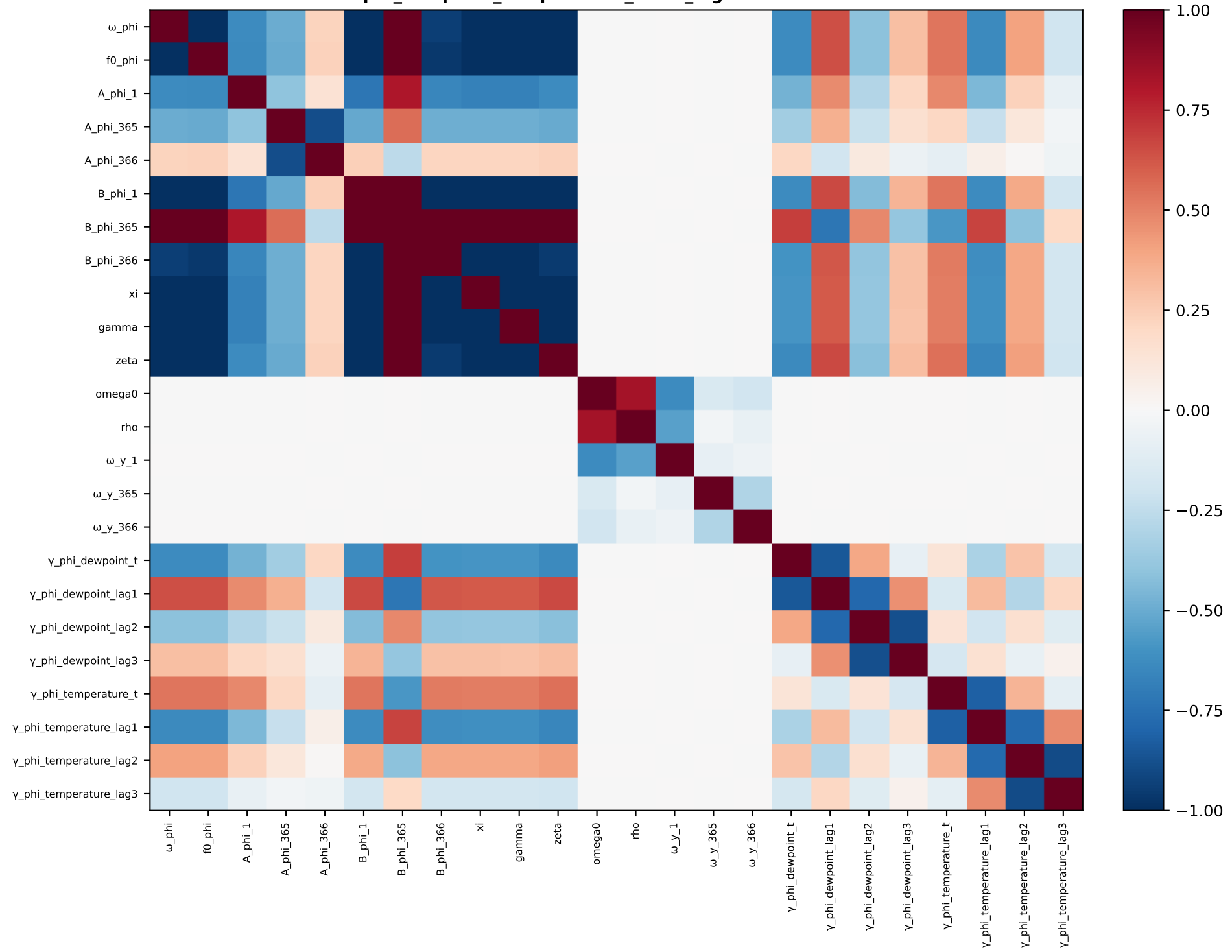
phi_dewpoint_temperature_short_lags — correlation
