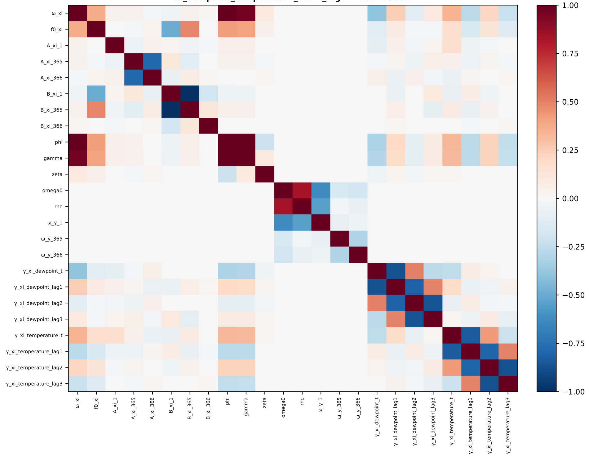
xi_dewpoint_temperature_short_lags — correlation
