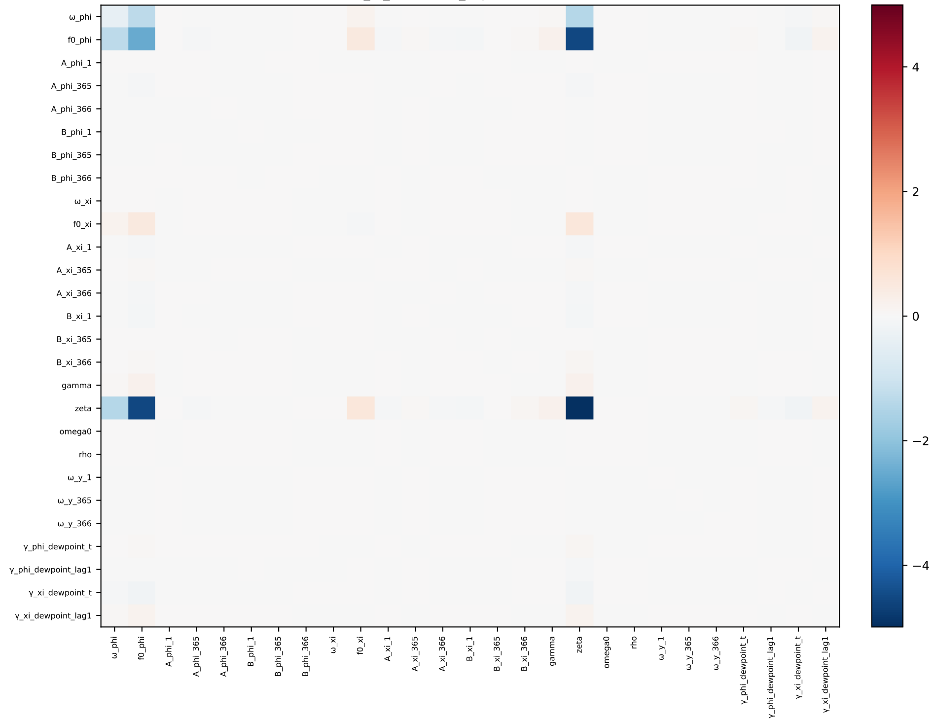
phi_xi_dewpoint_lag1 — covariance
