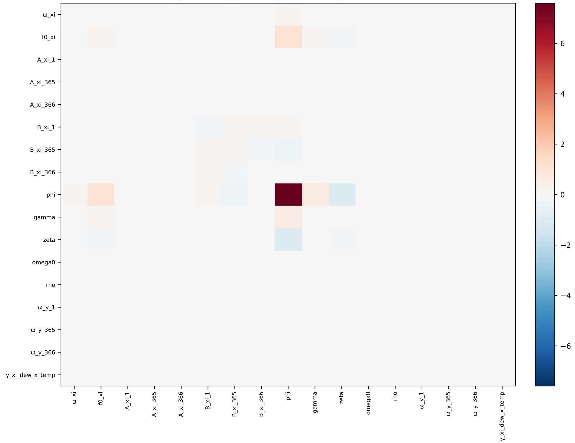
xi_interaction_dewpoint_temperature_t — covariance
