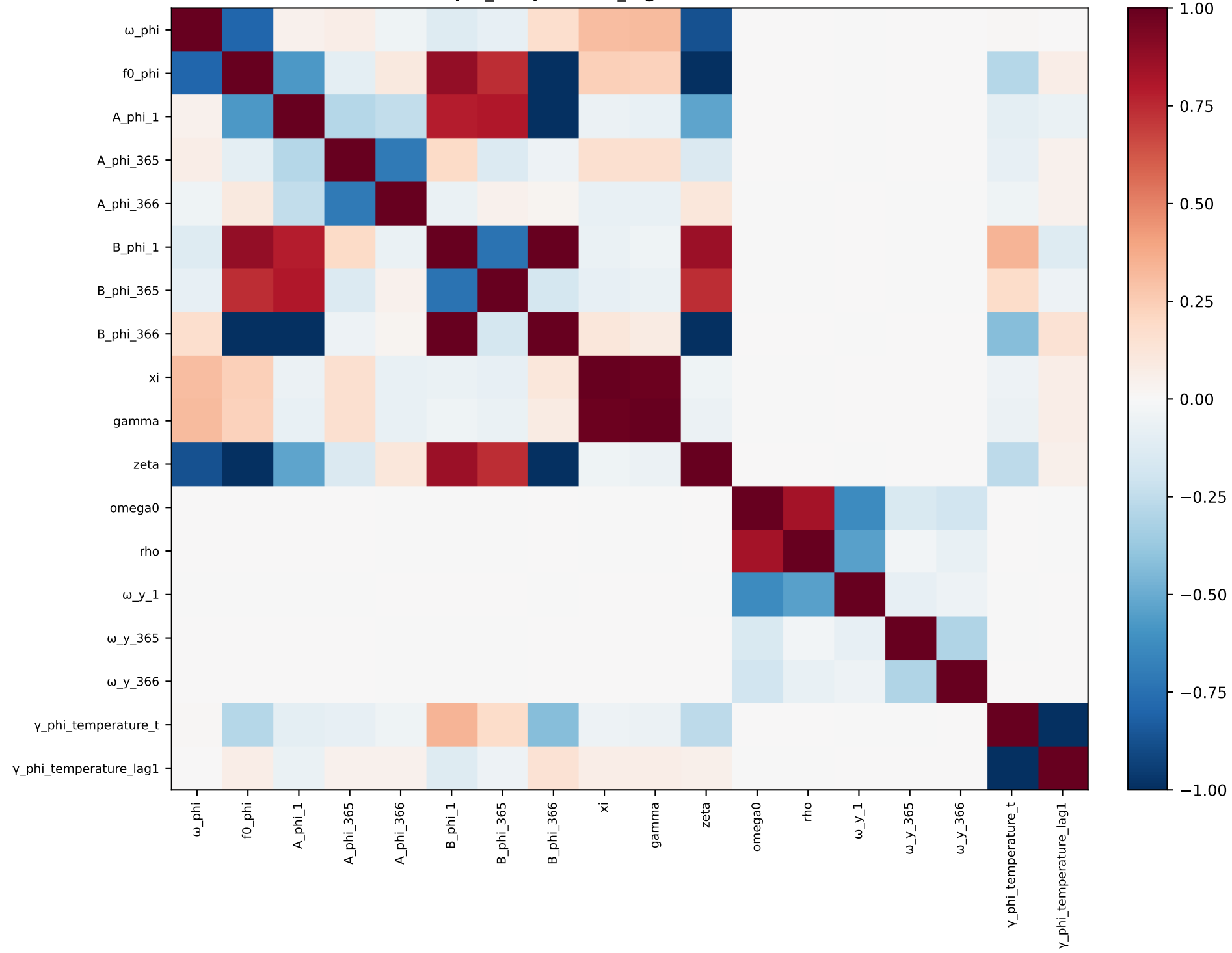
phi_temperature_lag1 — correlation
