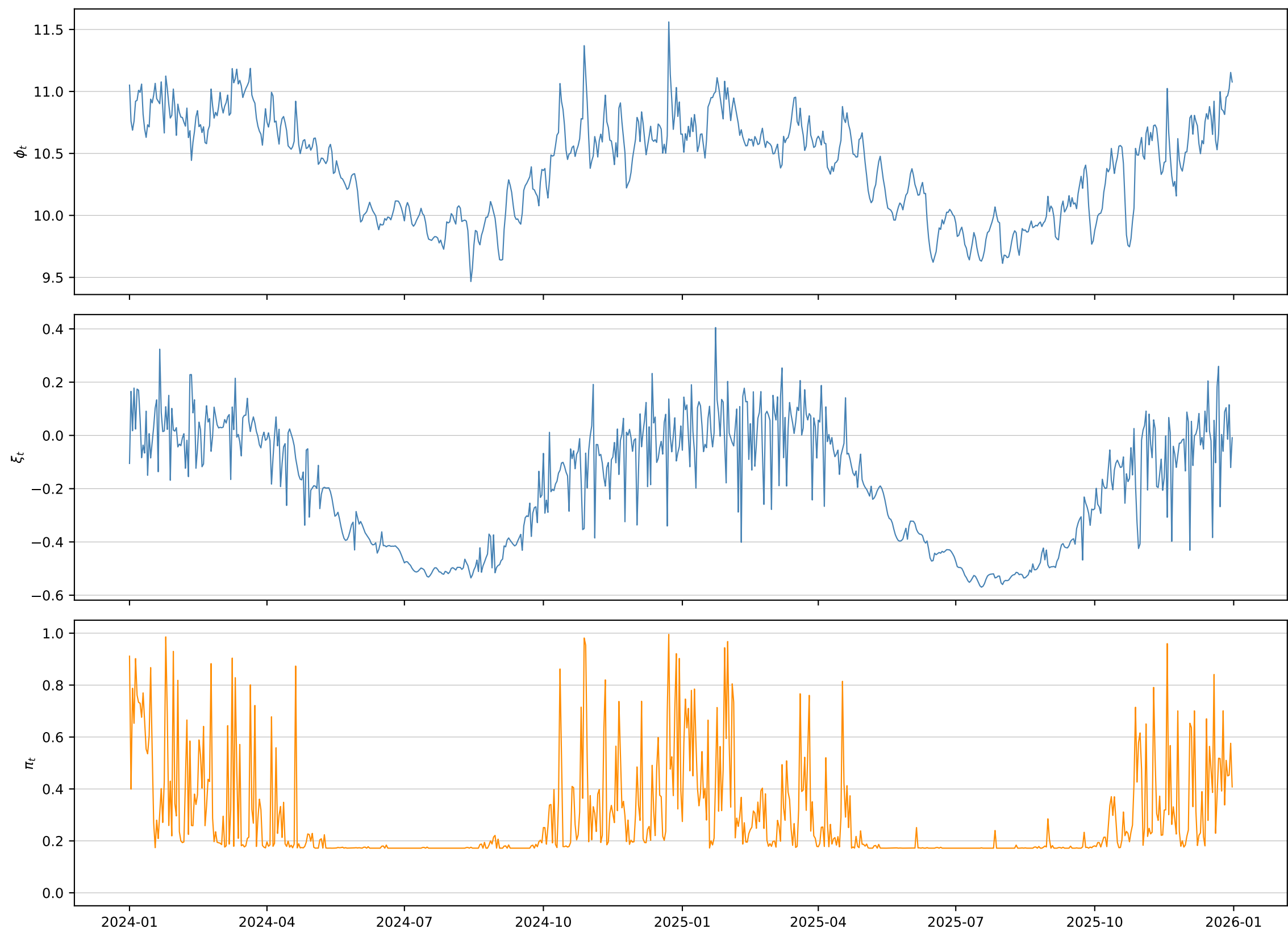
phi_xi_interaction_dewpoint_temperature_t — filtered states (OOS)
