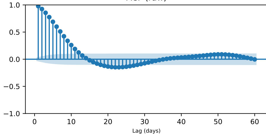
ACF (raw)
