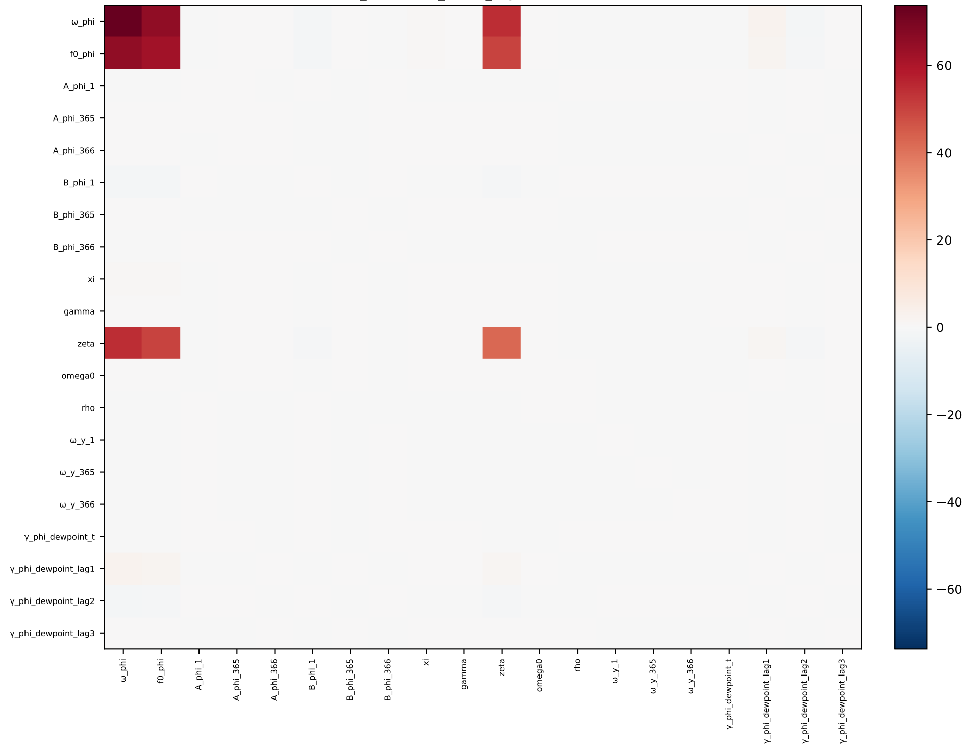
phi_dewpoint_short_lags — covariance
