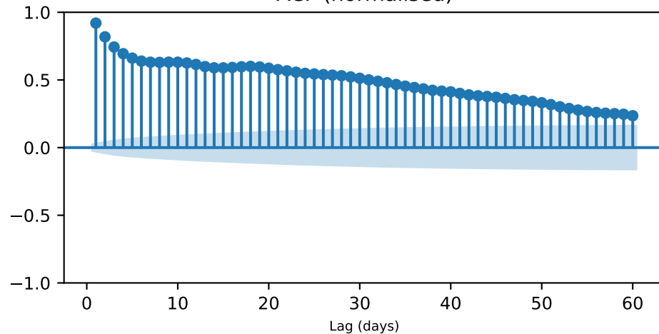
ACF (normalised)
