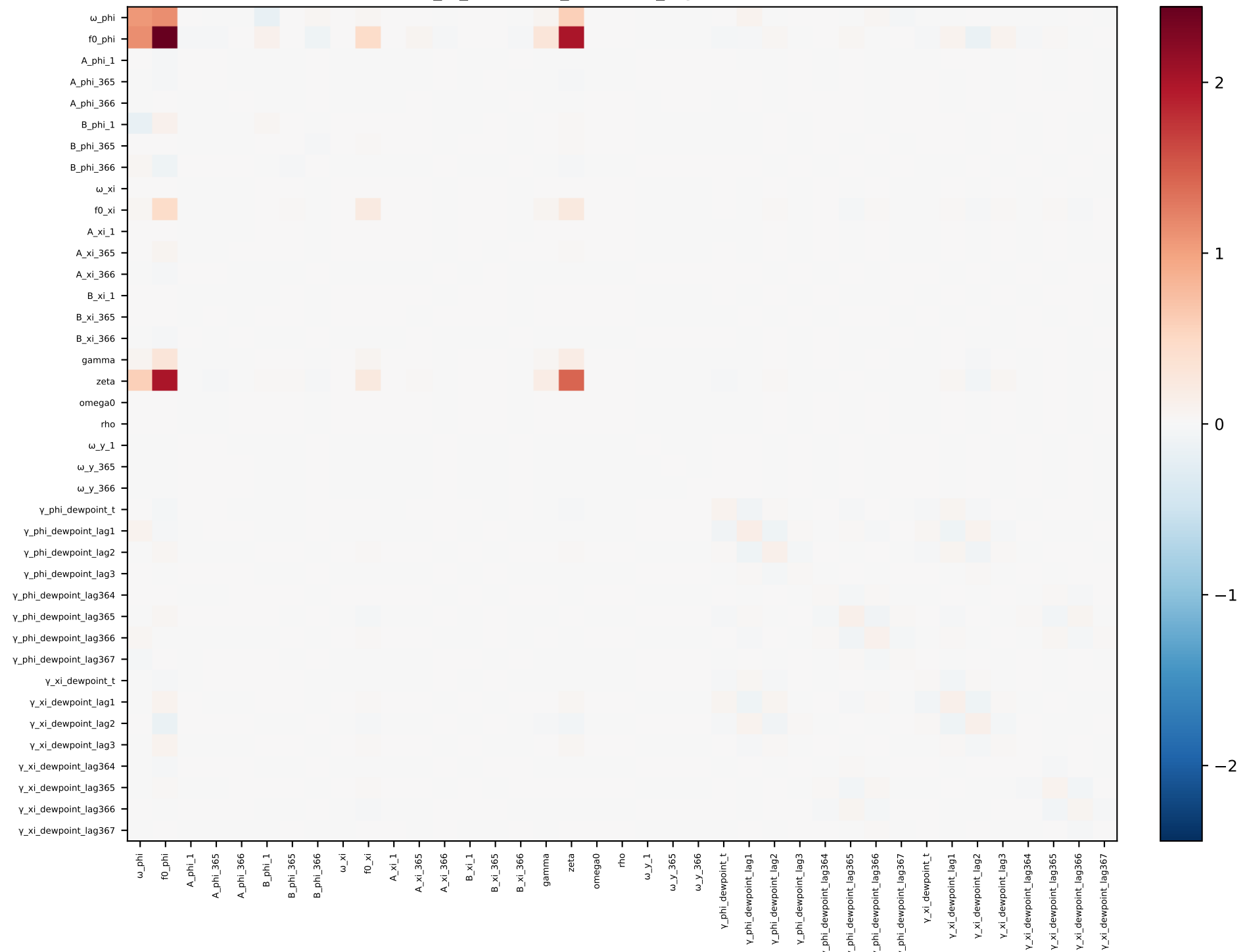
phi_xi_dewpoint_seasonal_lags — covariance
