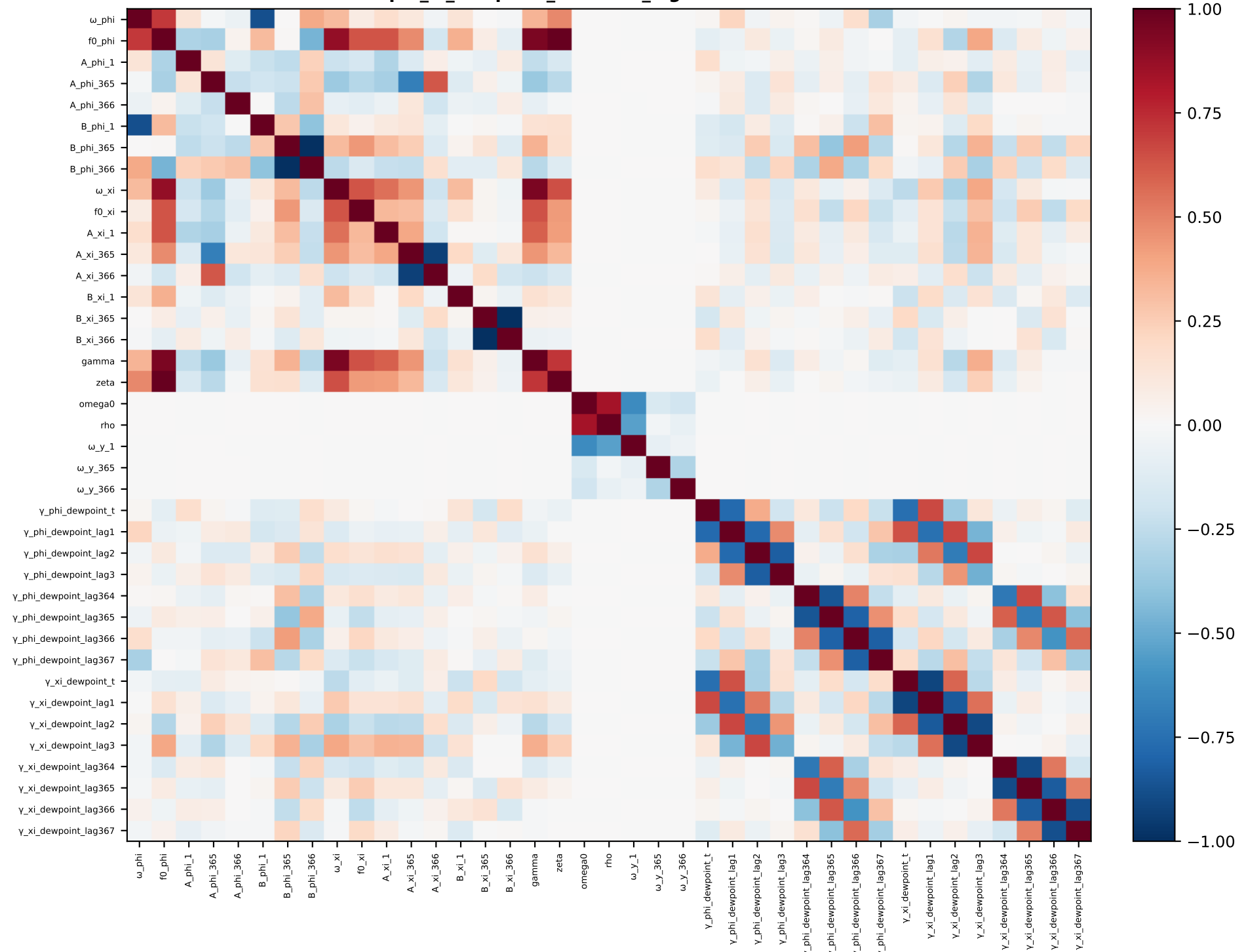
phi_xi_dewpoint_seasonal_lags — correlation
