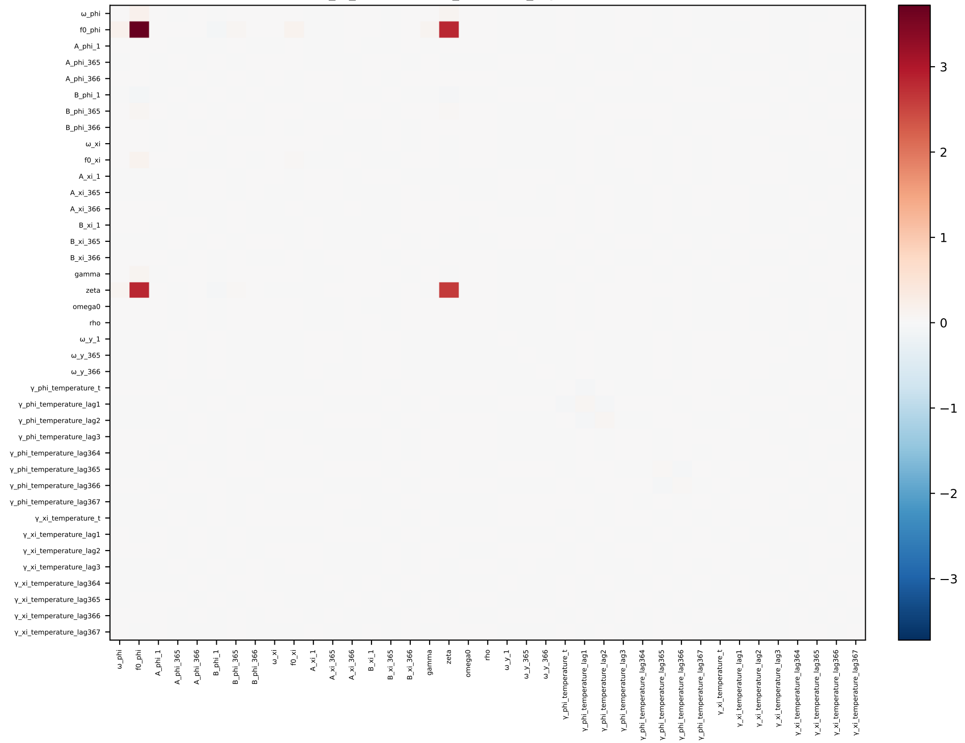
phi_xi_temperature_seasonal_lags — covariance
