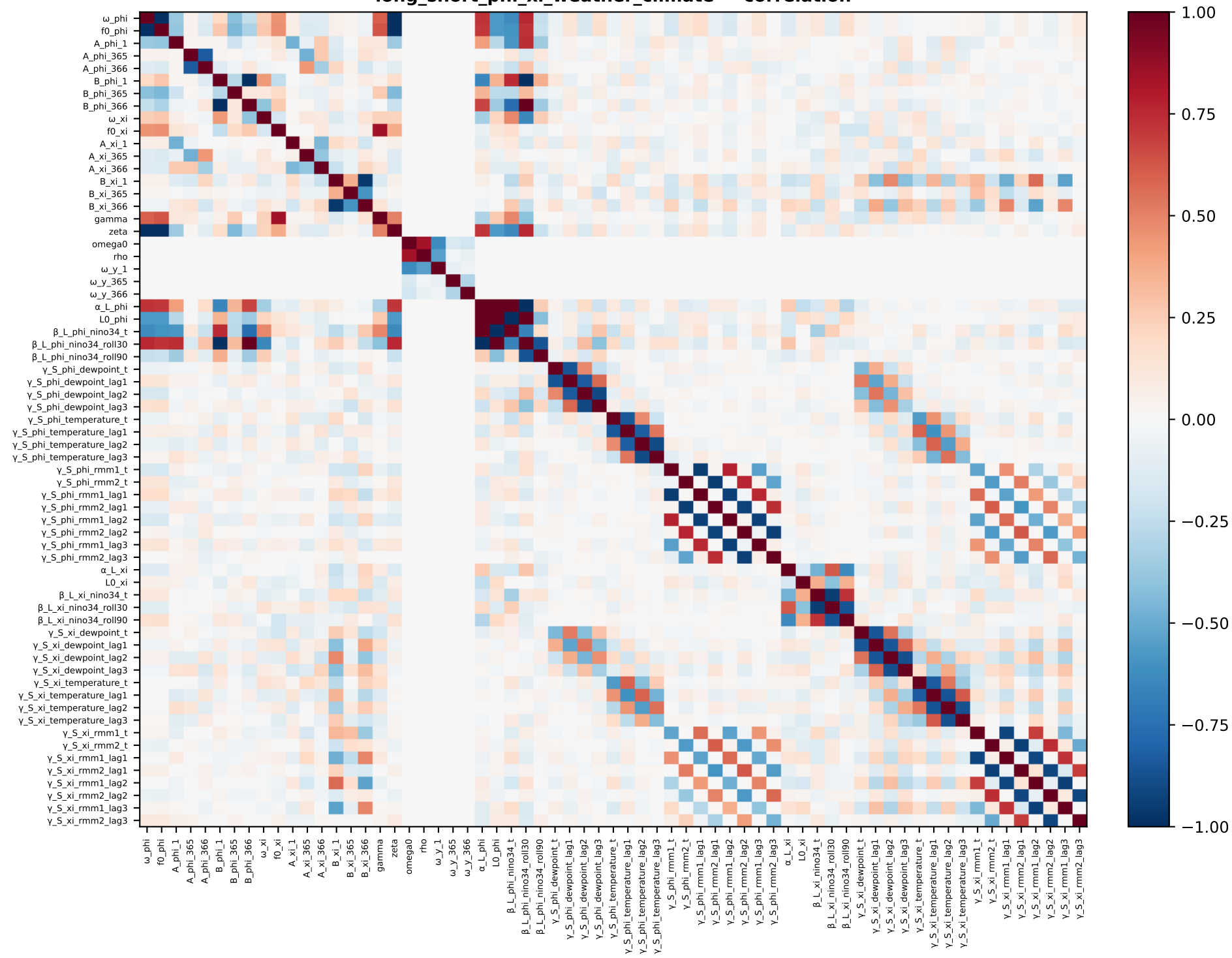
long_short_phi_xi_weather_climate — correlation
