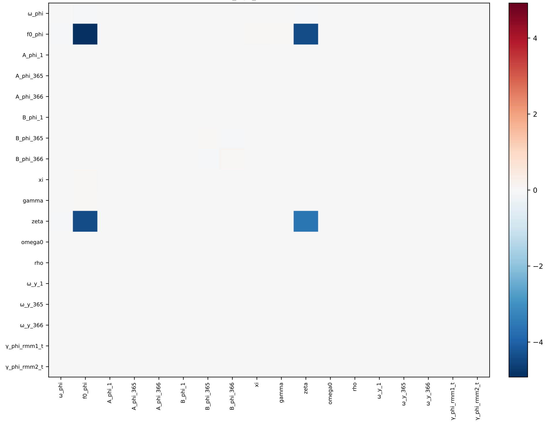
phi_mjo_t — covariance
