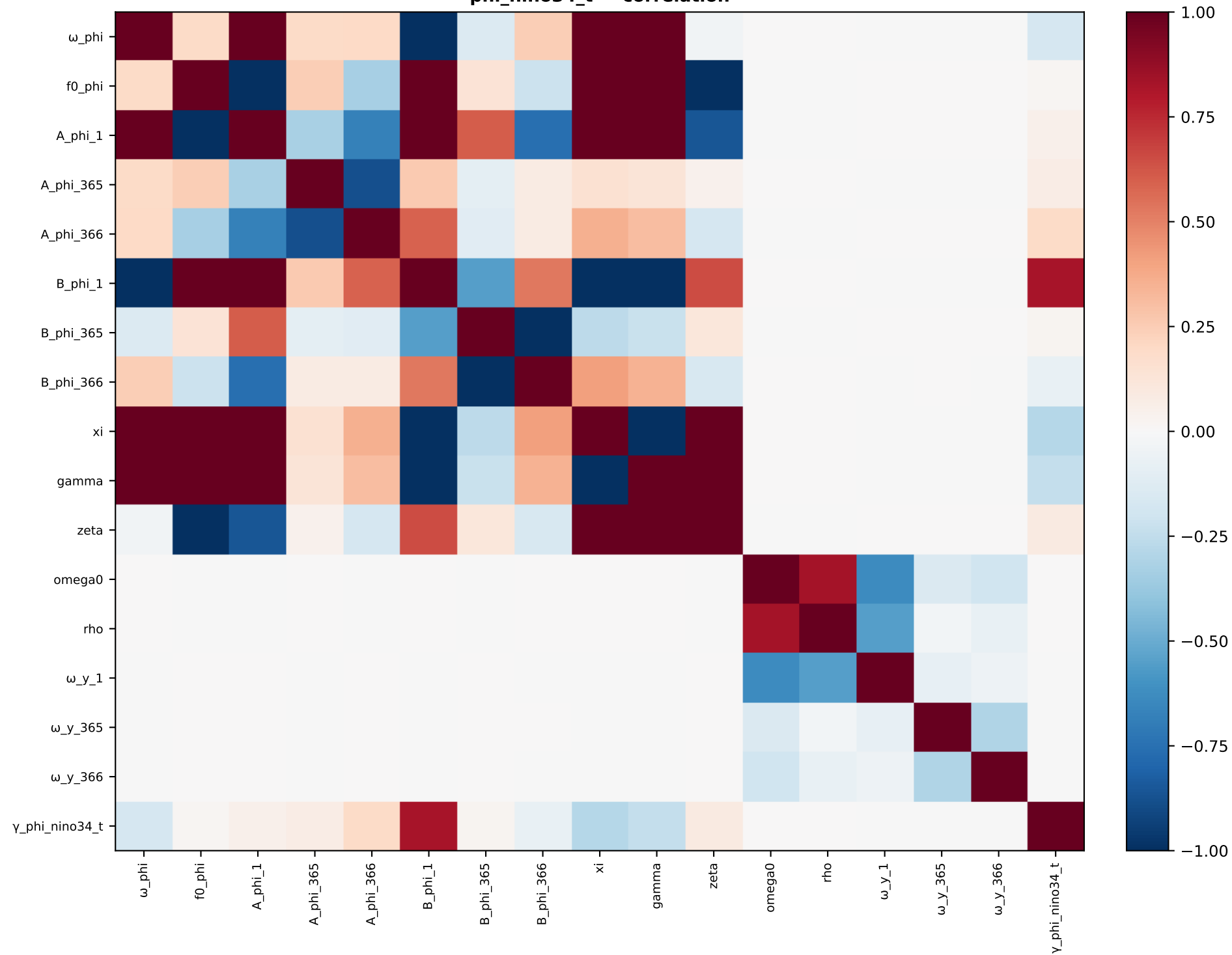
phi_nino34_t — correlation
