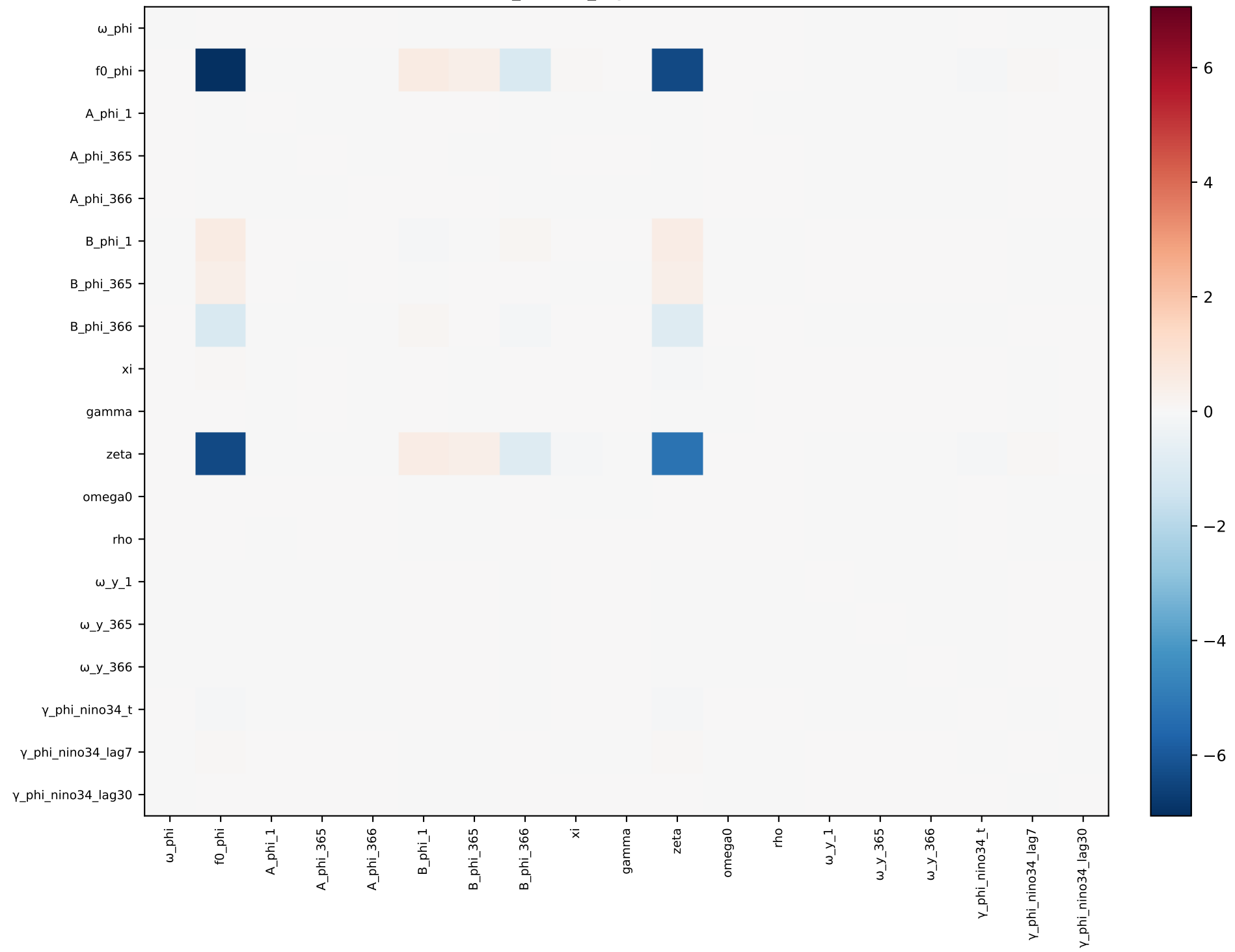
phi_nino34_lags — covariance
