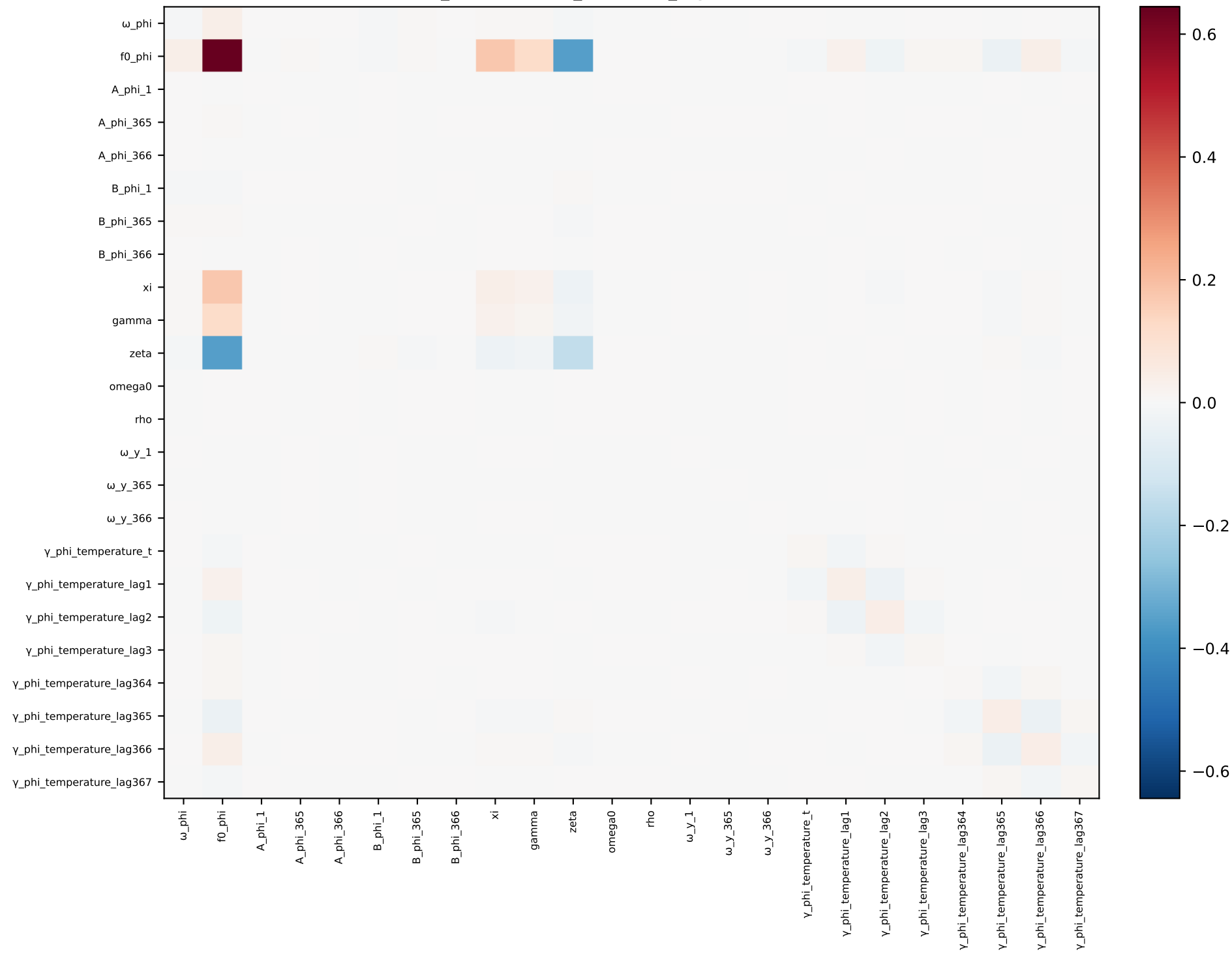
phi_temperature_seasonal_lags — covariance
