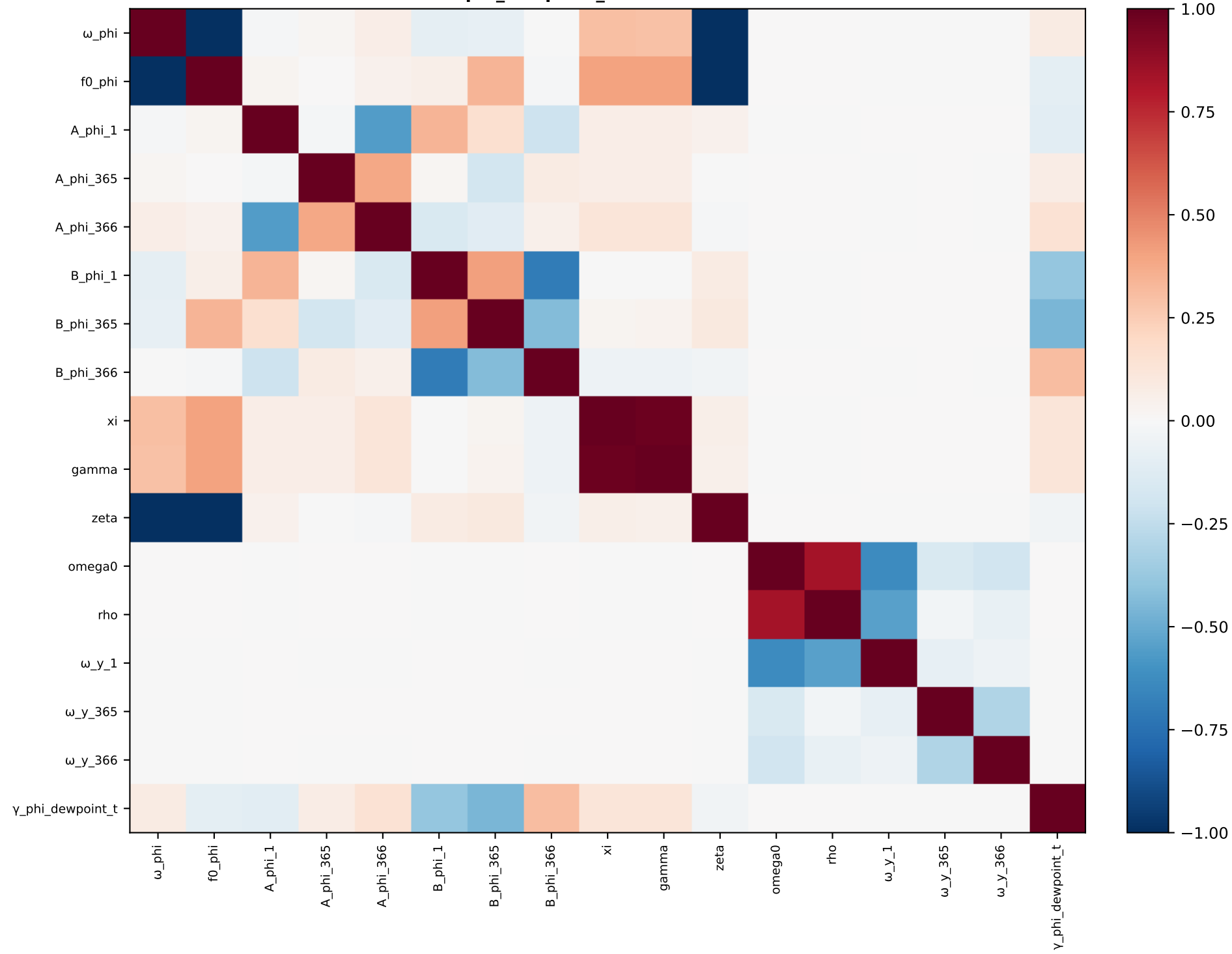
phi_dewpoint_t — correlation
