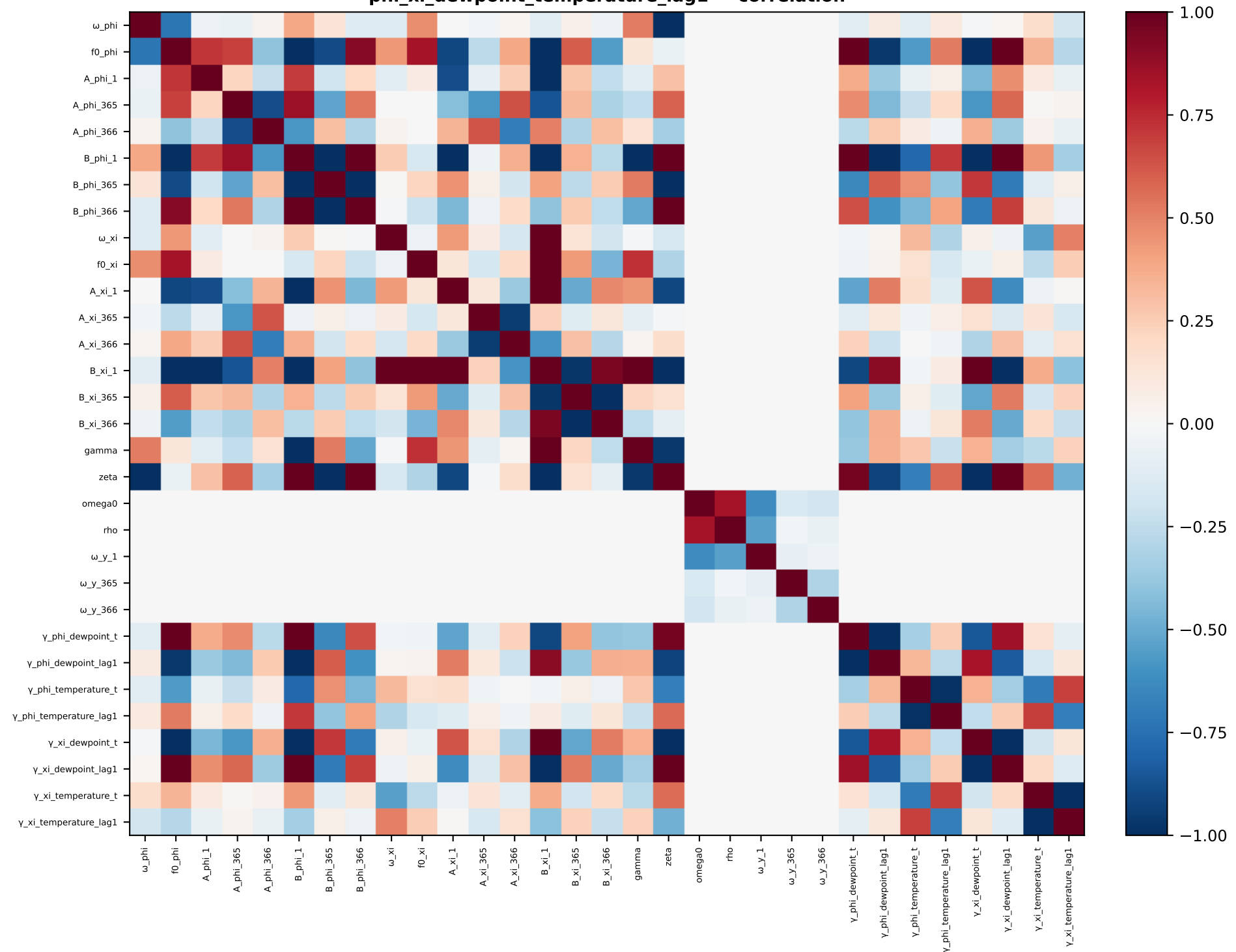
phi_xi_dewpoint_temperature_lag1 — correlation
