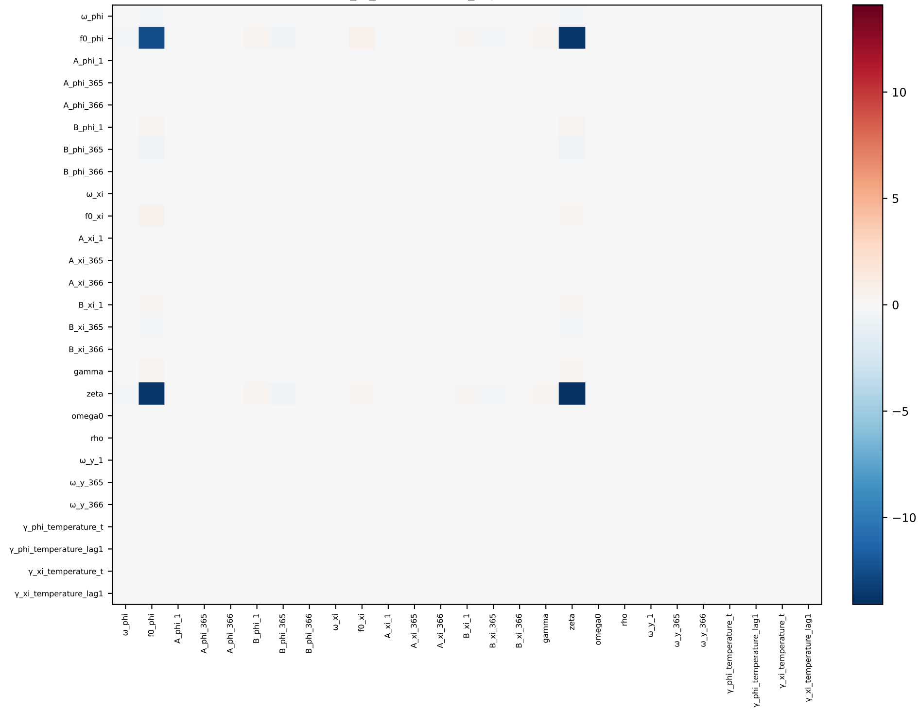
phi_xi_temperature_lag1 — covariance
