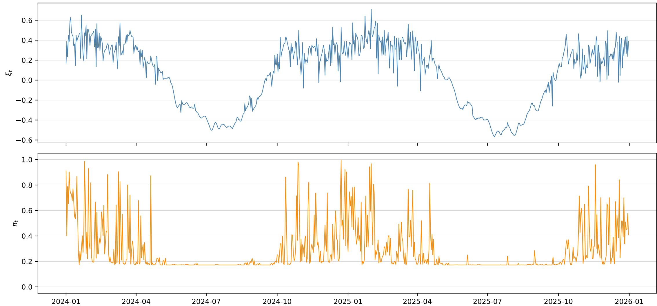
xi_interaction_temperature_nino34 — filtered states (OOS)
