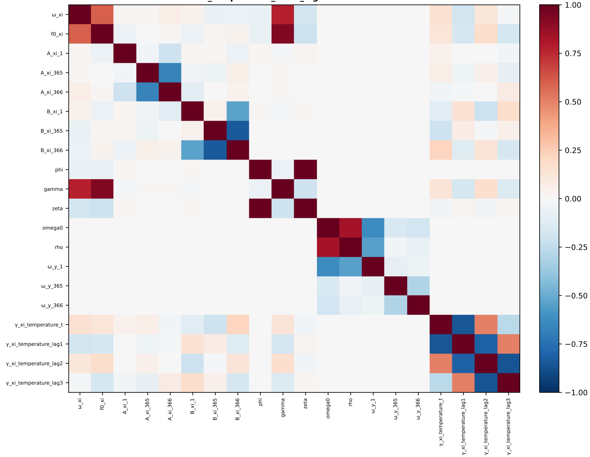
xi_temperature_short_lags — correlation
