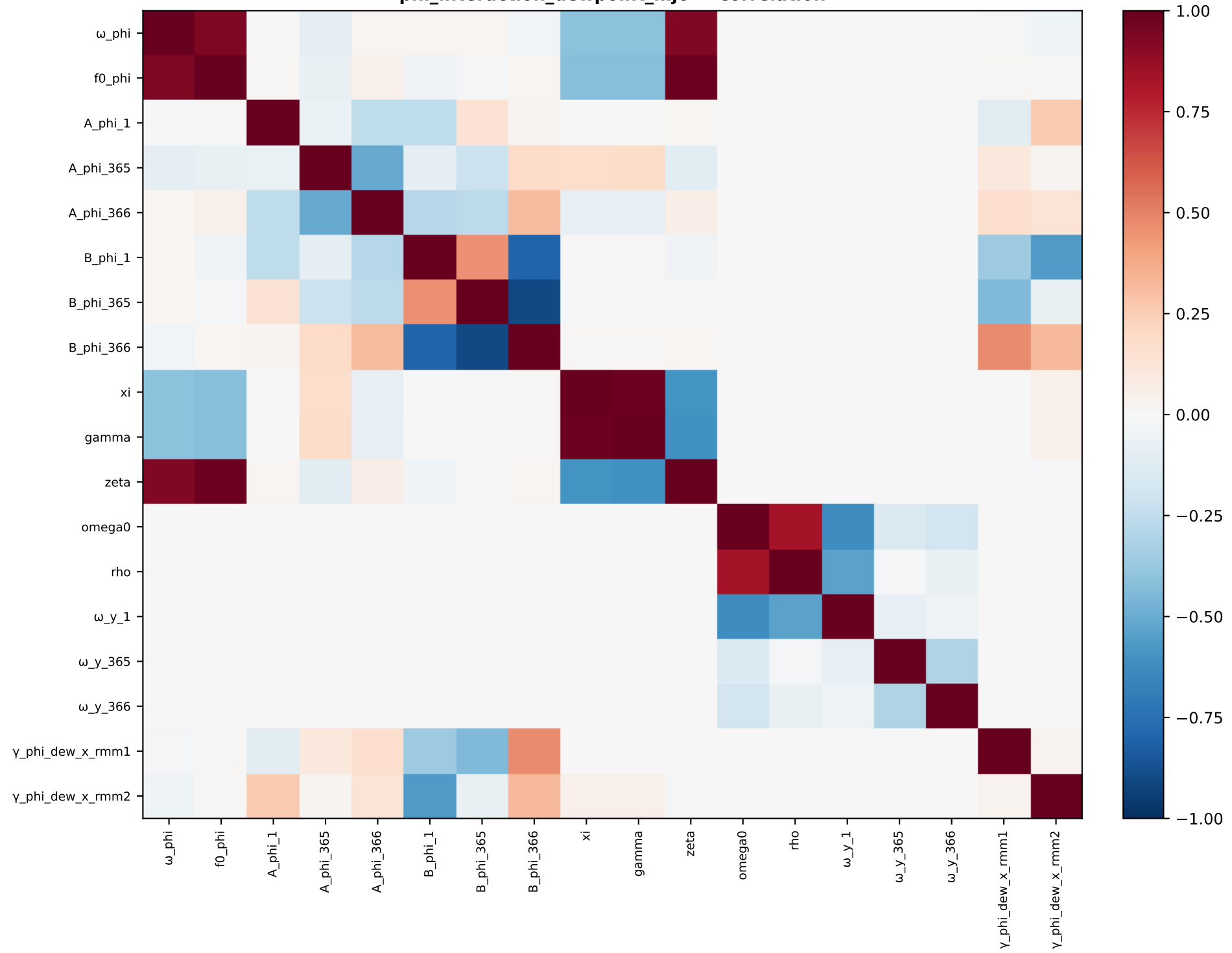
phi_interaction_dewpoint_mjo — correlation
