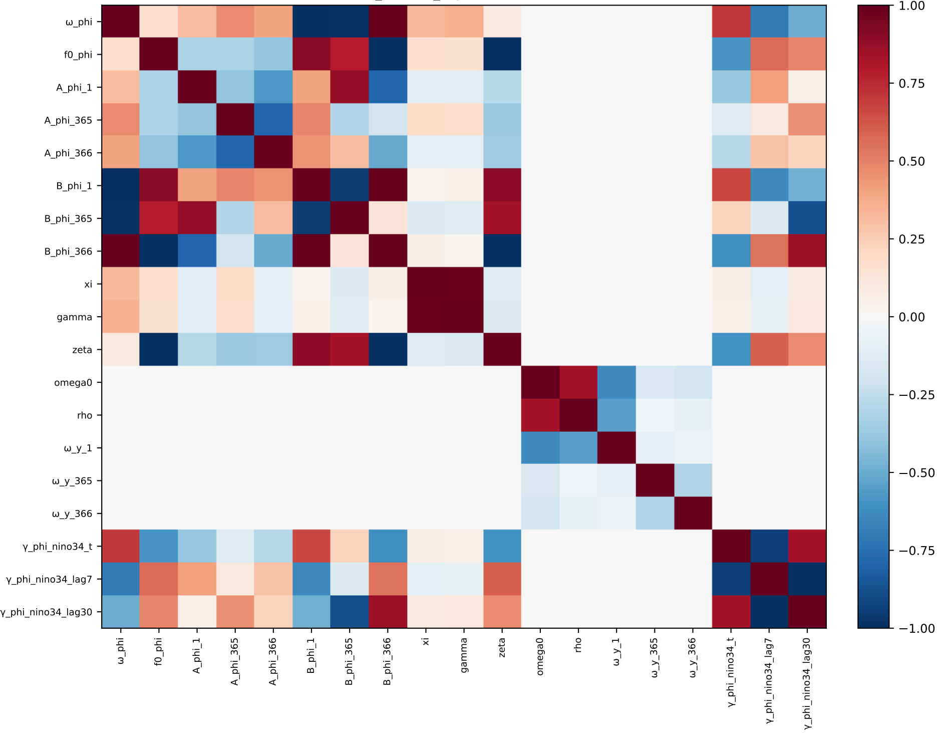
phi_nino34_lags — correlation
