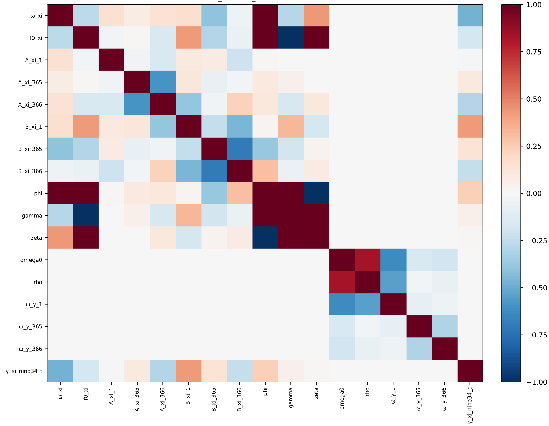
xi_nino34_t — correlation
