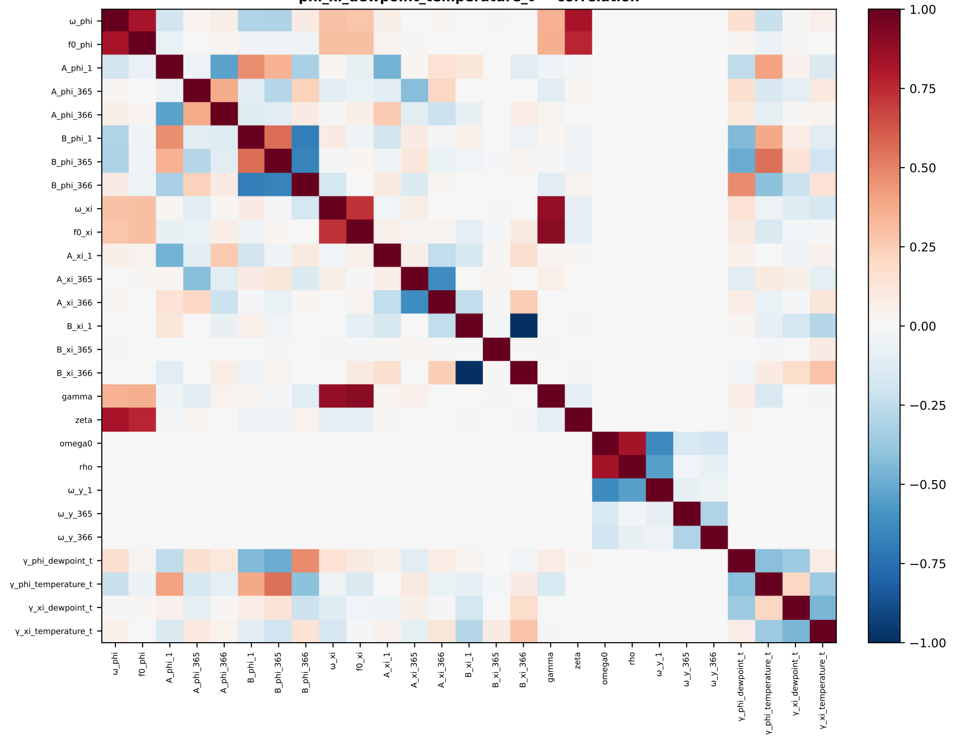
phi_xi_dewpoint_temperature_t — correlation
