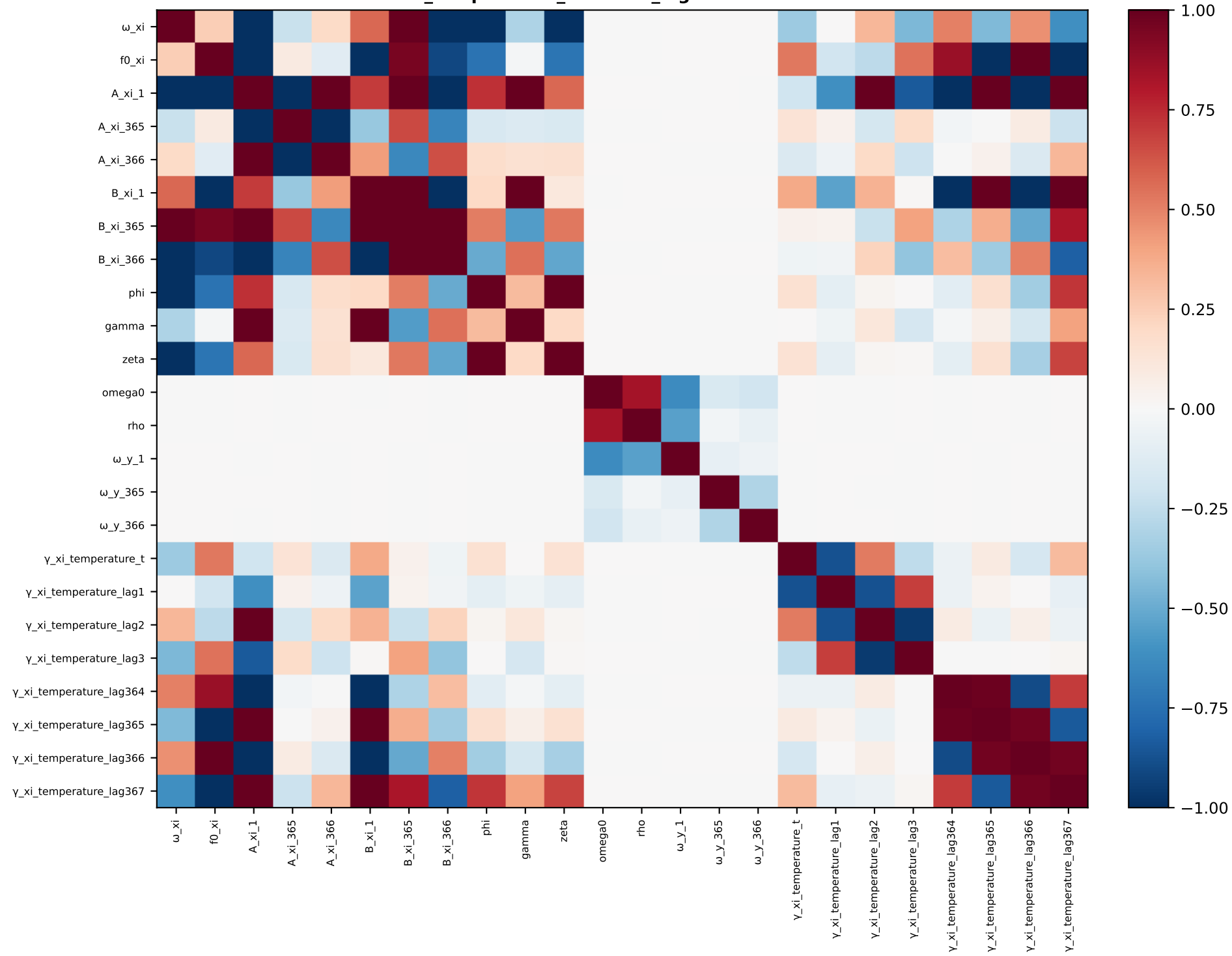
xi_temperature_seasonal_lags — correlation
