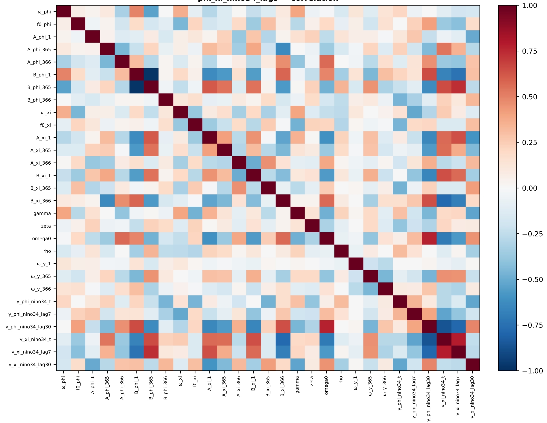
phi_xi_nino34_lags — correlation
