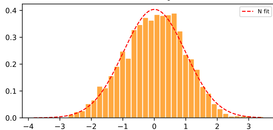
Normalised histogram
