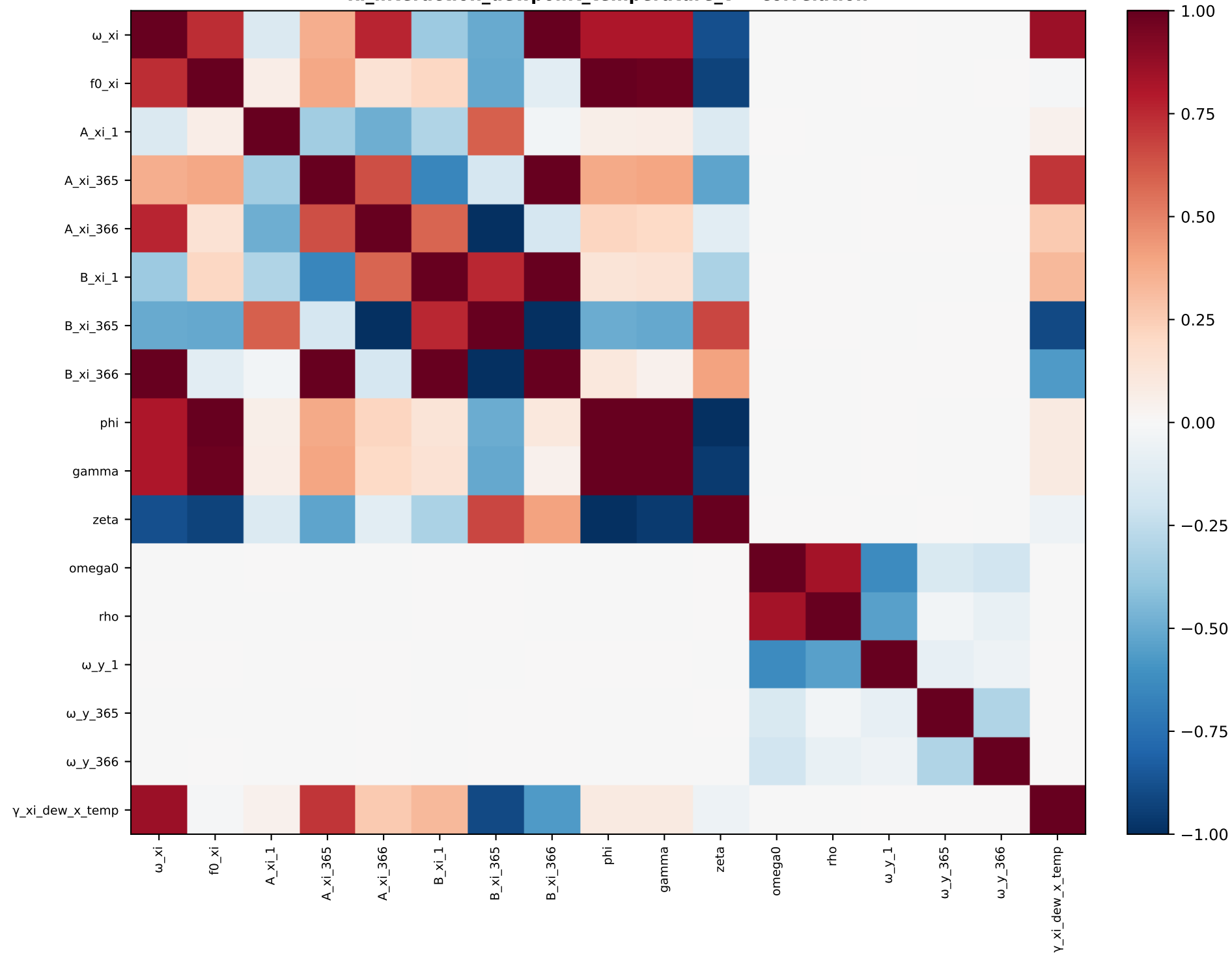
xi_interaction_dewpoint_temperature_t — correlation
