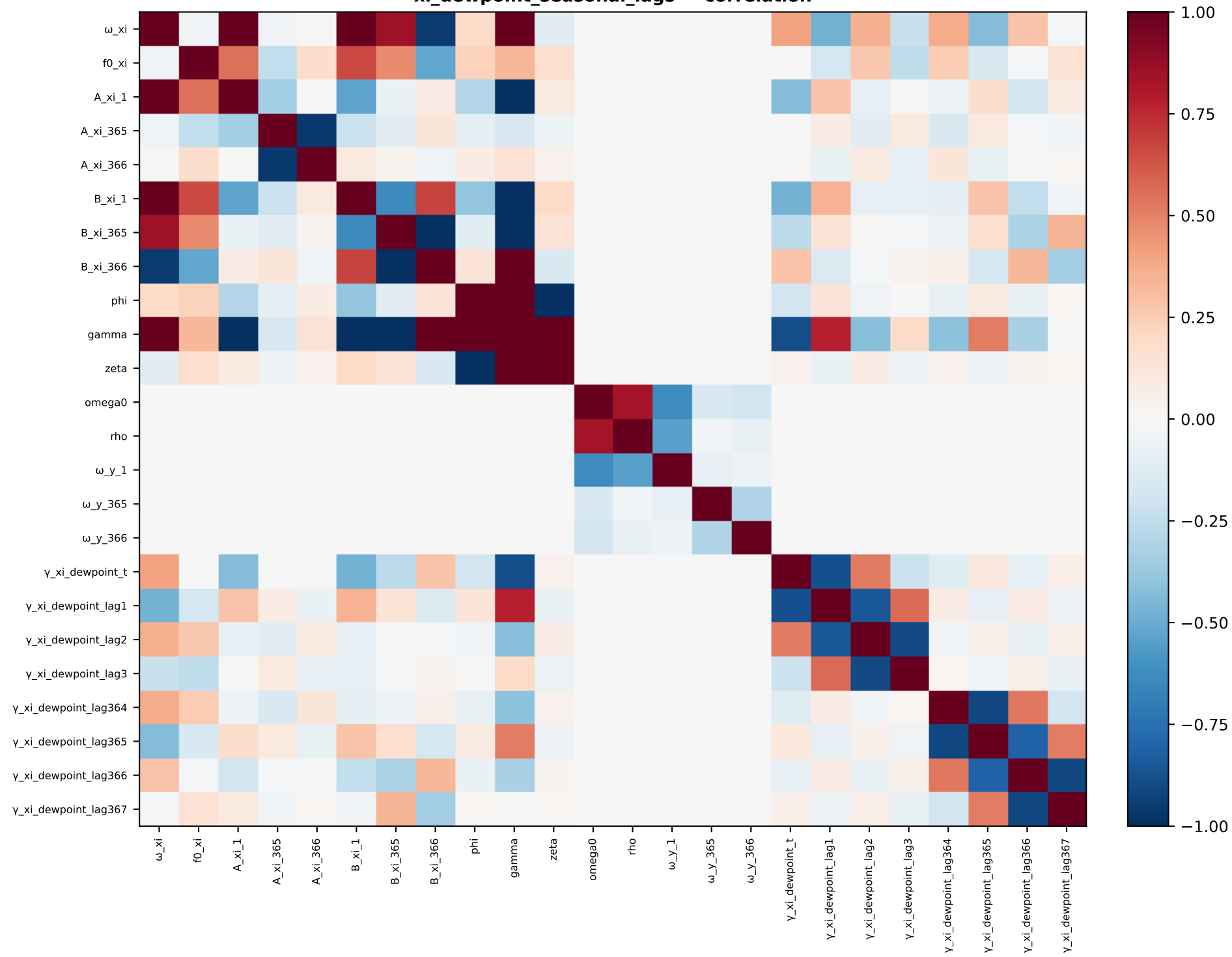
xi_dewpoint_seasonal_lags — correlation
