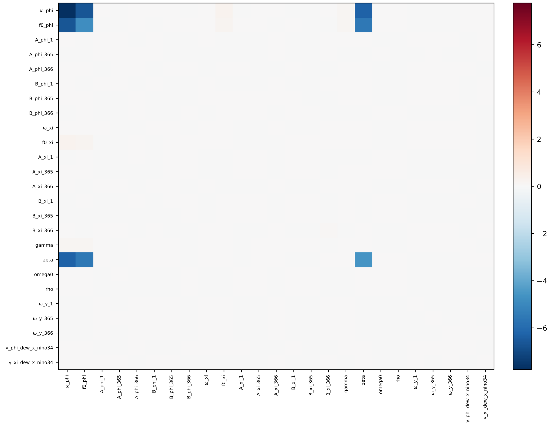
phi_xi_interaction_dewpoint_nino34 — covariance
