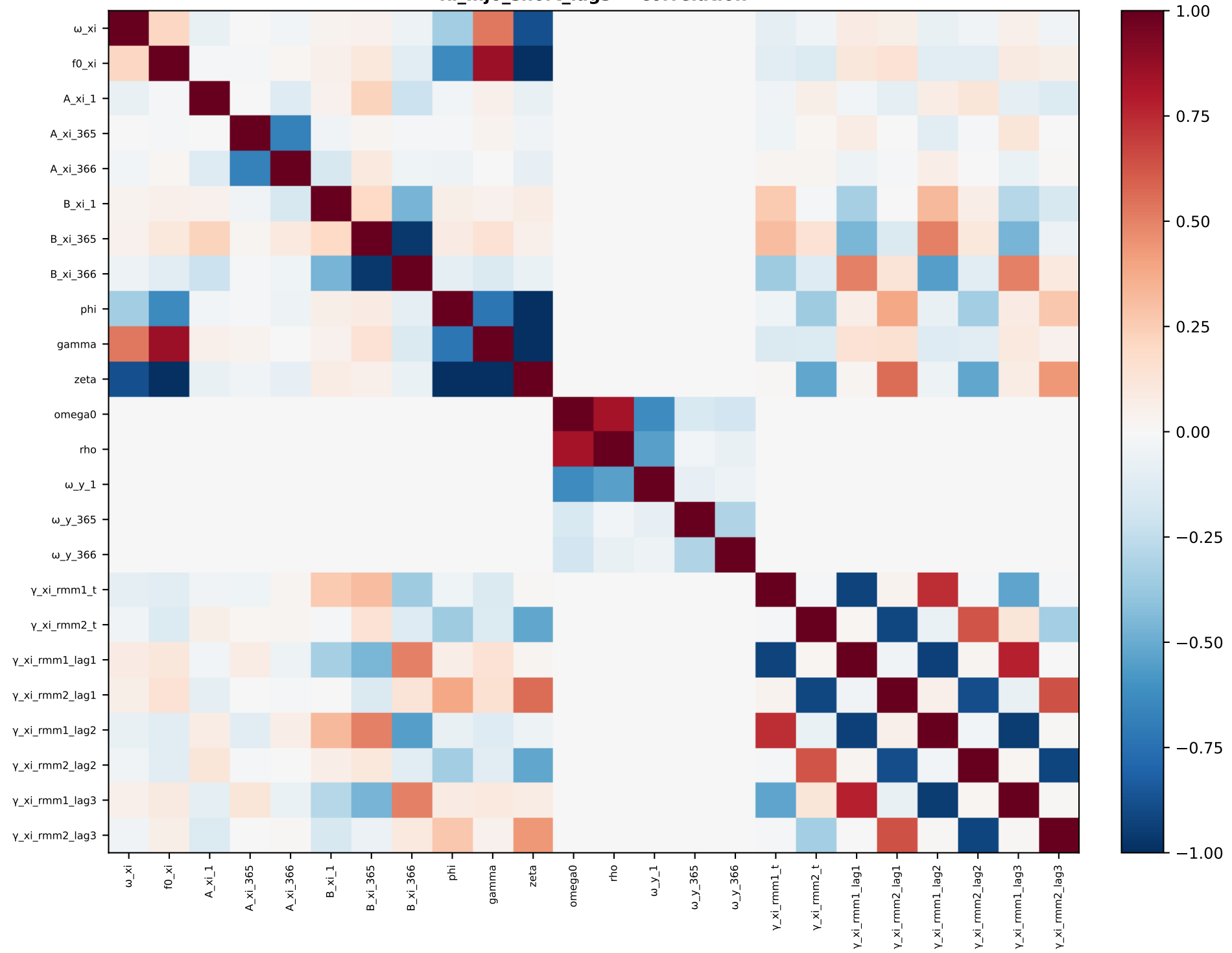
xi_mjo_short_lags — correlation
