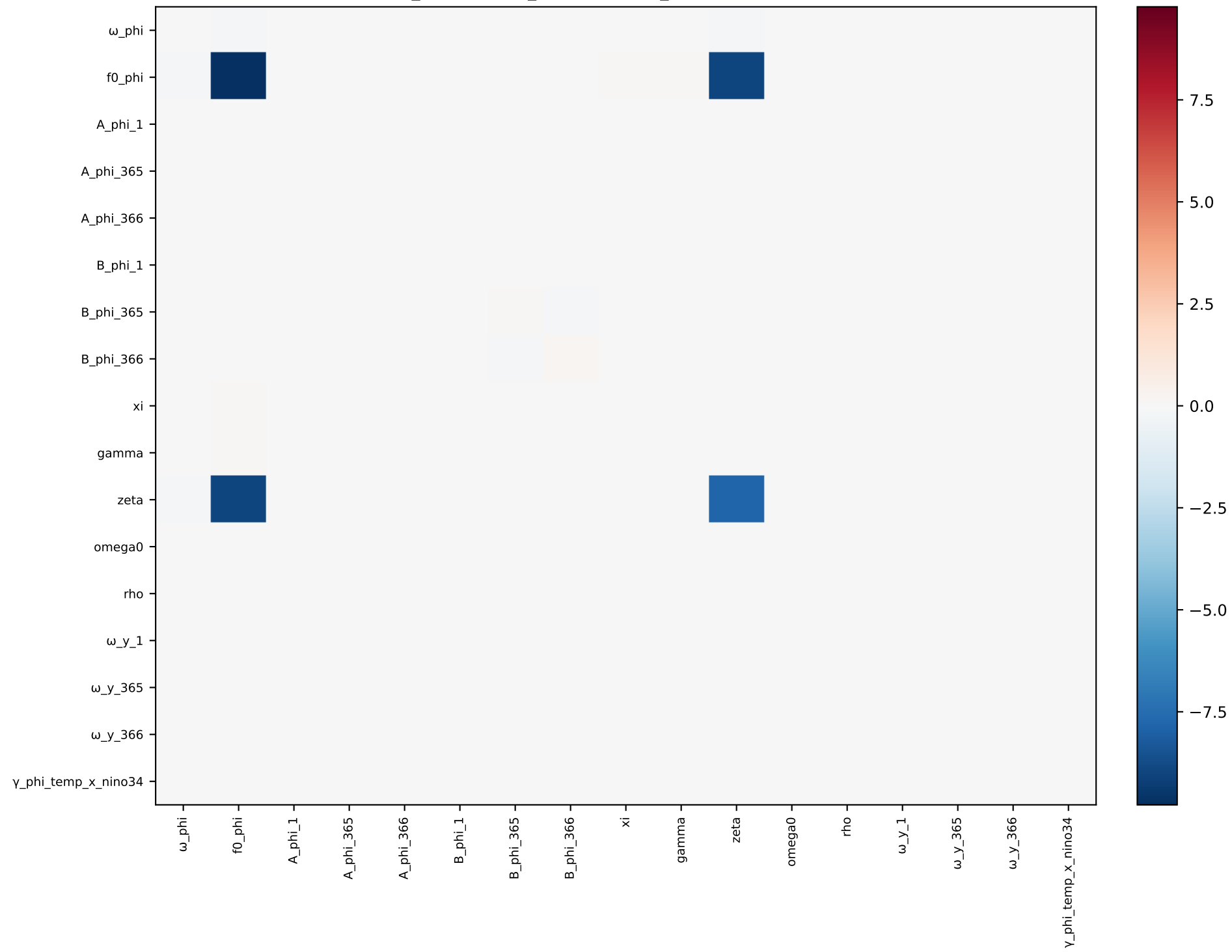
phi_interaction_temperature_nino34 — covariance
