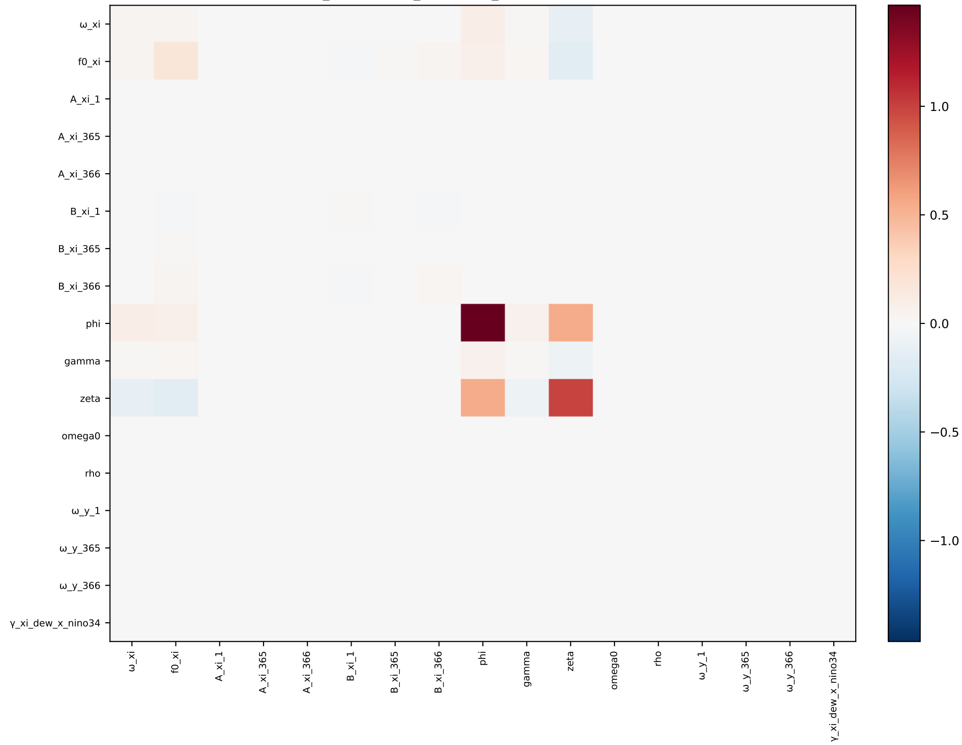
xi_interaction_dewpoint_nino34 — covariance
