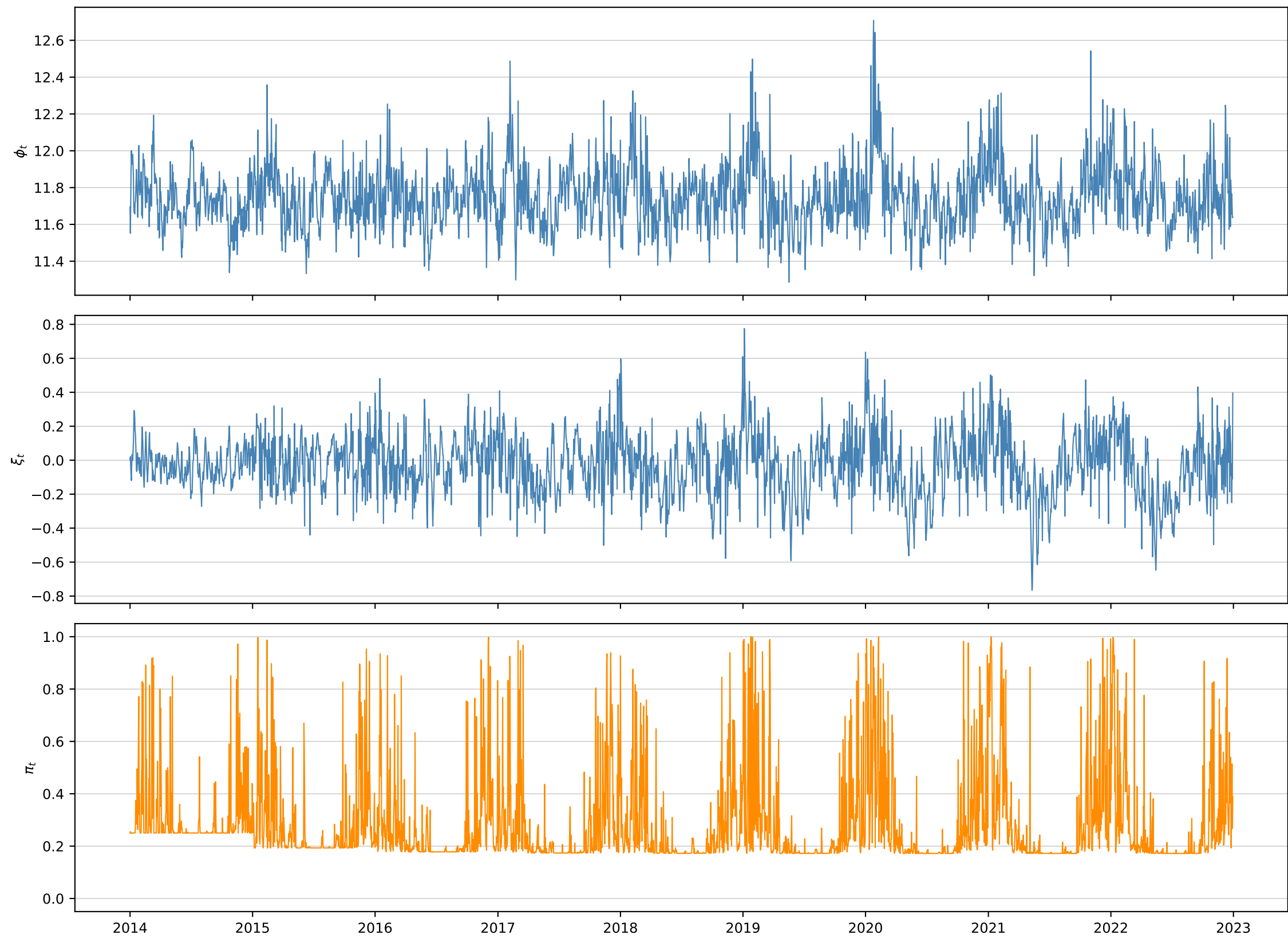
phi_xi_mjo_lag1 — filtered states (IS)
