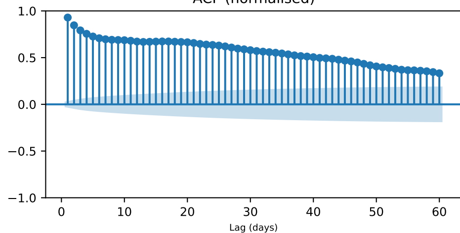
ACF (normalised)
