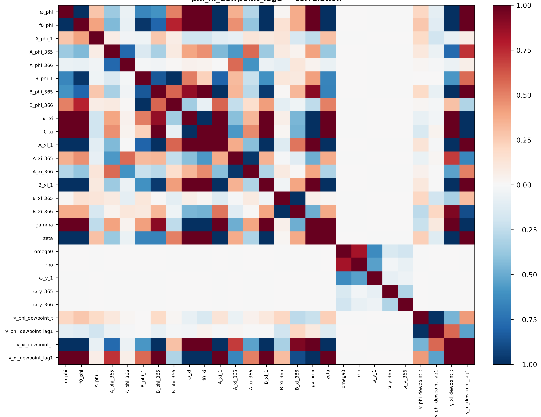
phi_xi_dewpoint_lag1 — correlation
