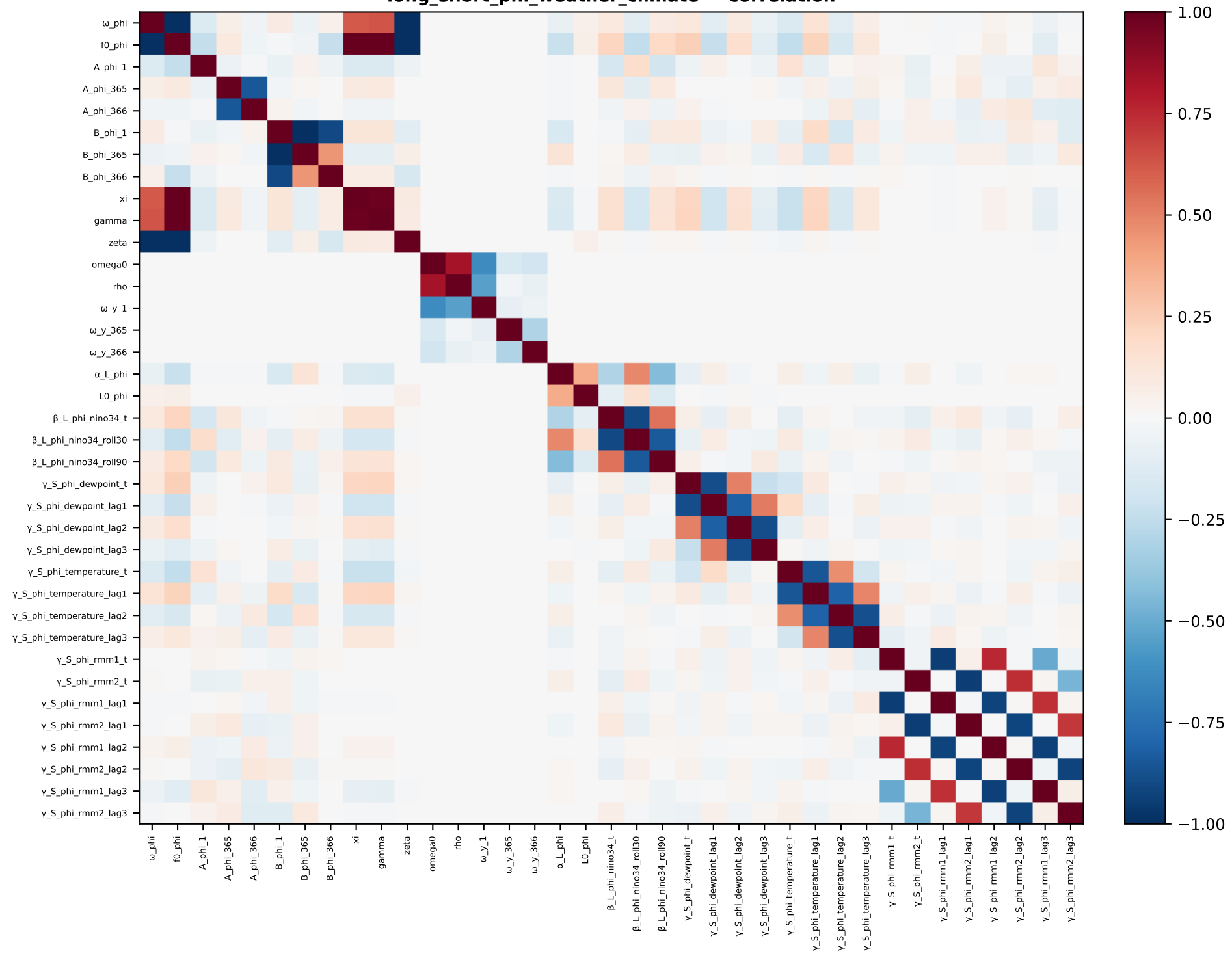
long_short_phi_weather_climate — correlation
