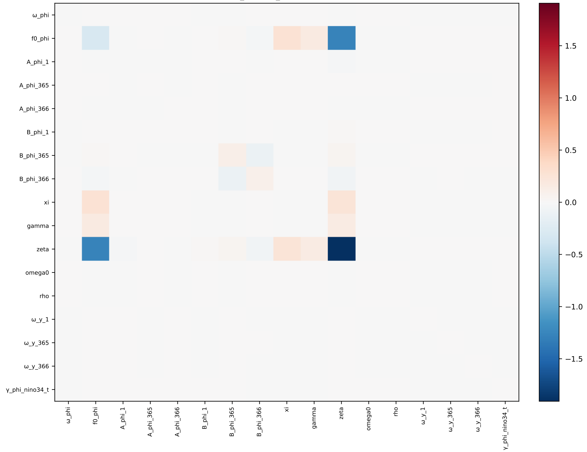
phi_nino34_t – covariance
