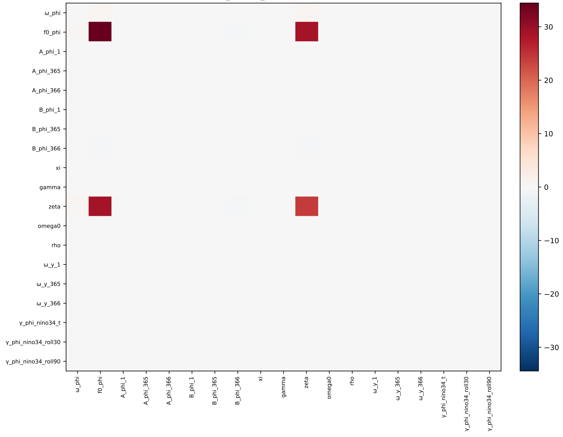
phi_nino34_rolling — covariance
