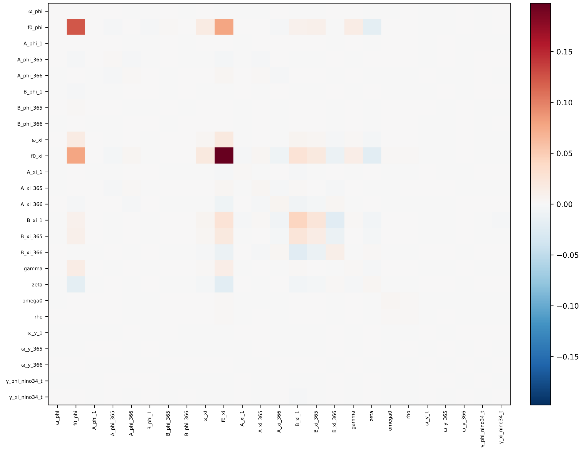
phi_xi_nino34_t — covariance
