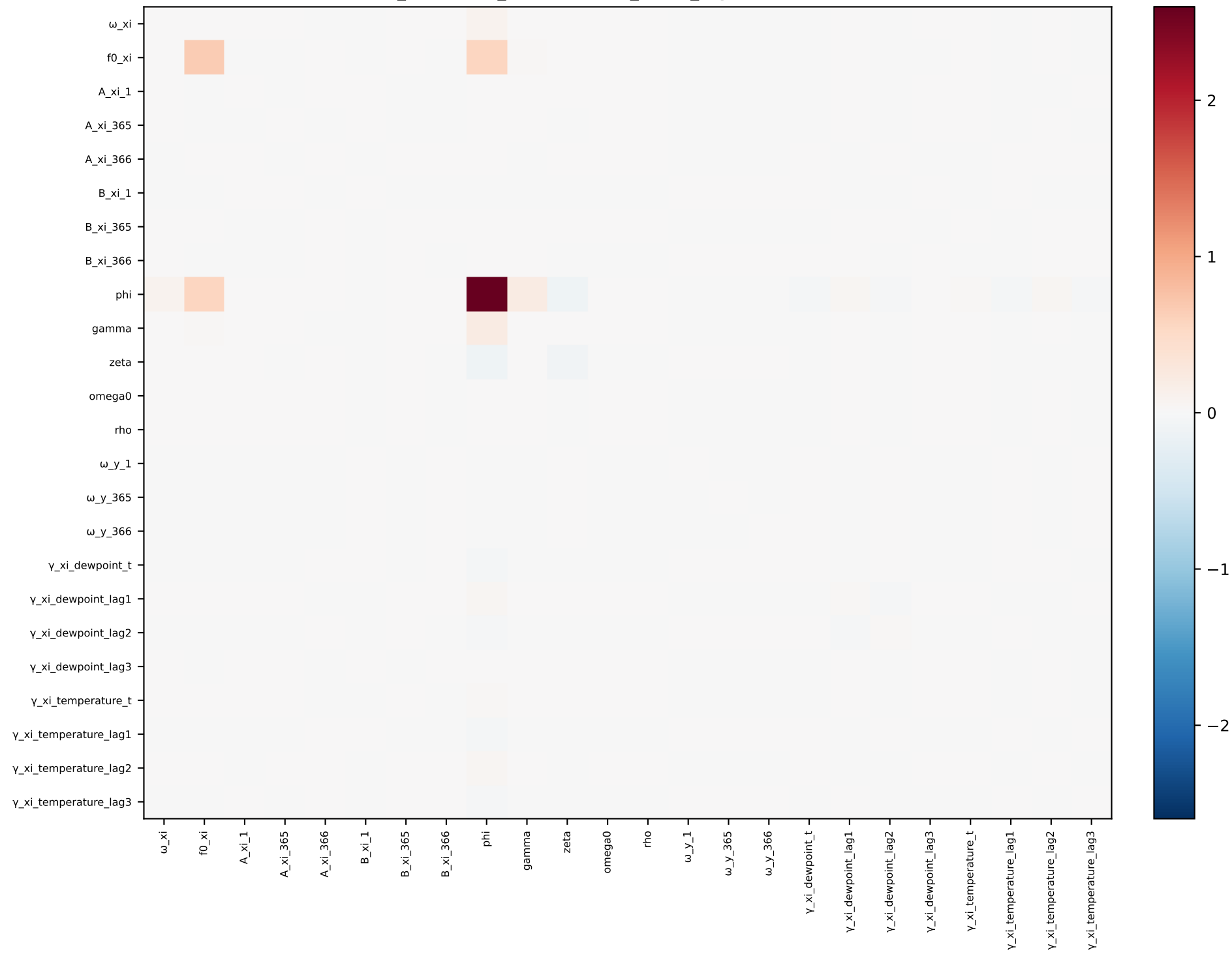
xi_dewpoint_temperature_short_lags — covariance
