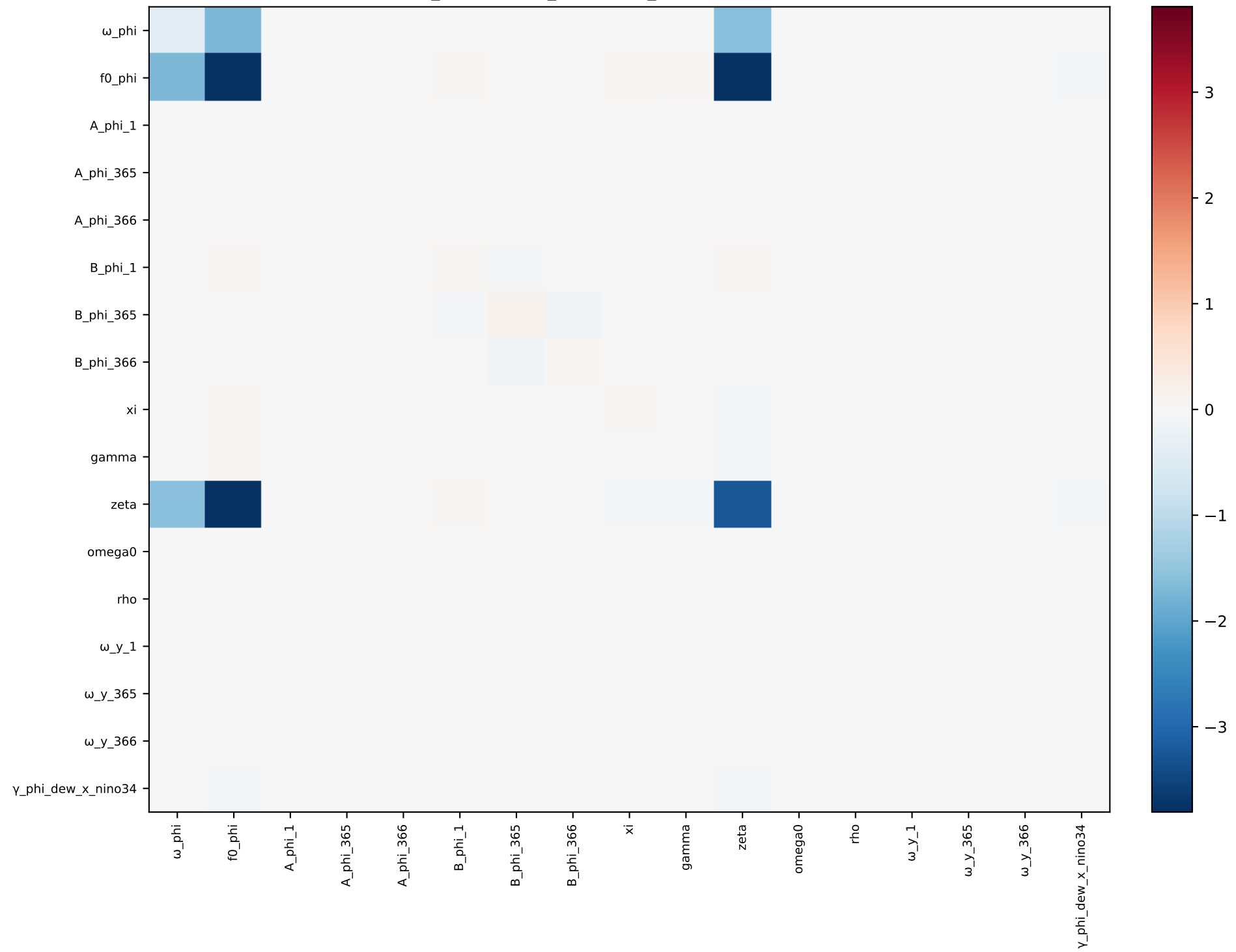
phi_interaction_dewpoint_nino34 — covariance
