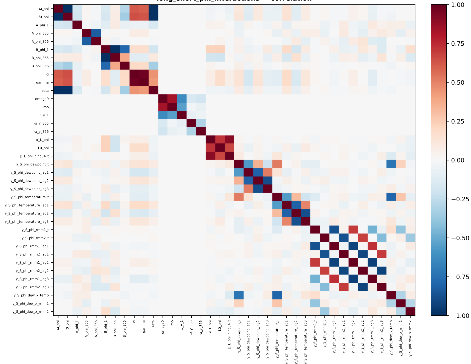
long_short_phi_interactions — correlation
