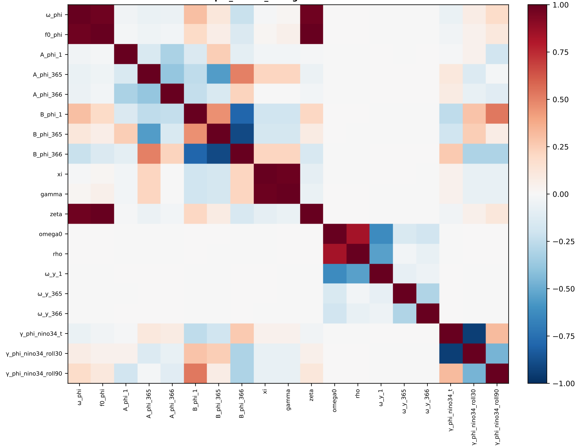
phi_nino34_rolling – correlation
