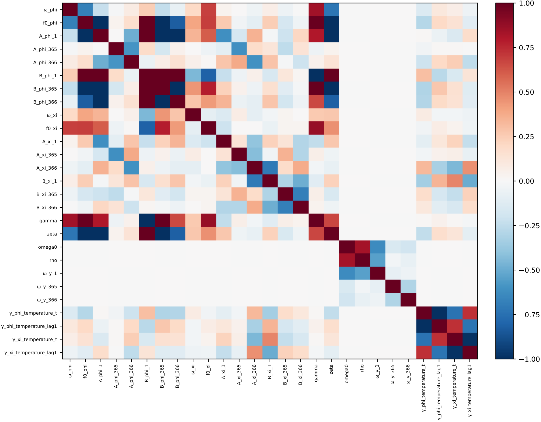
phi_xi_temperature_lag1 — correlation
