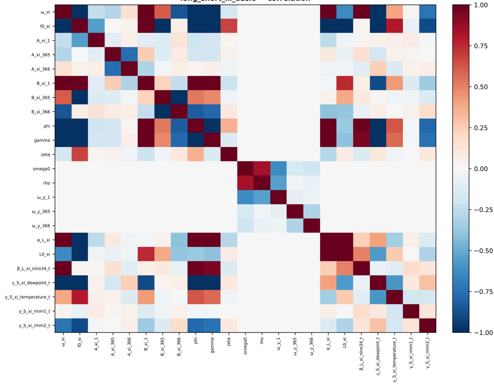
long_short_xi_basic — correlation
