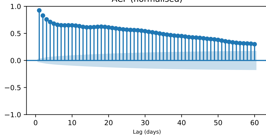
ACF (normalised)
