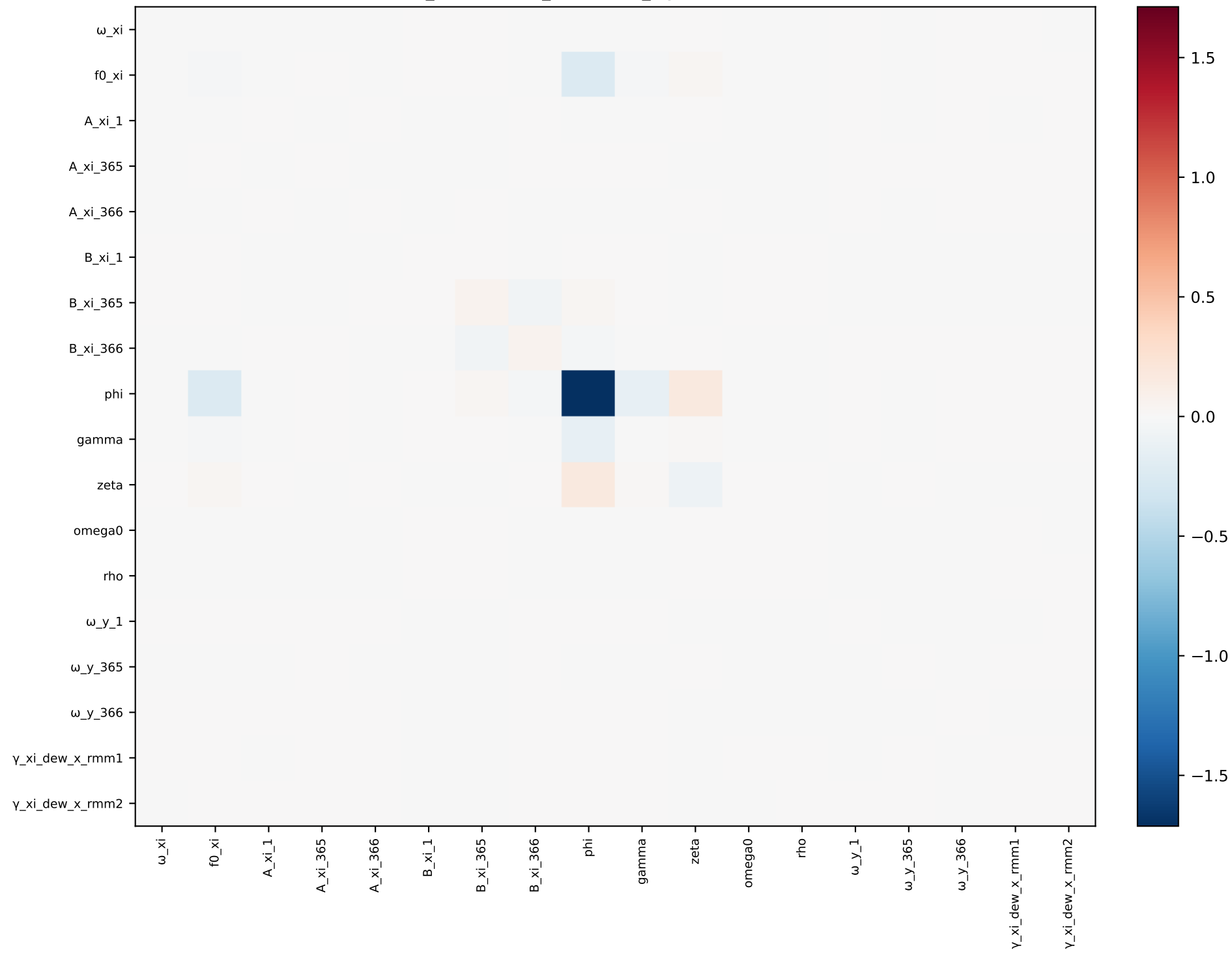
xi_interaction_dewpoint_mjo — covariance
