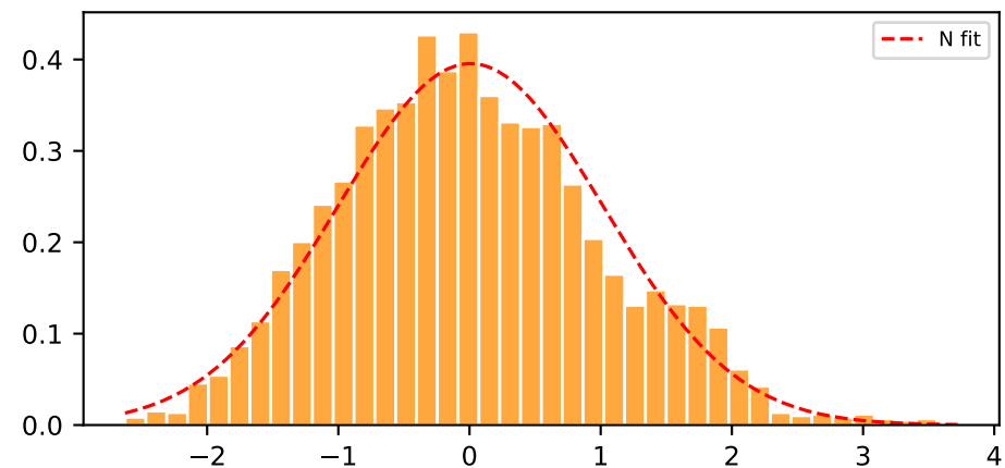
Normalised histogram
