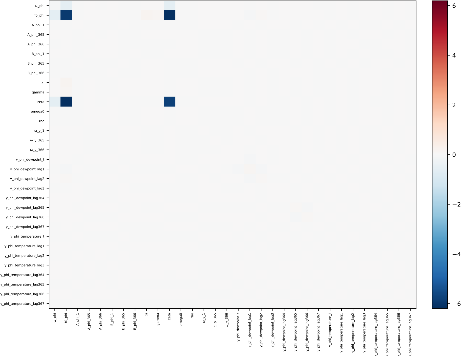
phi_dewpoint_temperature_seasonal_lags – covariance
