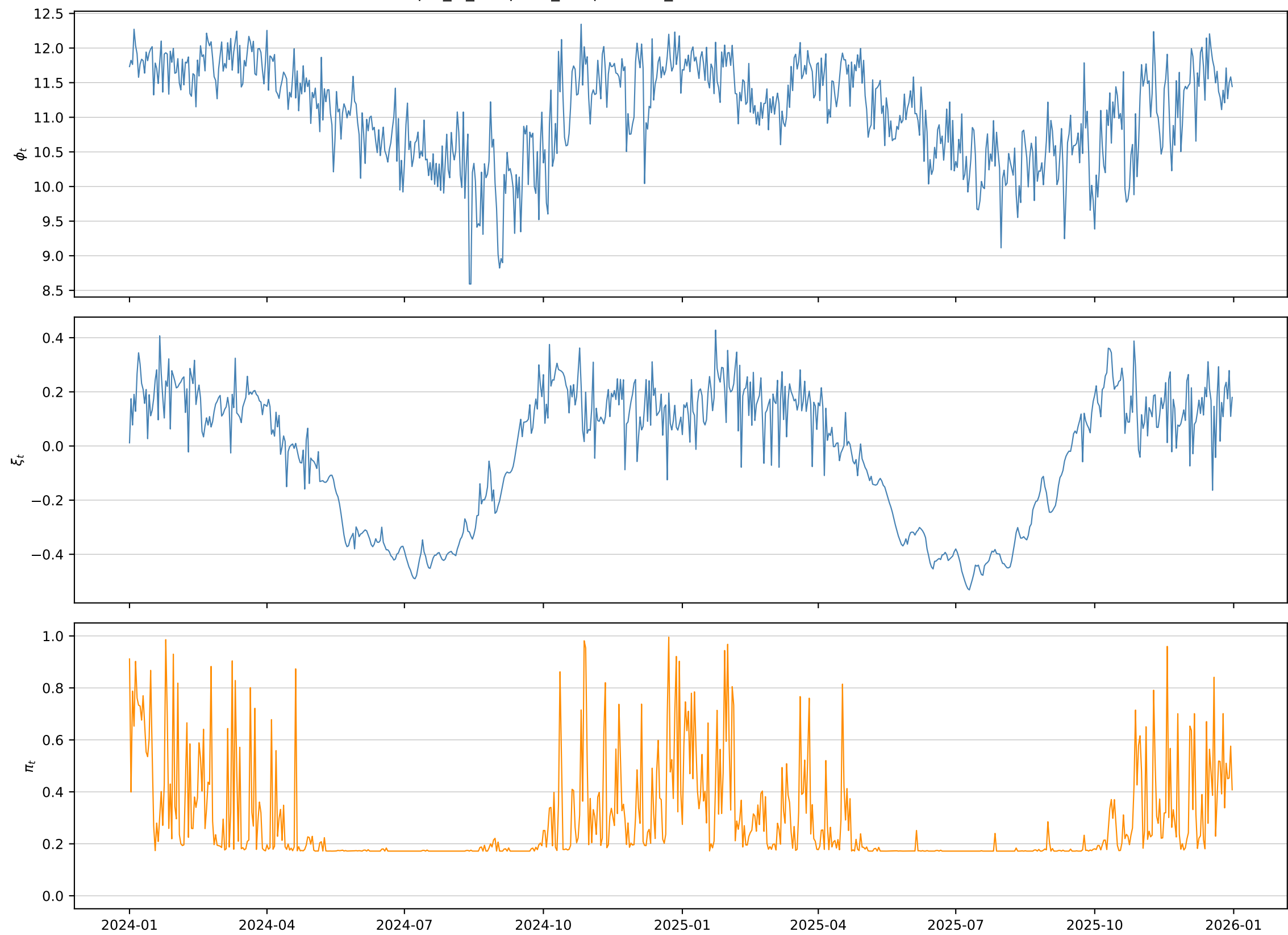
phi_xi_dewpoint_temperature_t — filtered states (OOS)
