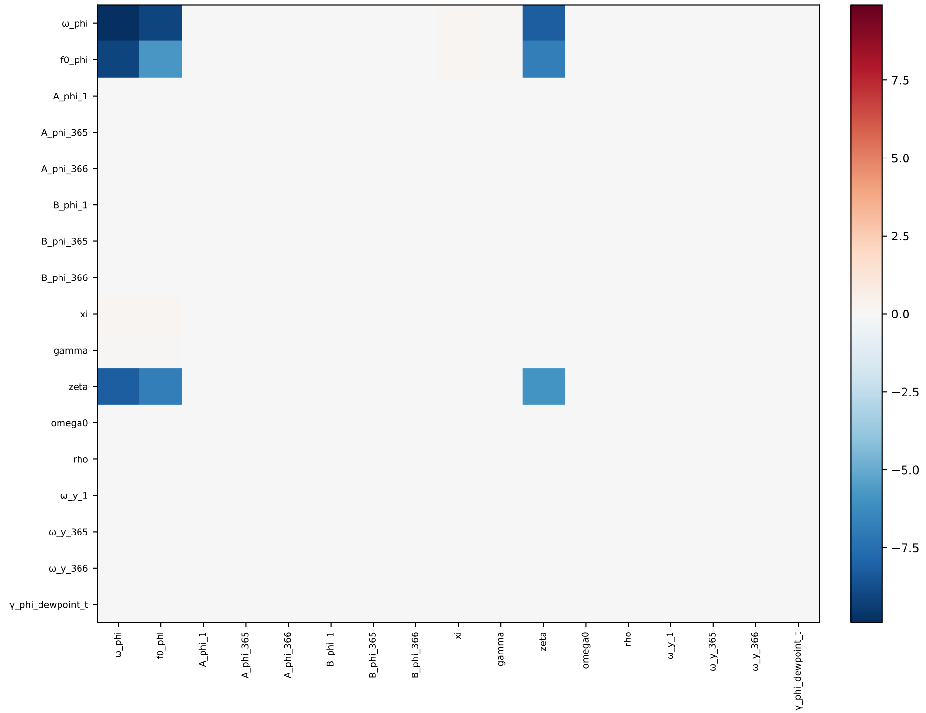
phi_dewpoint_t — covariance
