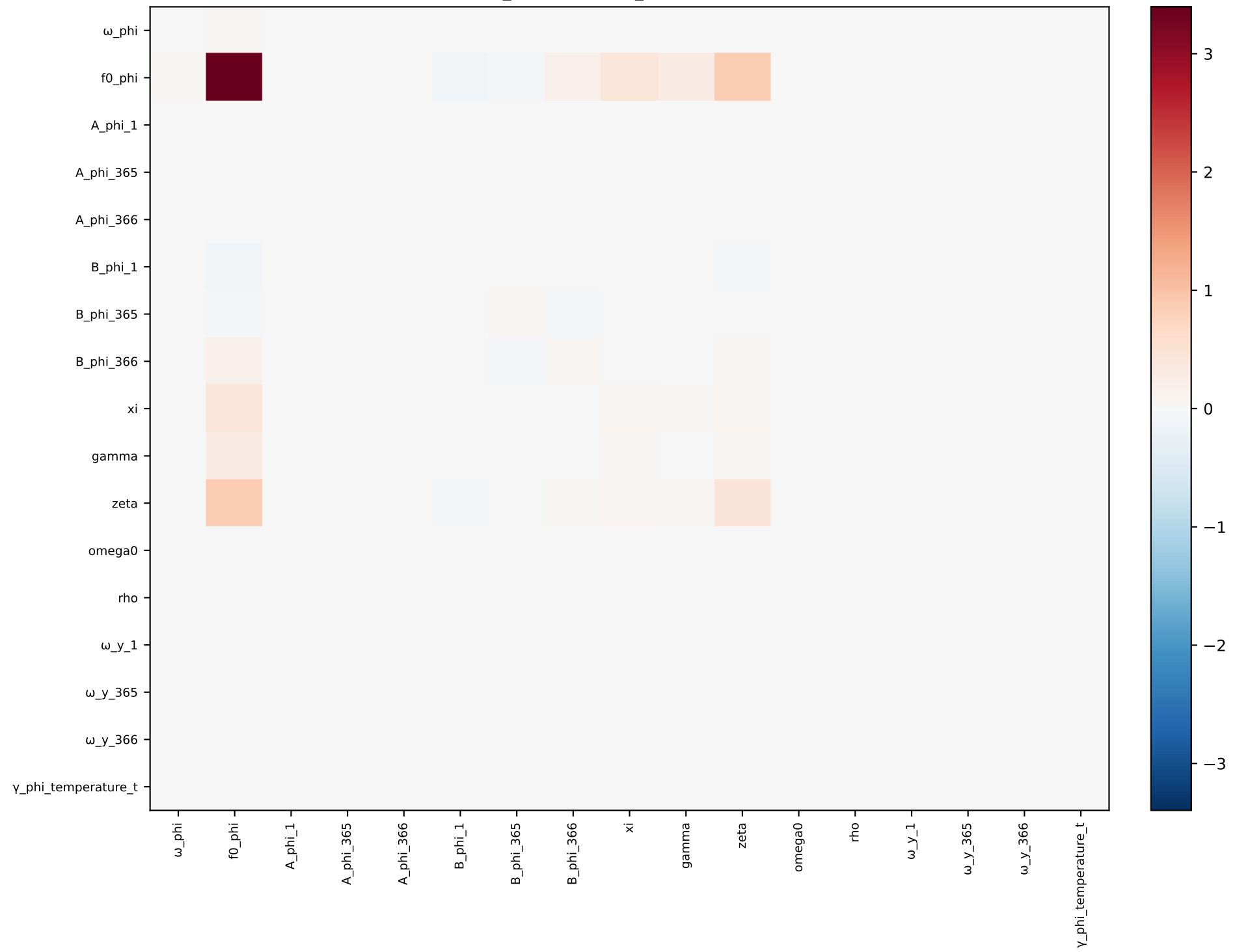
phi_temperature_t — covariance
