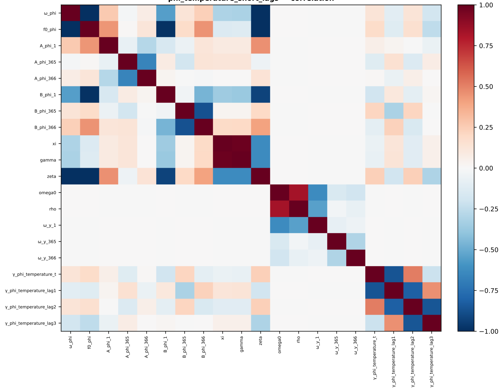
phi_temperature_short_lags — correlation
