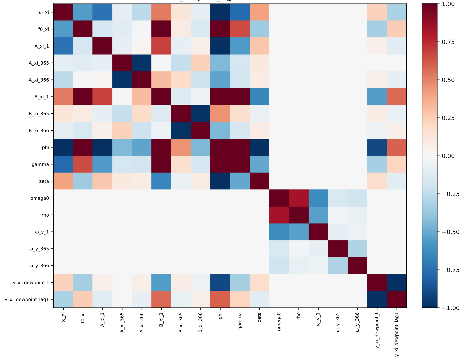
xi_dewpoint_lag1 — correlation
