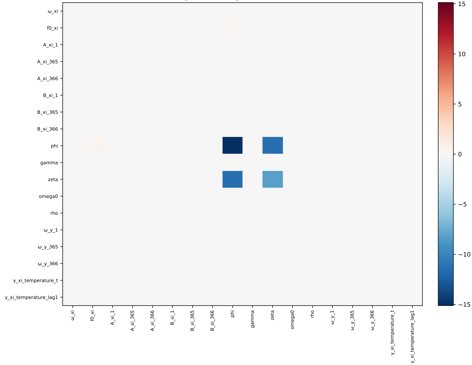
xi_temperature_lag1 — covariance
