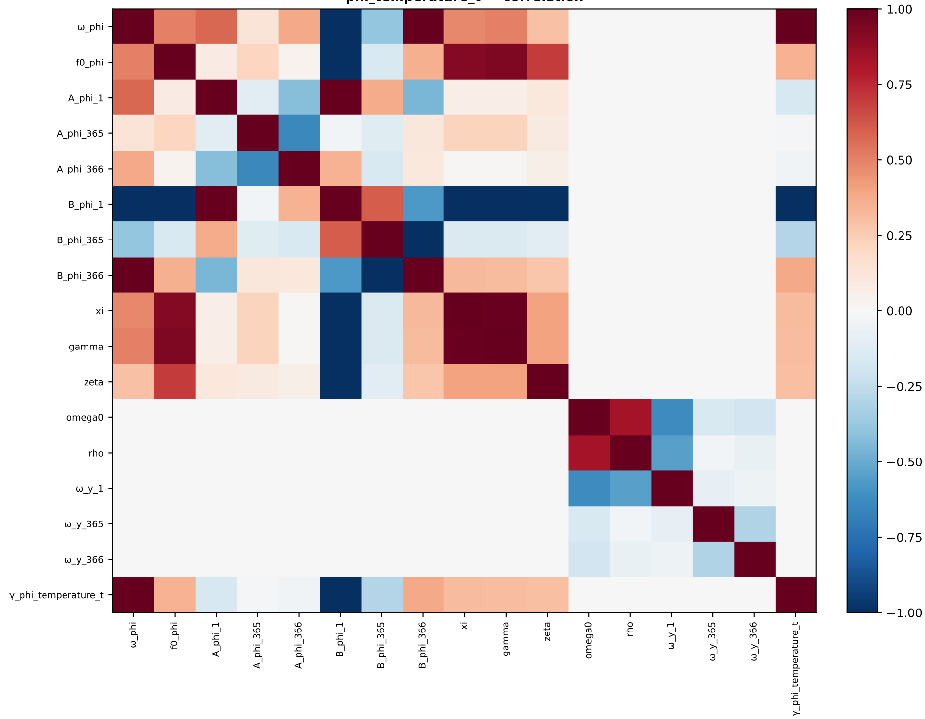
phi_temperature_t — correlation
