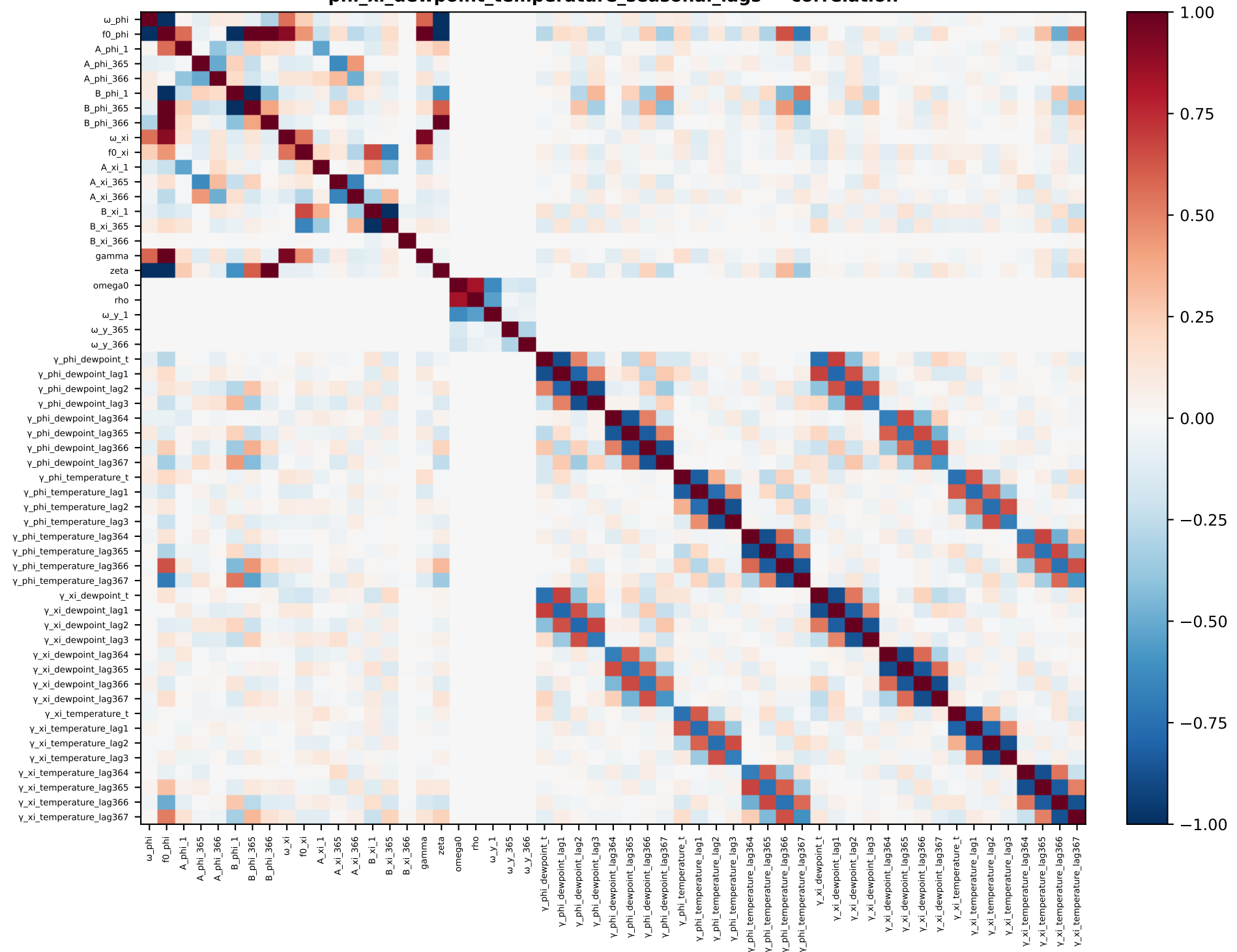
phi_xi_dewpoint_temperature_seasonal_lags — correlation
