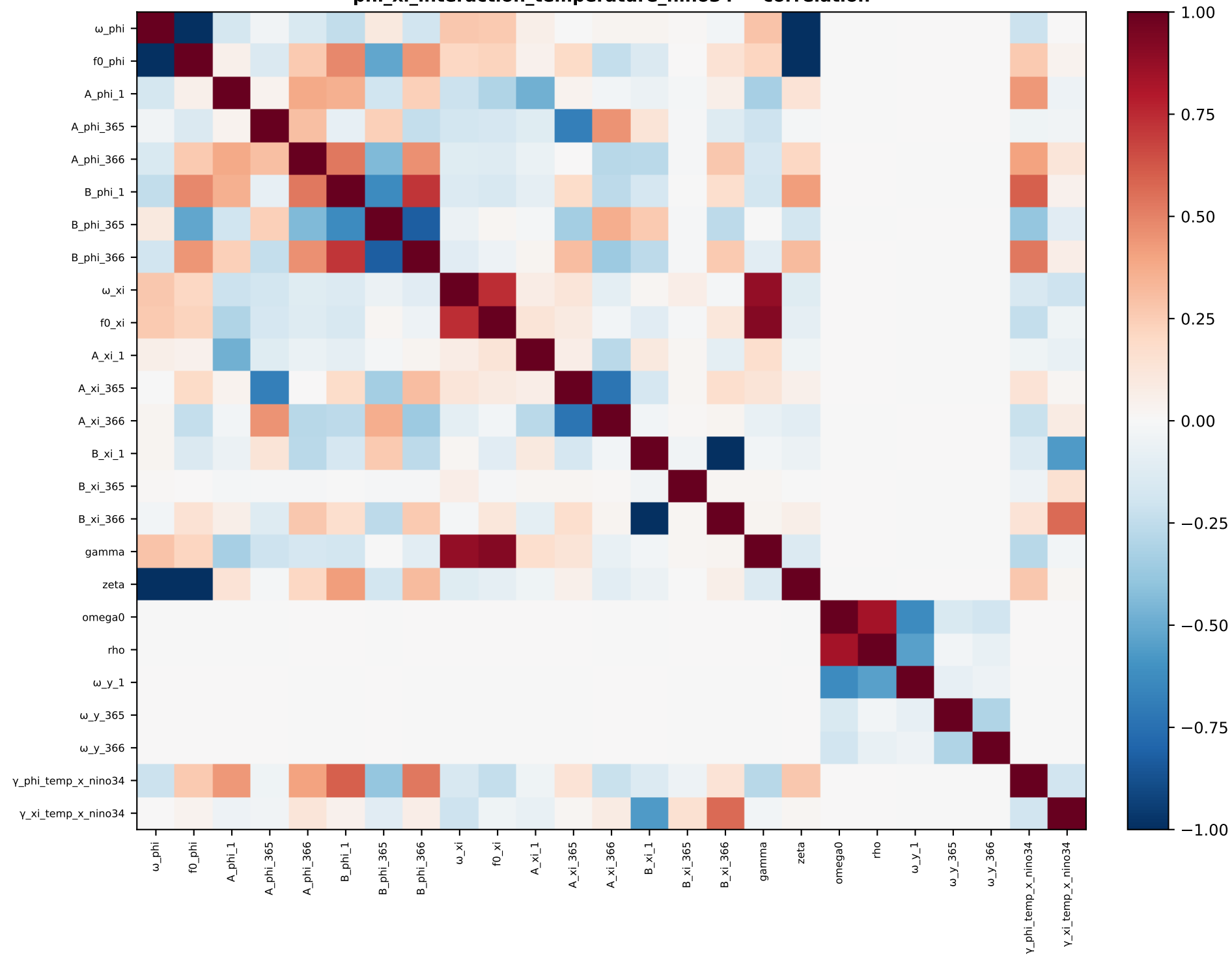
phi_xi_interaction_temperature_nino34 — correlation
