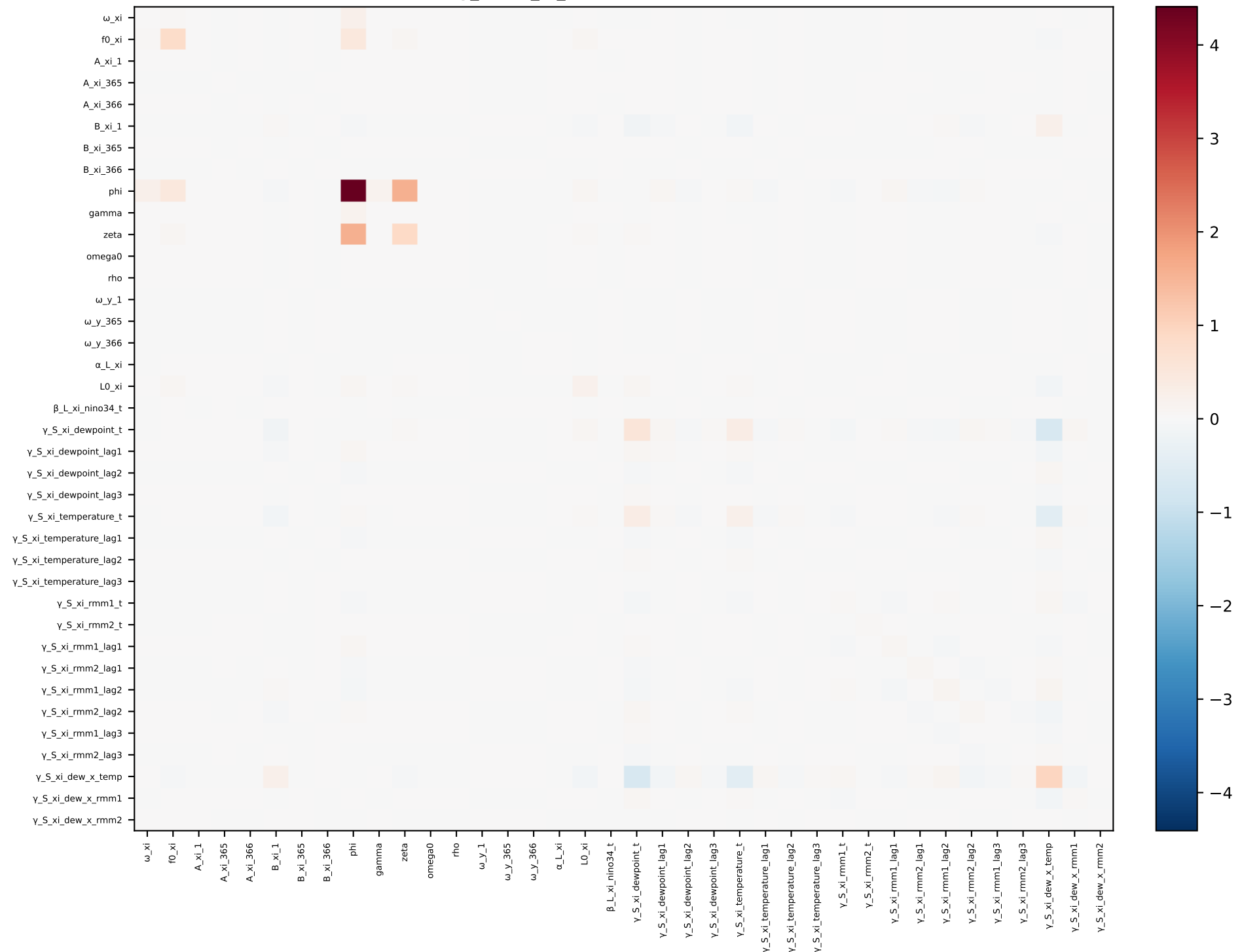
long_short_xi_interactions — covariance
