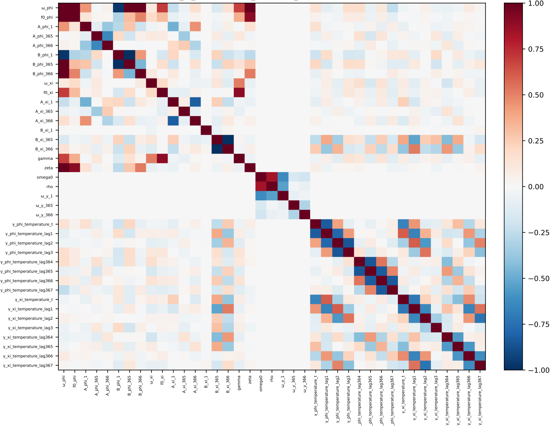
phi_xi_temperature_seasonal_lags — correlation
