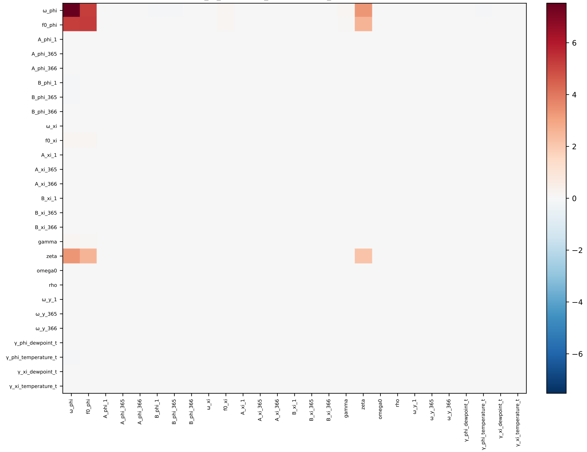
phi_xi_dewpoint_temperature_t — covariance
