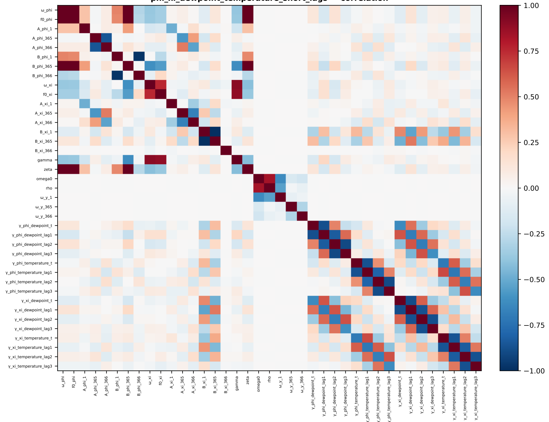
phi_xi_dewpoint_temperature_short_lags — correlation
