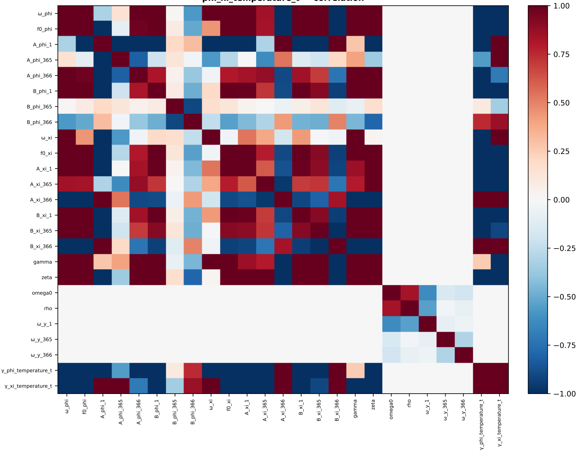
phi_xi_temperature_t — correlation
