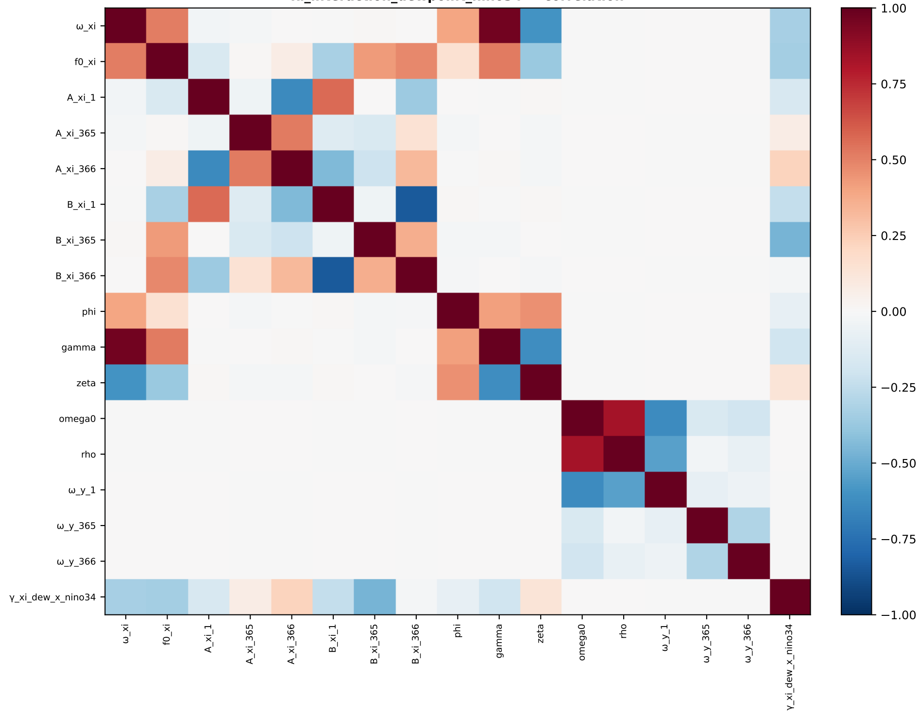
xi_interaction_dewpoint_nino34 — correlation
