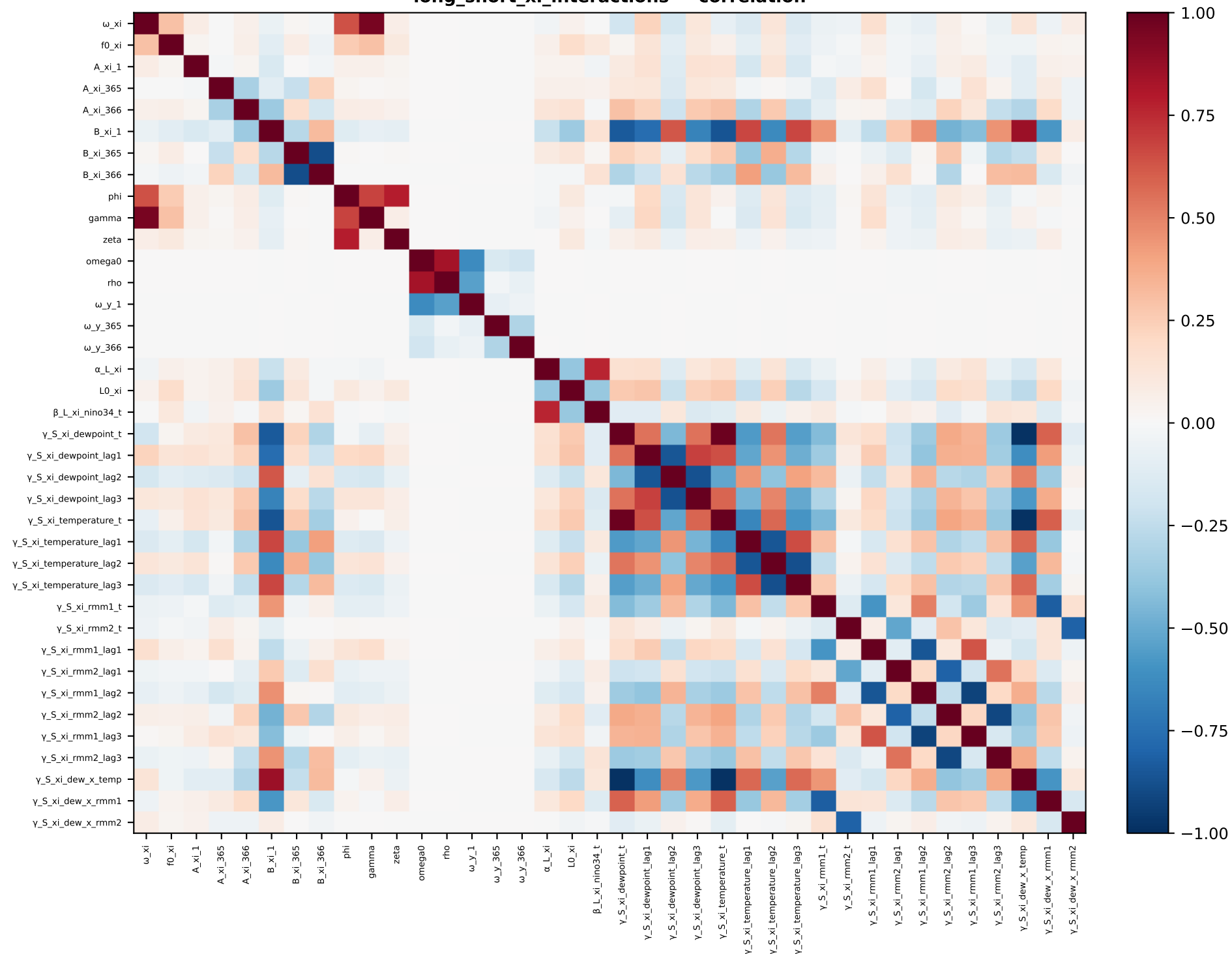
long_short_xi_interactions — correlation
