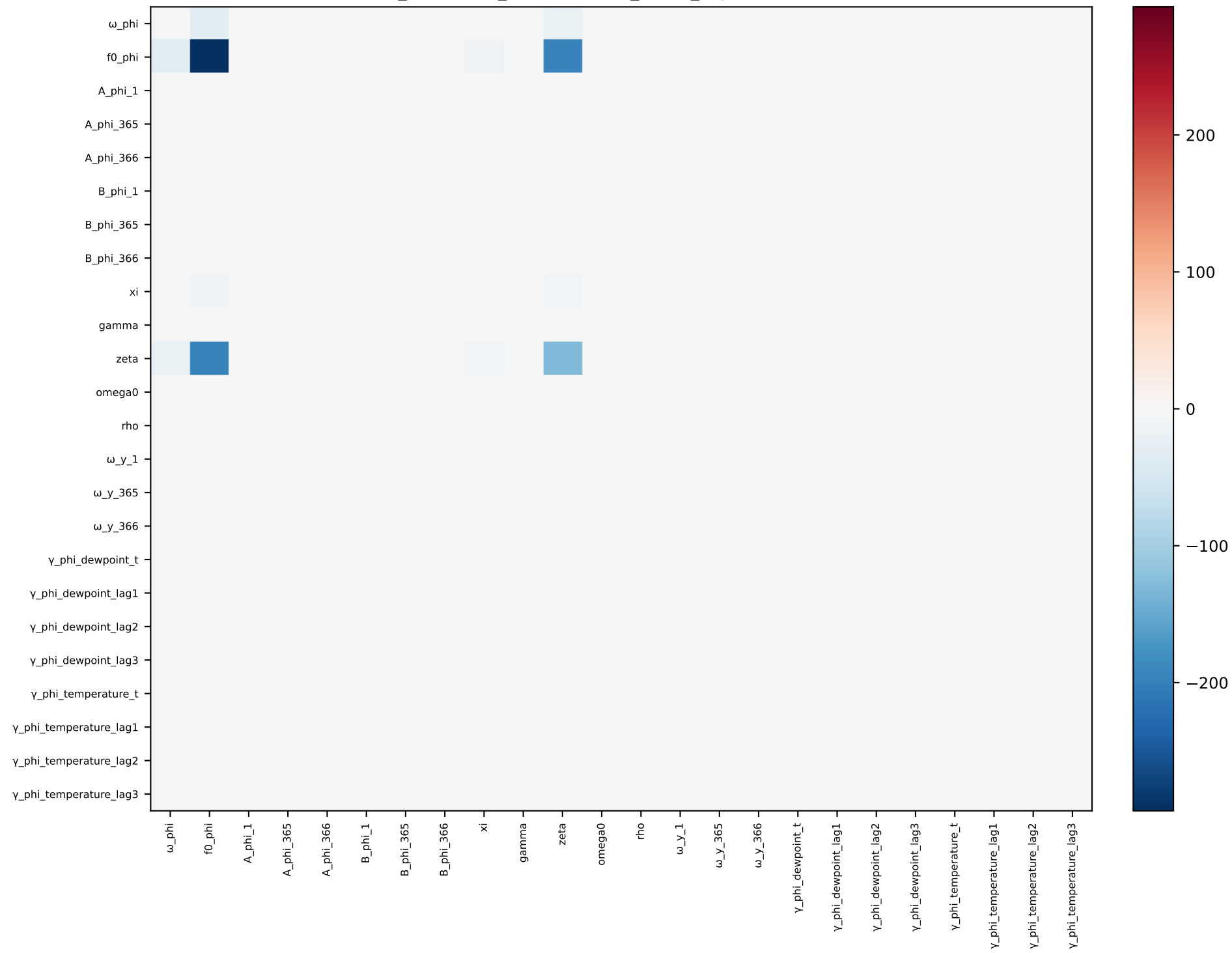
phi_dewpoint_temperature_short_lags – covariance
