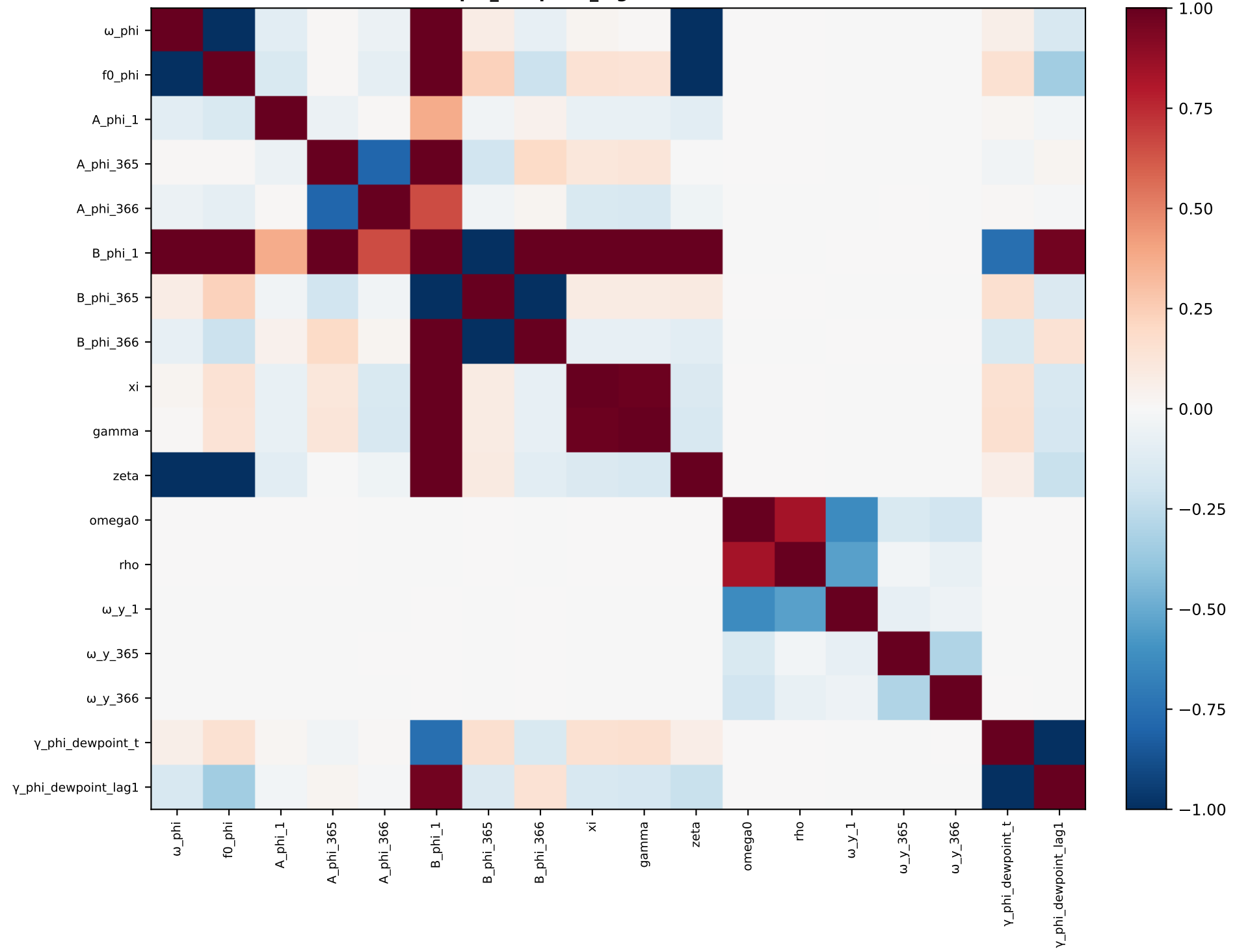
phi_dewpoint_lag1 — correlation
