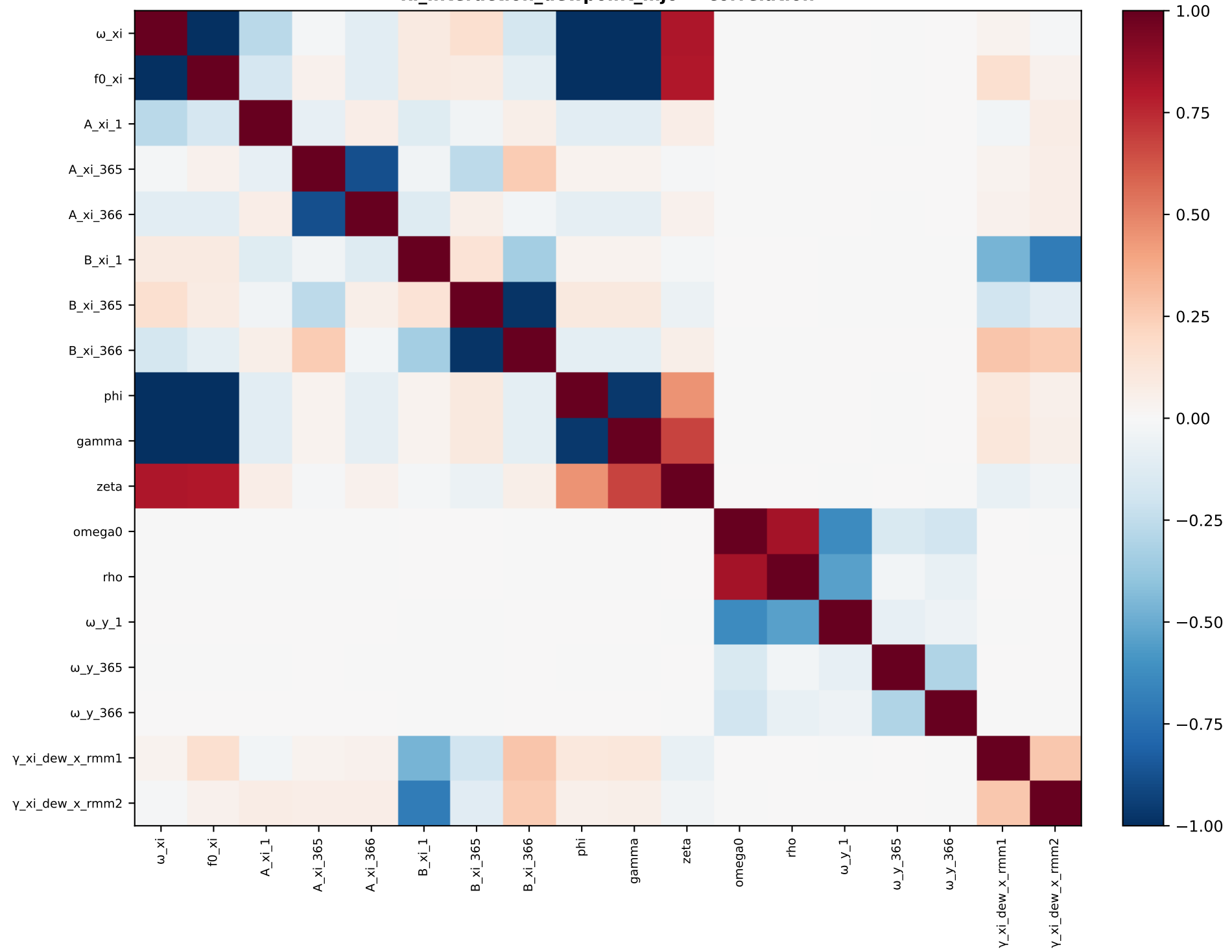
xi_interaction_dewpoint_mjo — correlation
