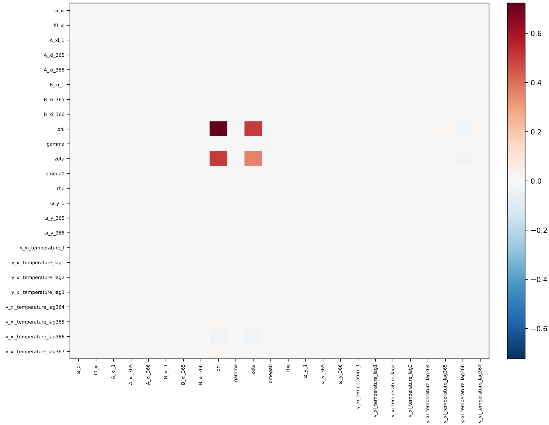
xi_temperature_seasonal_lags — covariance
