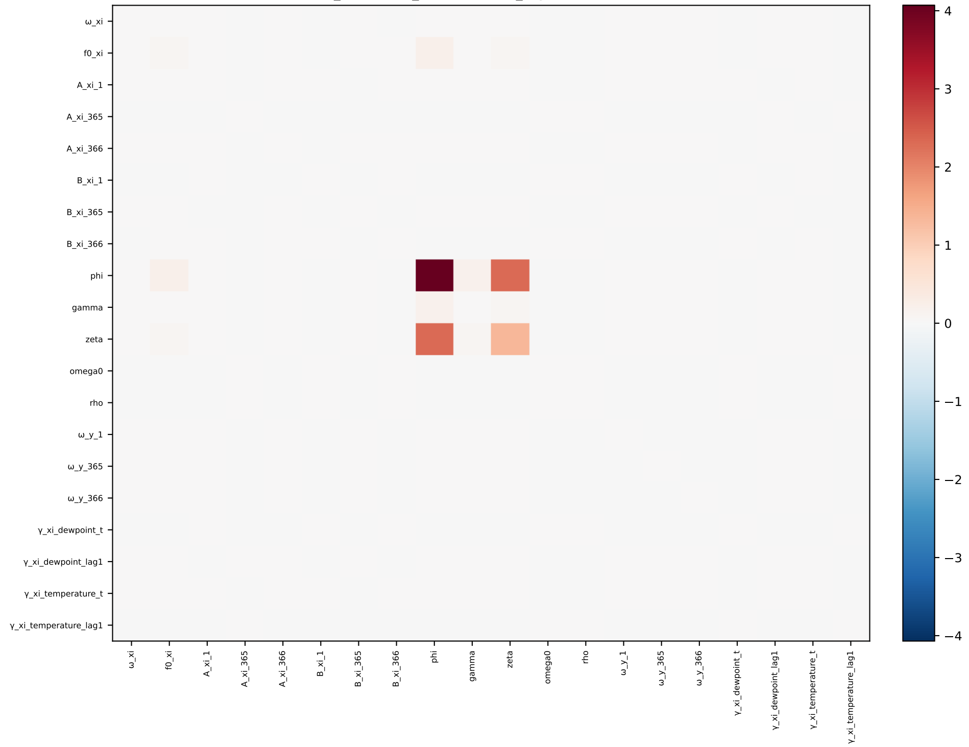
xi_dewpoint_temperature_lag1 — covariance
