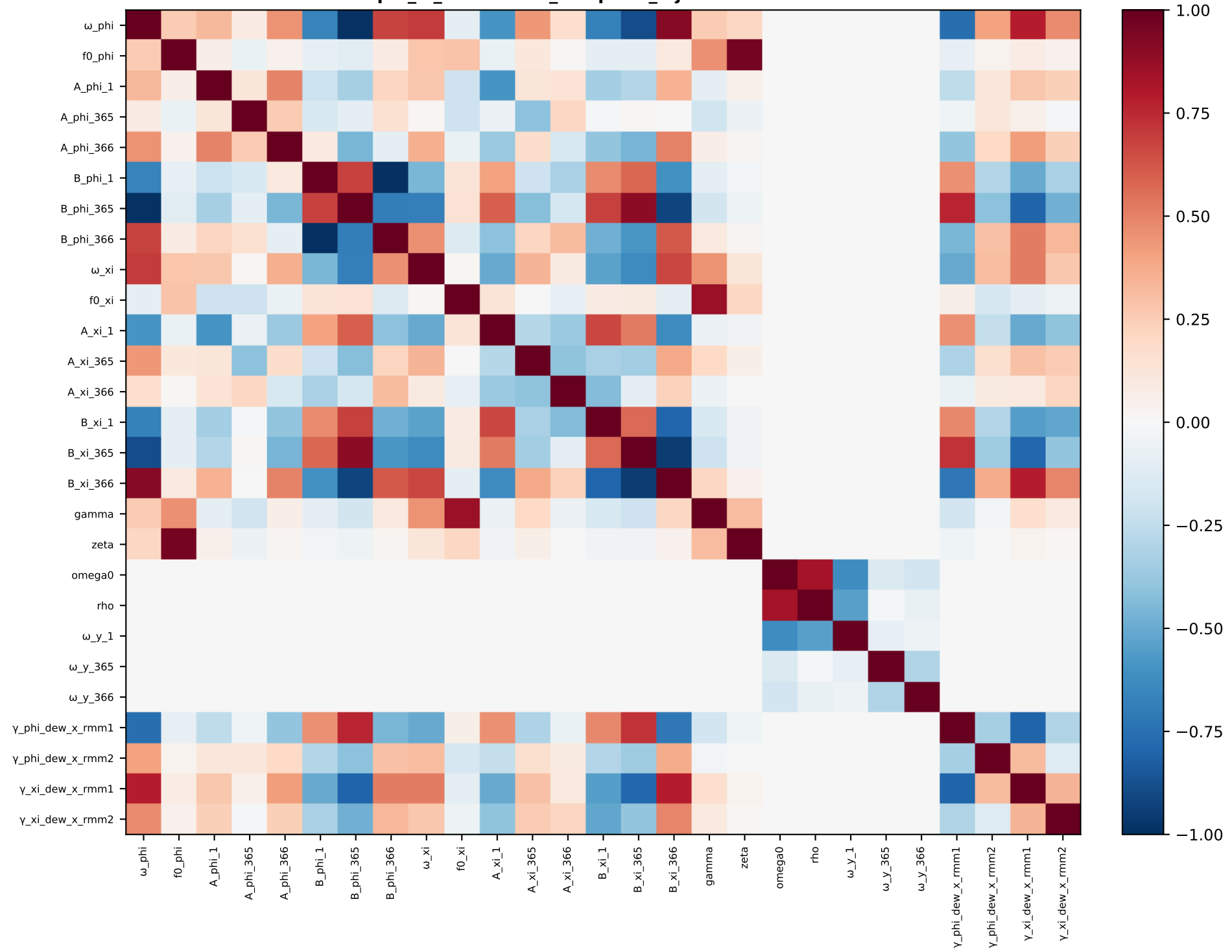
phi_xi_interaction_dewpoint_mjo — correlation
