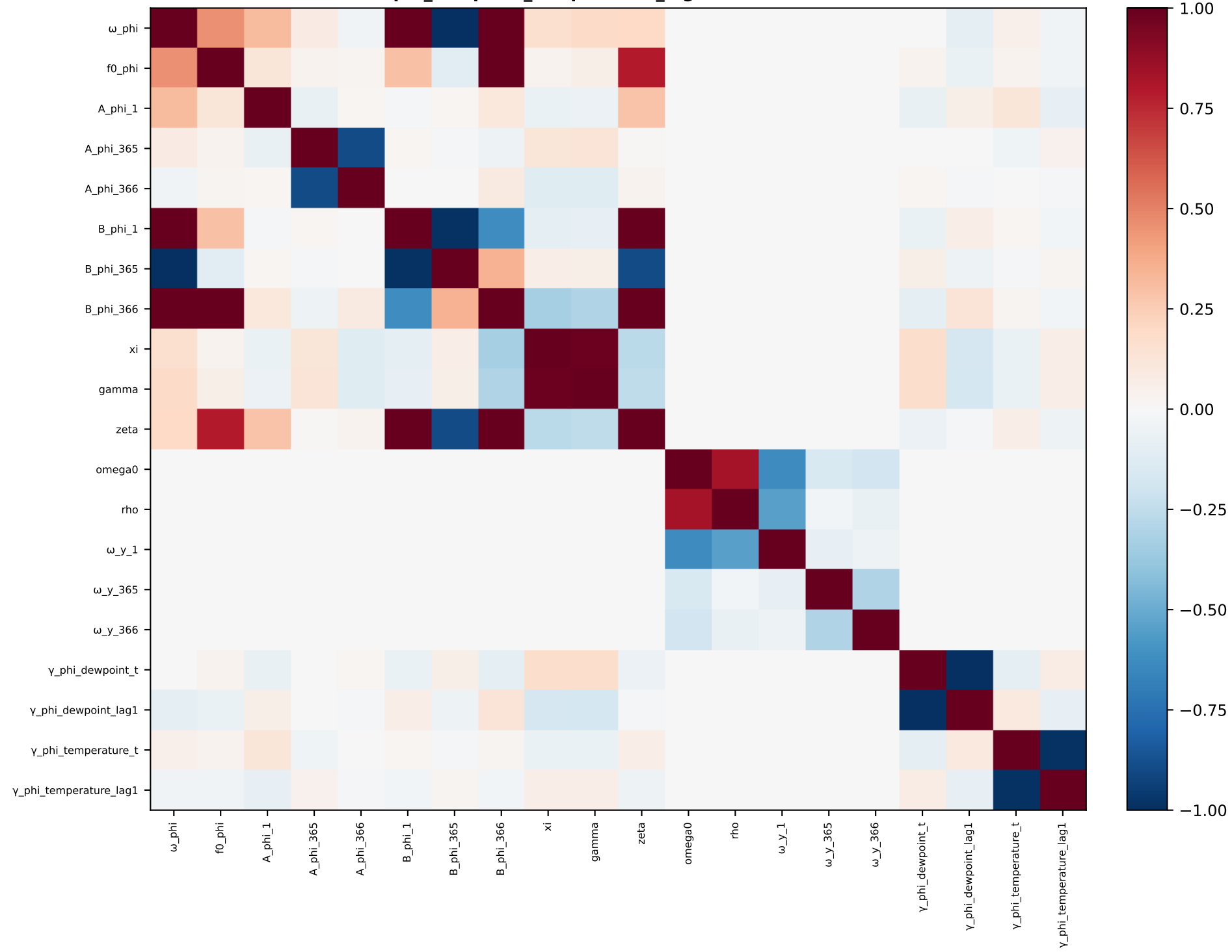
phi_dewpoint_temperature_lag1 — correlation
