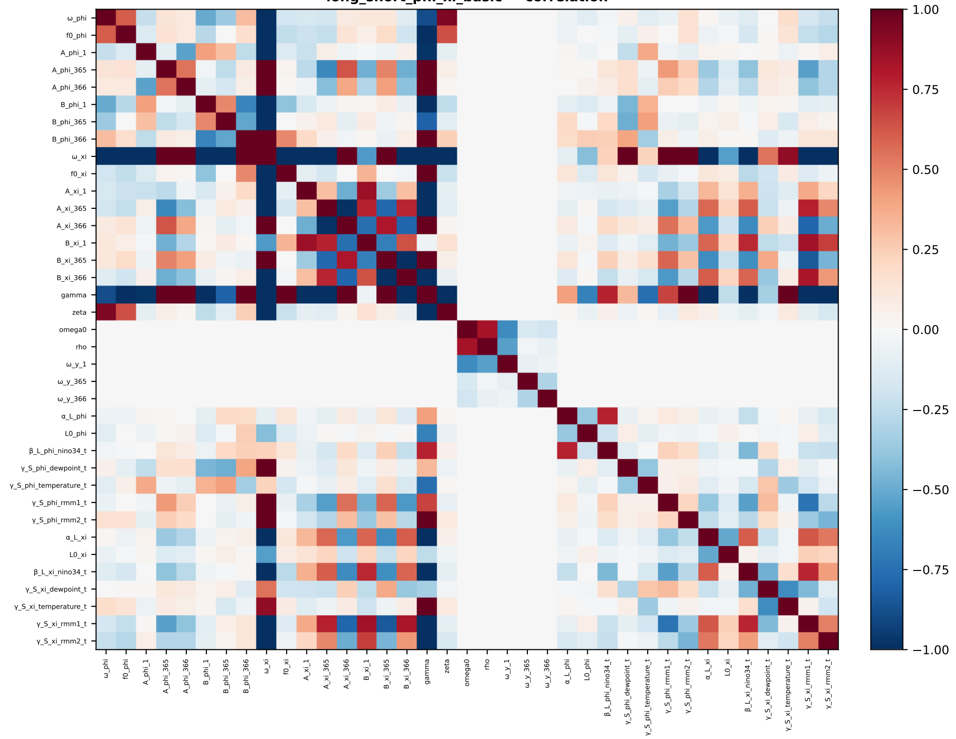
long_short_phi_xi_basic — correlation
