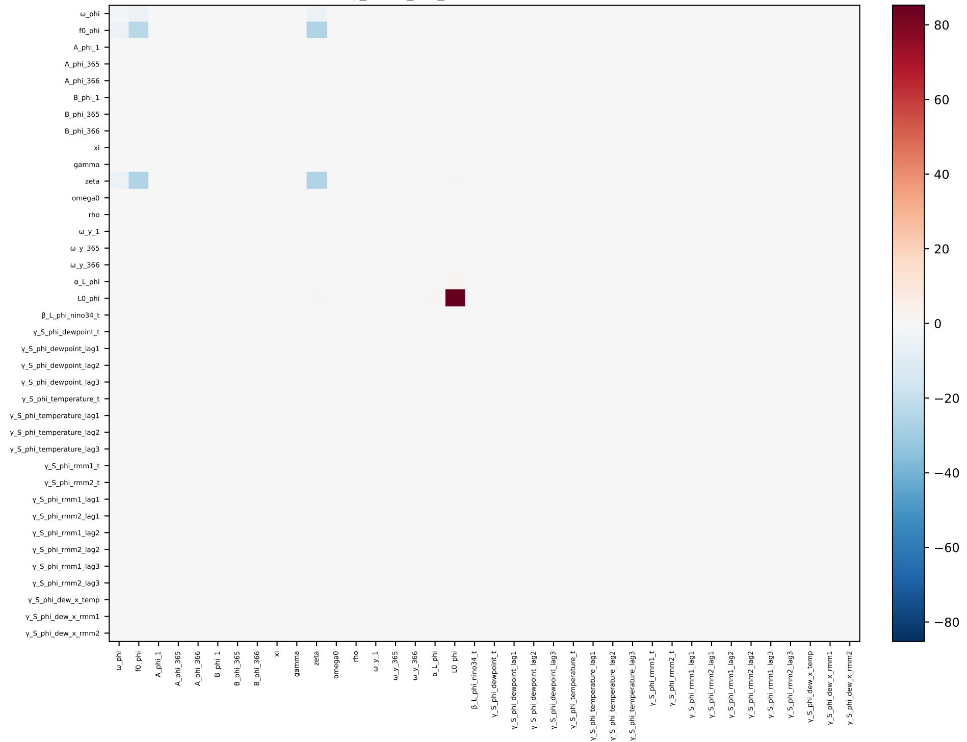
long_short_phi_interactions — covariance
