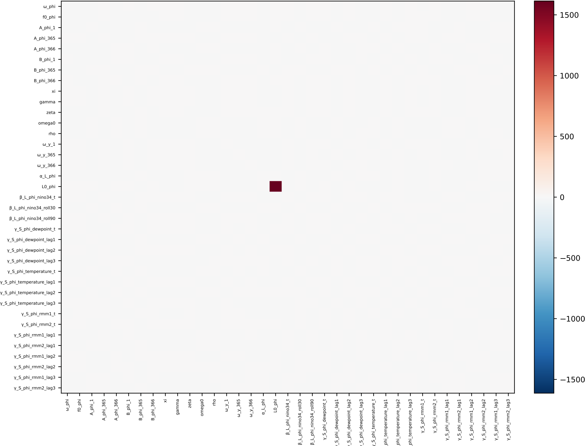
long_short_phi_weather_climate – covariance
