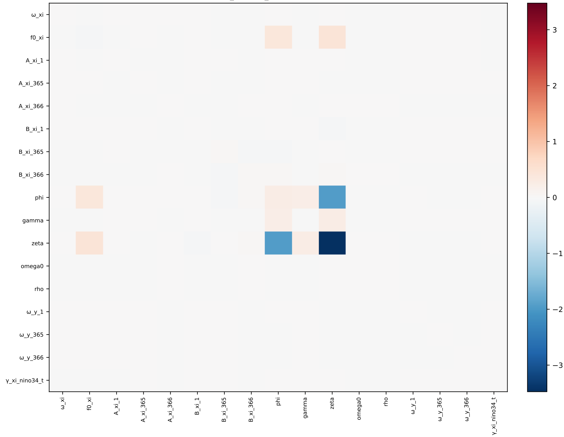
xi_nino34_t — covariance
