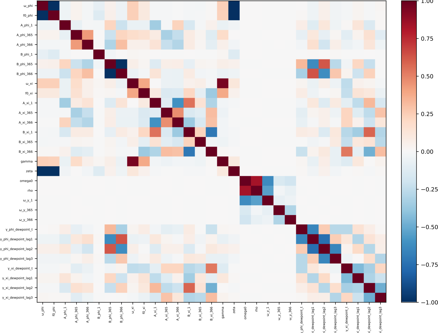
phi_xi_dewpoint_short_lags – correlation
