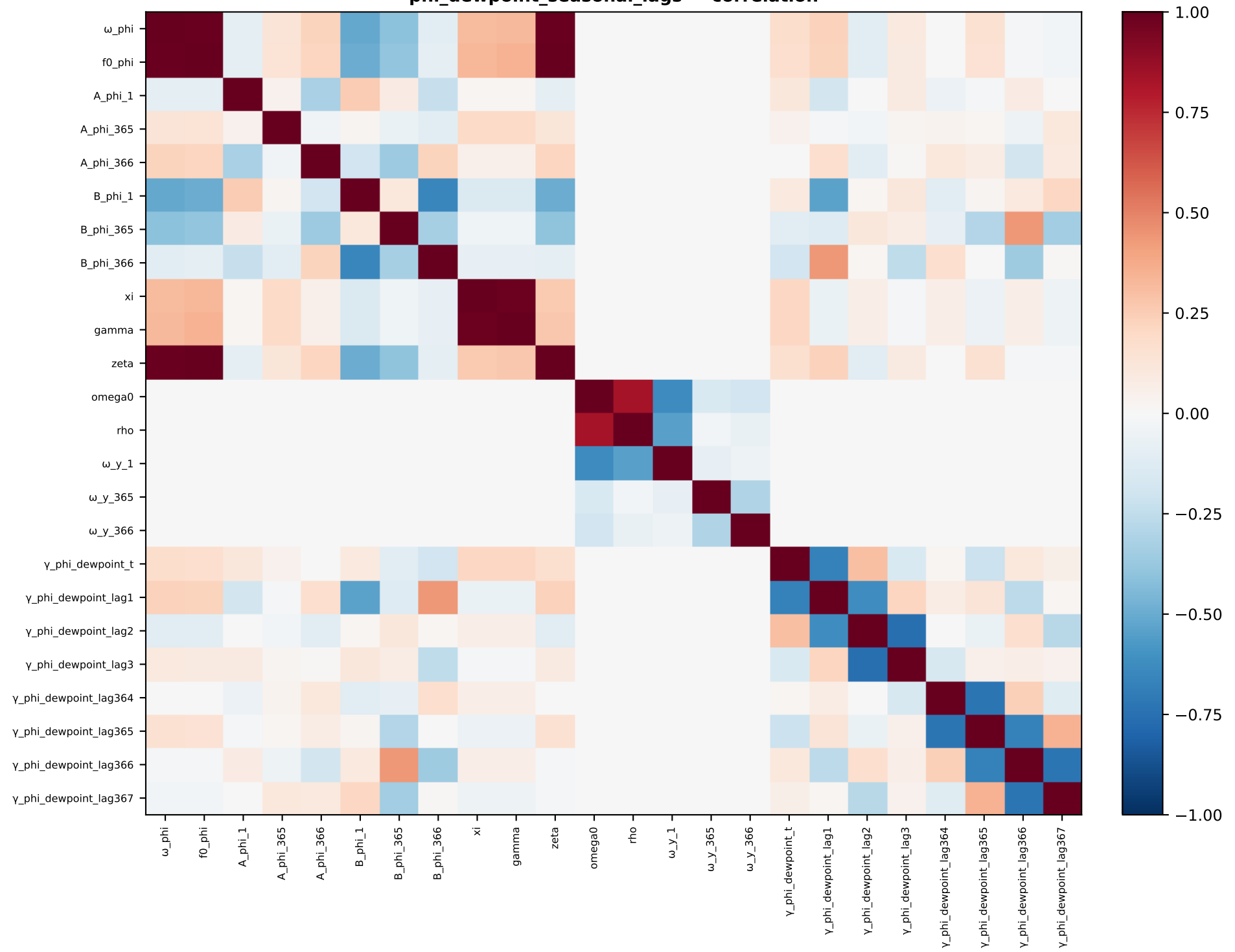
phi_dewpoint_seasonal_lags — correlation
