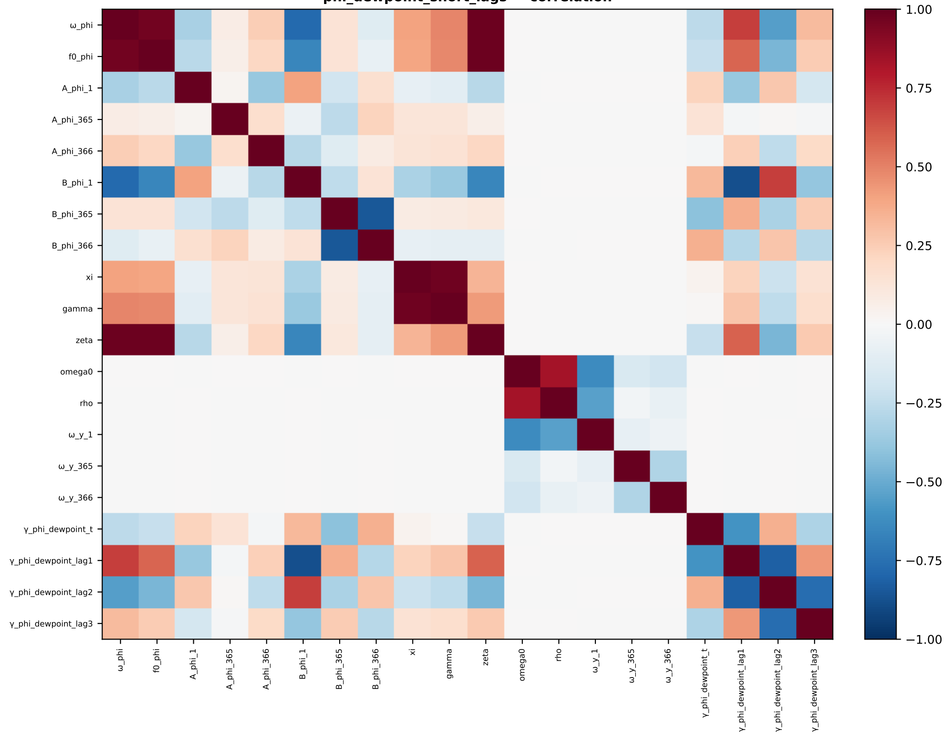
phi_dewpoint_short_lags — correlation
