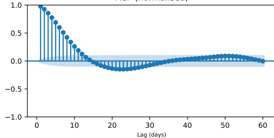
ACF (normalised)
