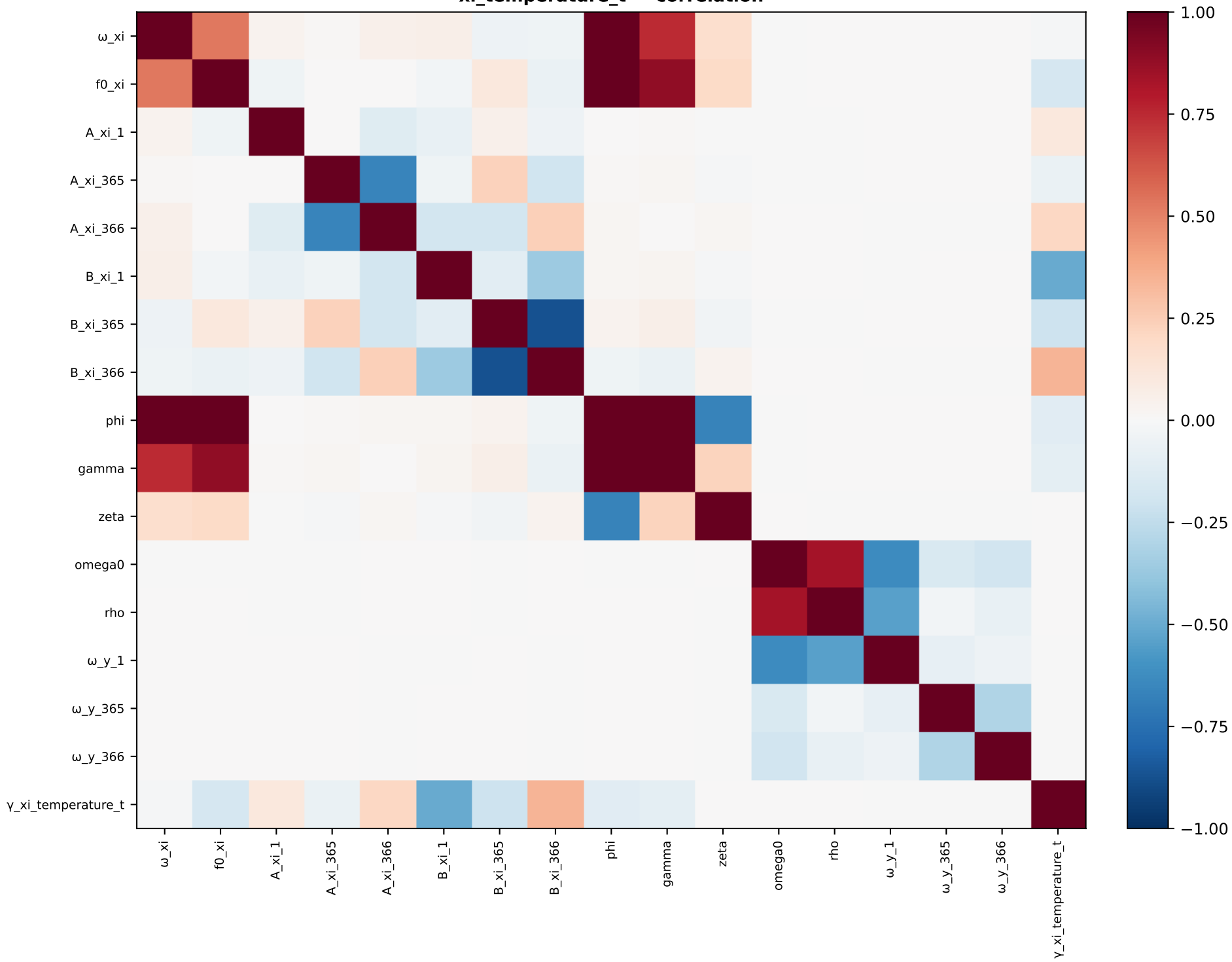
xi_temperature_t — correlation
