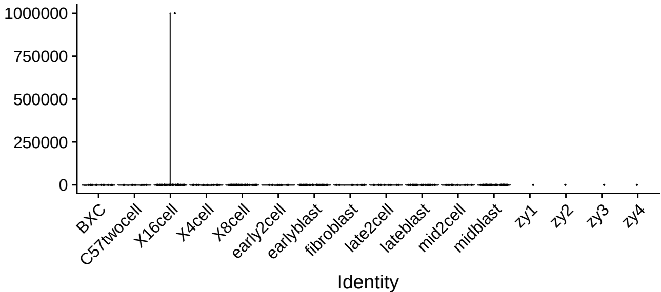
nCount_RNA
