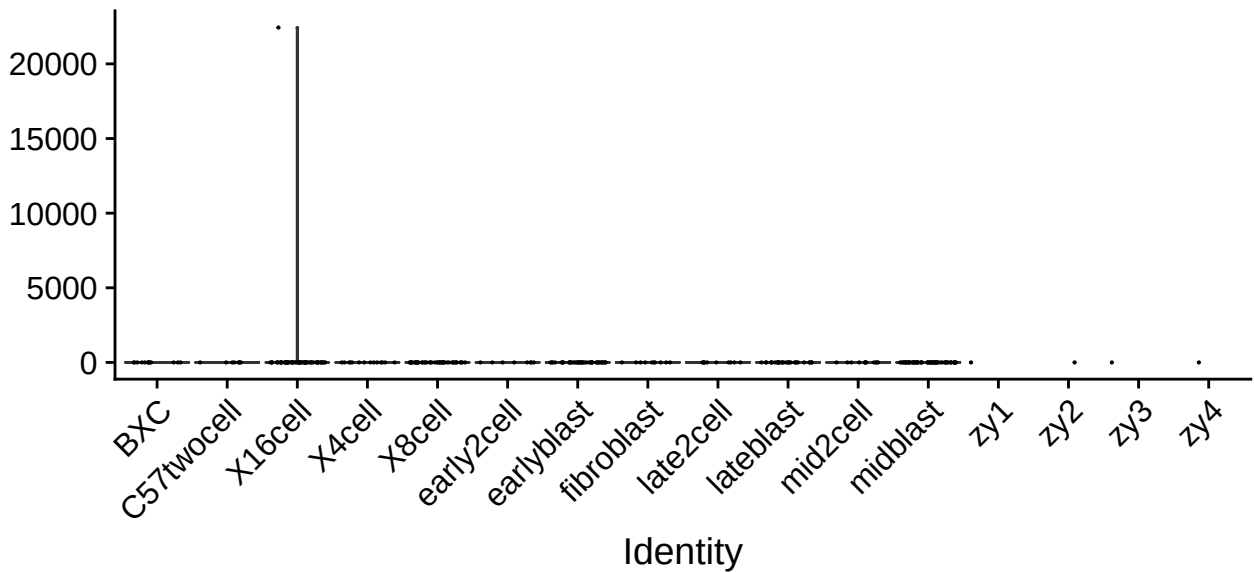
nCount_RNA
