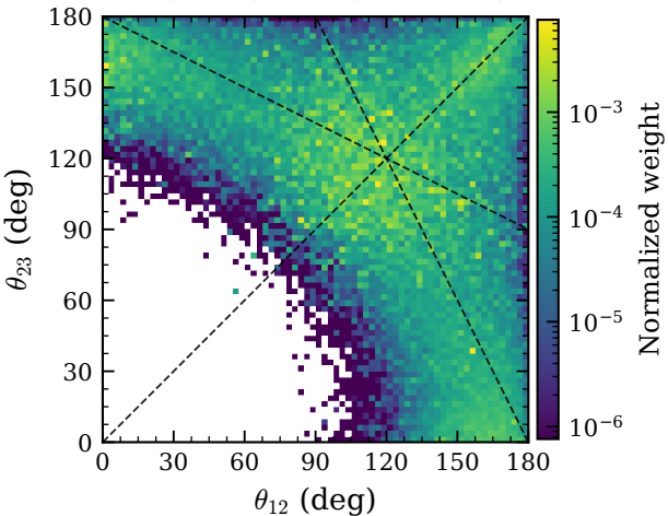
3N (no FSI) on ^{12}\text{C} ( N=14248105 )
