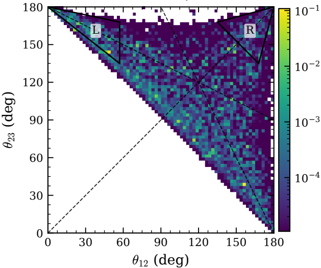
3N+FSI (OLD code) ( n_{>k_F}=2 , N=157770 )
