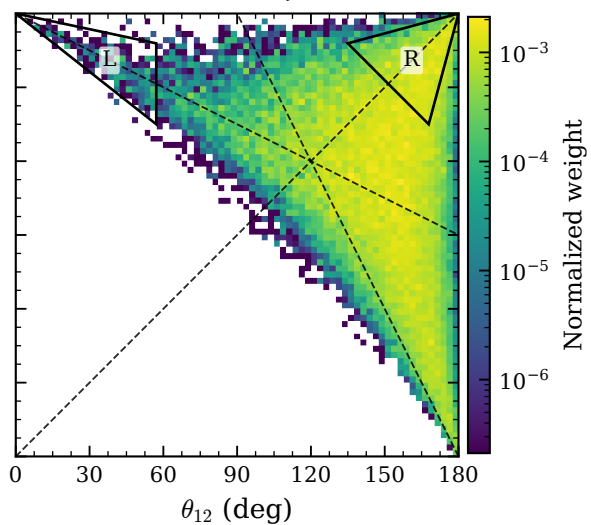
2N+FSI (OLD code) ( n_{>k_F}=2 , N=688540 )
