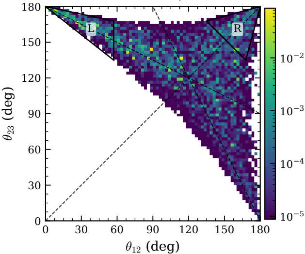
3N+FSI (OLD code) ( n_{>k_F}=2 , N=26733 )
