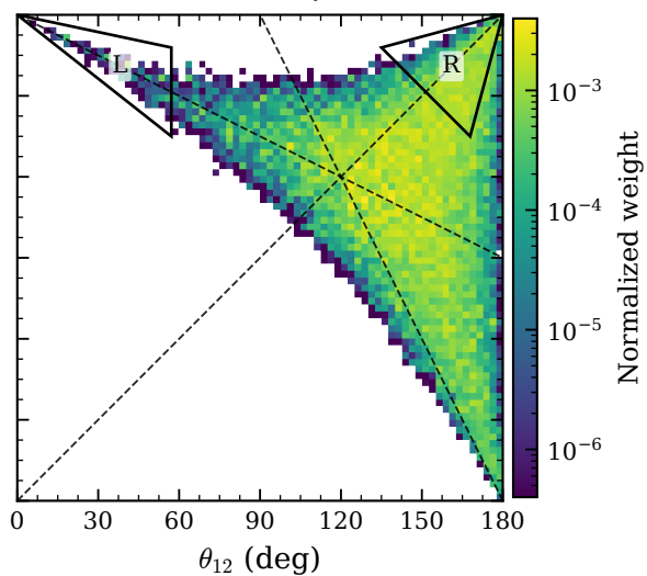
2N+FSI (OLD code) ( n_{>k_F}=2 , N=254248 )
