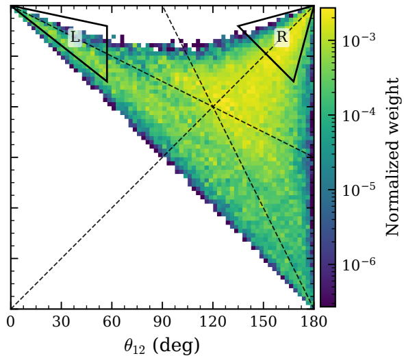
2N+FSI ( n_{>k_F}=2 , N=1043279 )
