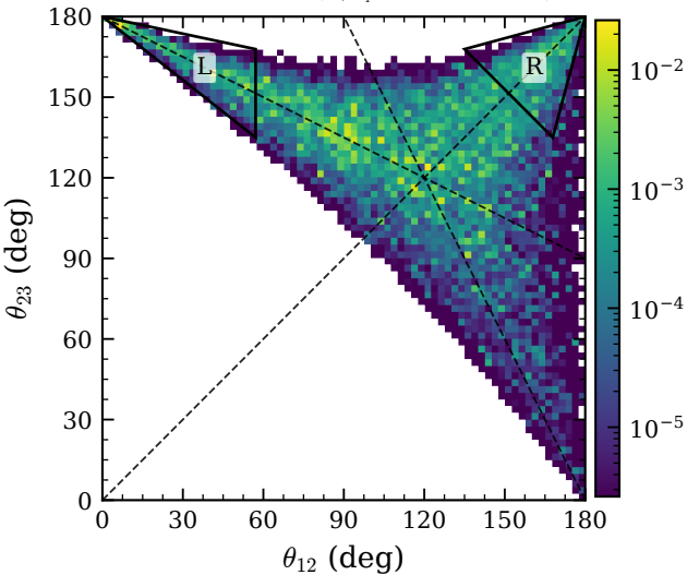
3N+FSI on ^{12}\text{C} ( n_{>k_F}=2 , N=309241 )
