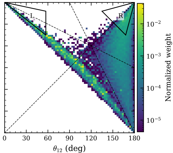
2N+FSI ( n_{>k_F}=2 , N=166695 )
