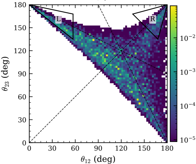
3N+FSI on ^{12}\text{C} ( n_{>k_F}=2 , N=129661 )
