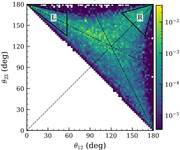
3N+FSI on ^{12}\text{C} ( n_{>k_F}=2 , N=2396586 )
