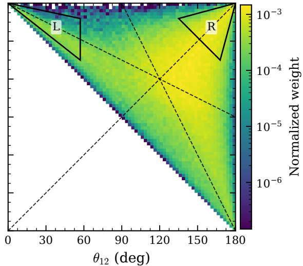
2N+FSI ( n_{>k_F}=2 , N=8480045 )
