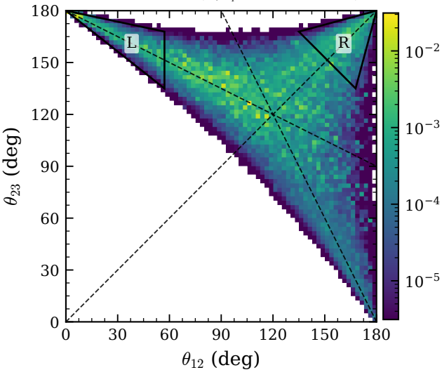
3N+FSI on ^{12}\text{C} ( n_{>k_F}=2 , N=1051615 )
