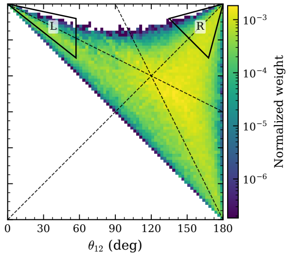
2N+FSI ( n_{>k_F}=2 , N=3590743 )
