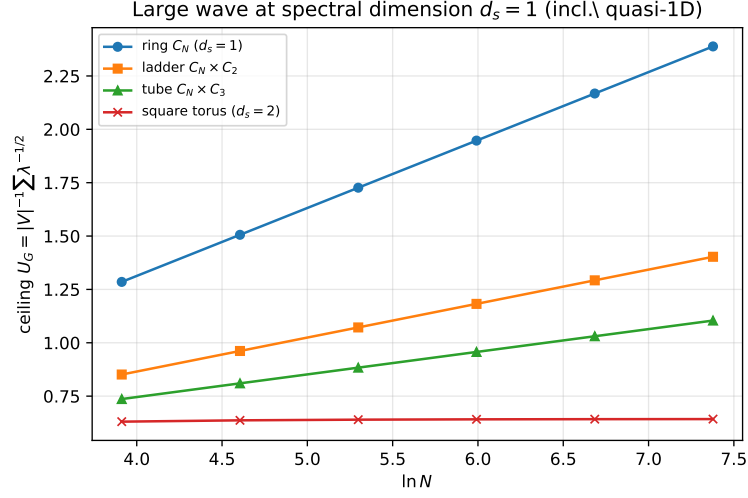
FIGURE 13. Spectral-dimension threshold. The ceiling U_G = |V|^{-1} \sum \lambda^{-1/2} grows like \ln N for d_s = 1 —the ring and, with reduced slope 1/(\pi w) , the quasi-1D ladder and tube—but saturates for the d_s = 2 square torus. The ceiling is a critical-dimension ( d_s = 1 ) phenomenon.
