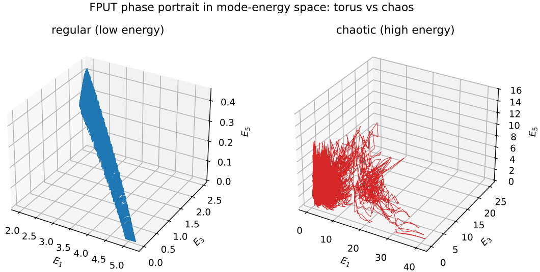
FIGURE 21. FPUT phase portrait in the odd-mode energy space (E_1, E_3, E_5) . Left: at low energy the orbit lies on a thin quasi-periodic torus (regular). Right: at high energy it fills a three-dimensional chaotic cloud—the same regular-to-chaotic transition measured by \lambda_{\max} .
