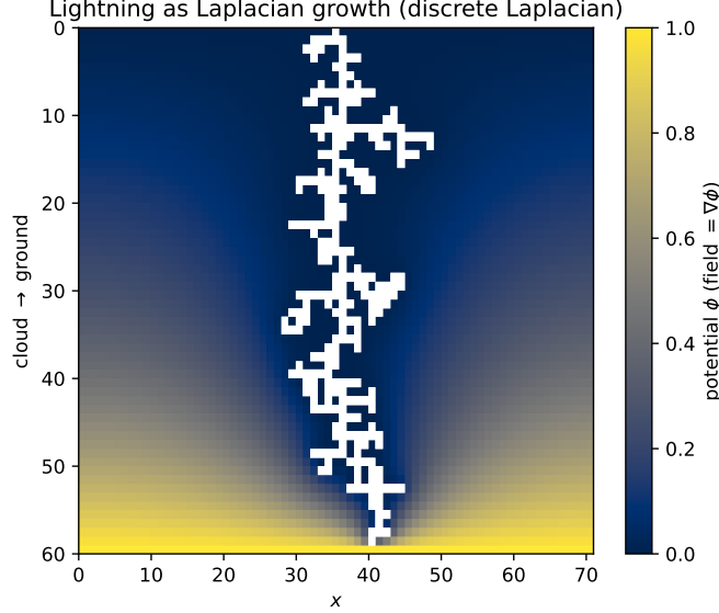
FIGURE 29. Lightning as Laplacian growth: the leader (white) advances cloud-to-ground where the field is strongest, the potential \phi solving the discrete Laplace equation L_N^{(2)}\phi = 0 off it. A branched fractal discharge with the energy concentrated at its tips—energy concentration on the same discrete Laplacian, electrostatically.
