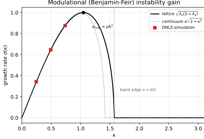
FIGURE 16. Modulational (Benjamin-Feir) instability gain (27) of the plane wave under the DNLS (24): lattice rate (solid), continuum approximation (dotted) and simulated growth rates (squares), with unstable band edge \kappa = \pi/2 and maximal rate \sigma_{\max} = \gamma A^2 .
