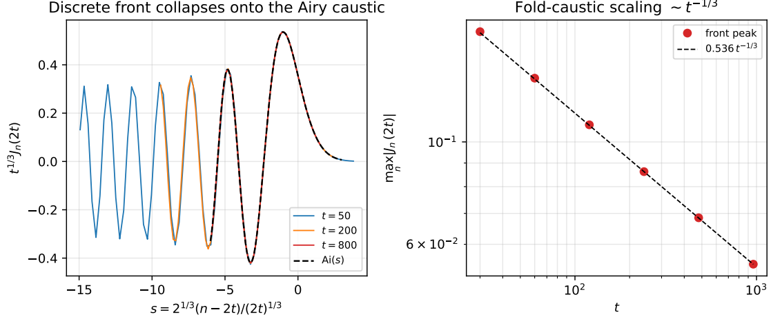
FIGURE 27. The discrete-Schrödinger front as a fold caustic. Left: the rescaled fronts t^{1/3} J_n(2t) for t = 50, 200, 800 collapse onto the Airy function \text{Ai}(s) , s = 2^{1/3}(n - 2t)/(2t)^{1/3} (Eq. (30)). Right: the front peak follows the universal fold scaling 0.536 t^{-1/3} .
