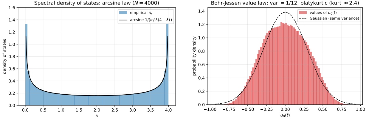
FIGURE 12. Left: spectral density of states converges to the arcsine law (22). Right: the Bohr–Jessen value law of u_0(t) —symmetric, variance (N^2 - 1)/(12N^2) \rightarrow 1/12 , platykurtic (flatter than the Gaussian of equal variance, dashed).
