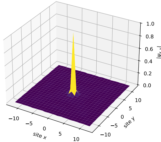
FIGURE 22. Two-dimensional discrete breather: a single-site seed under the 2D DNLS self-traps into a persistent localized hump above the 2D band top ( \gamma \approx 8 ). Nonlinearity restores a large localized amplitude in 2D, where the linear large wave is bounded.
