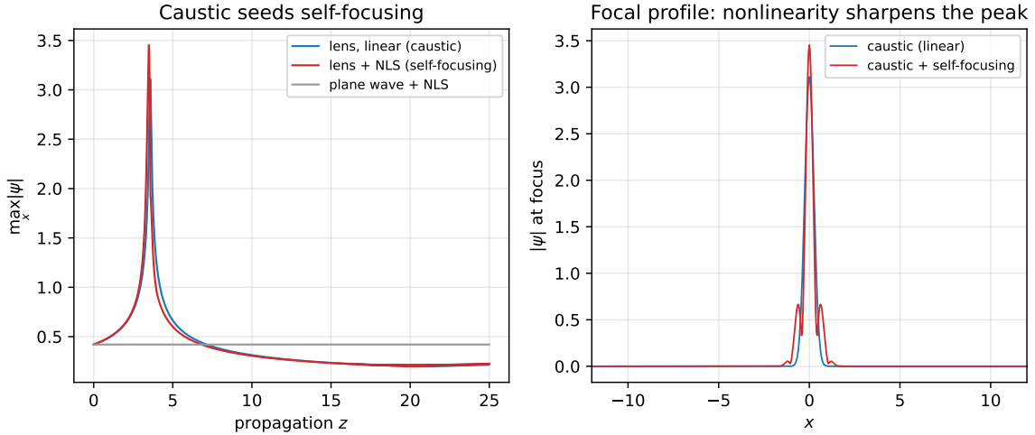
FIGURE 26. A linear caustic seeds nonlinear self-focusing (focusing NLS, lens-seeded beam). Left: the peak amplitude—the lens focuses a weak flat input \sim 7\times (caustic), the nonlinearity adds a further \sim 11\% , while the lensless plane wave stays flat. Right: at the focus the nonlinearity sharpens and heightens the peak.
