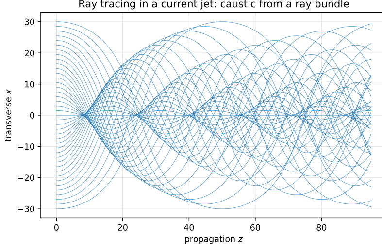
FIGURE 24. Ray tracing in a current jet. A bundle of parallel rays is refracted toward the jet, crosses on a caustic (the fold near z \approx 8 , then re-focusing), where the ray density and the linear amplitude concentrate.
