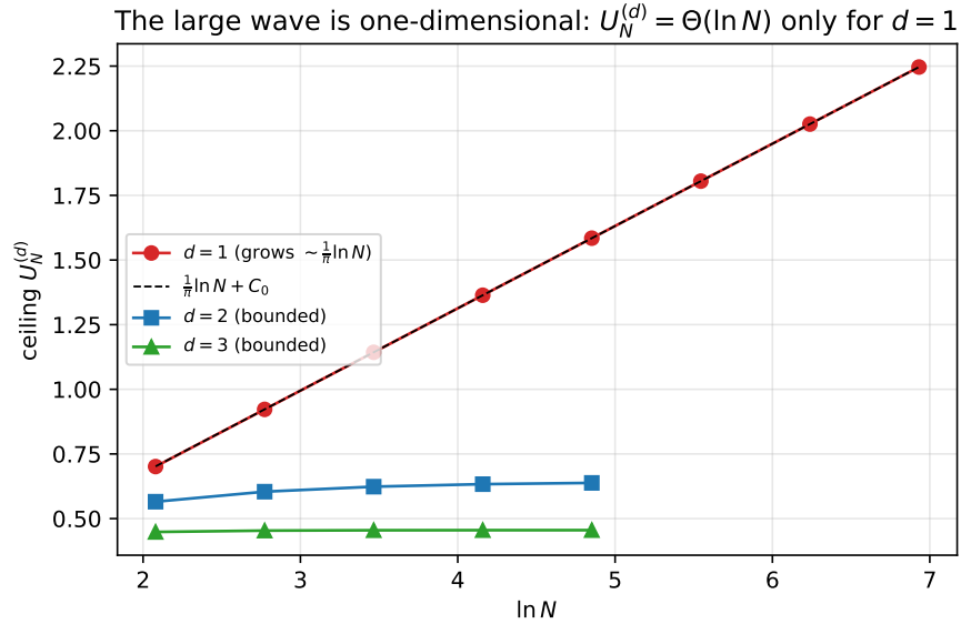
FIGURE 14. Ceilings U_N^{(d)} versus \ln N . Only d = 1 grows (slope 1/\pi , on the dashed \frac{1}{\pi} \ln N + C_0 ); the 2- and 3-torus ceilings saturate, so A_N^{(d)} = O(1) for d \geq 2 .
