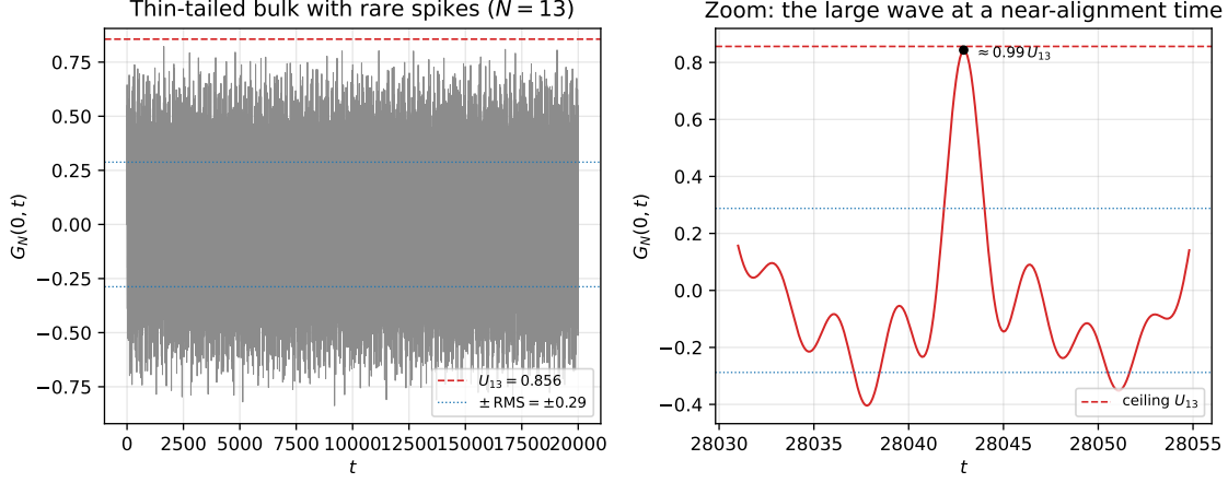
FIGURE 11. What the large wave looks like in time ( N = 13 , prime). Left: the node-0 response G_N(0, t) oscillates within the thin band \pm \text{RMS} ( \text{RMS} \approx 0.29 ) but throws rare spikes toward the ceiling U_{13} = 0.856 . Right: a zoom on the largest near-alignment spike, reaching \approx 0.99 U_N —the large wave forming as the modal phases briefly align ( verify_thesis_peaks.py ).
