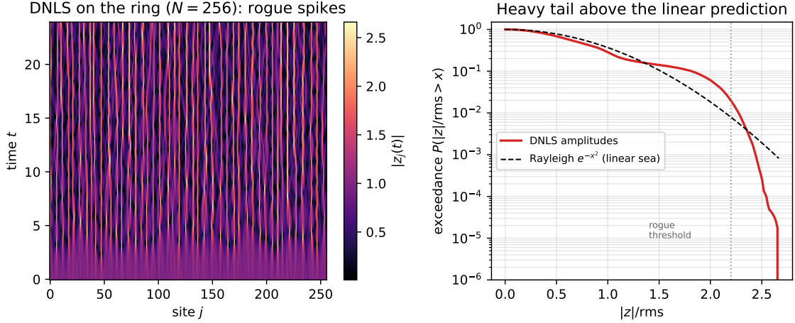
FIGURE 17. DNLS (24) on the ring seeded by a noisy plane wave. Left: space-time amplitude |z_j(t)| with localized rogue spikes. Right: the amplitude exceedance distribution develops a heavy tail above the Rayleigh law (dashed) of a linear Gaussian sea, crossing the rogue threshold—the opposite of the platykurtic linear value law.
