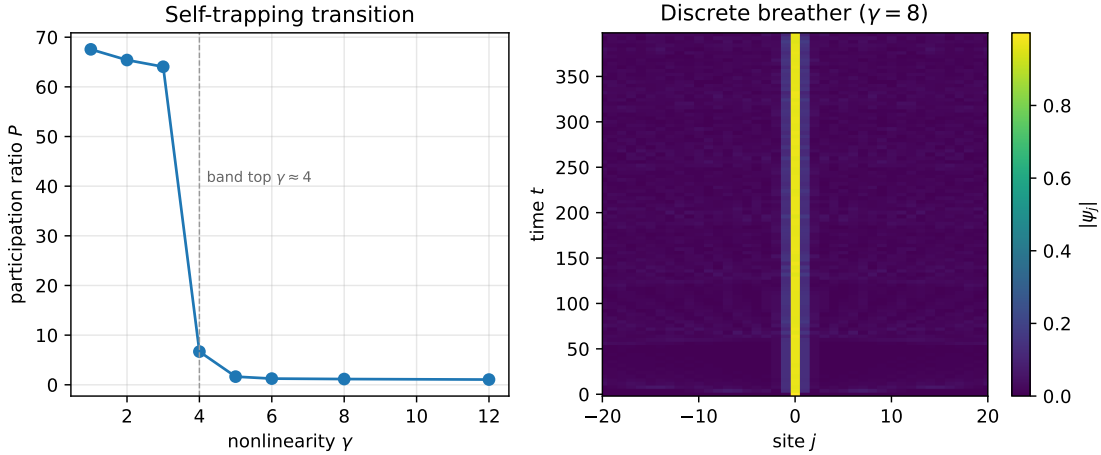
FIGURE 18. DNLS self-trapping ( N = 128 , single-site seed). Left: the participation ratio P collapses from \sim N (dispersed) to \sim 1 (trapped) as the nonlinearity crosses the band top \gamma \approx 4 . Right: above threshold the excitation is a persistent localized breather-like state—a localized column in space-time.
