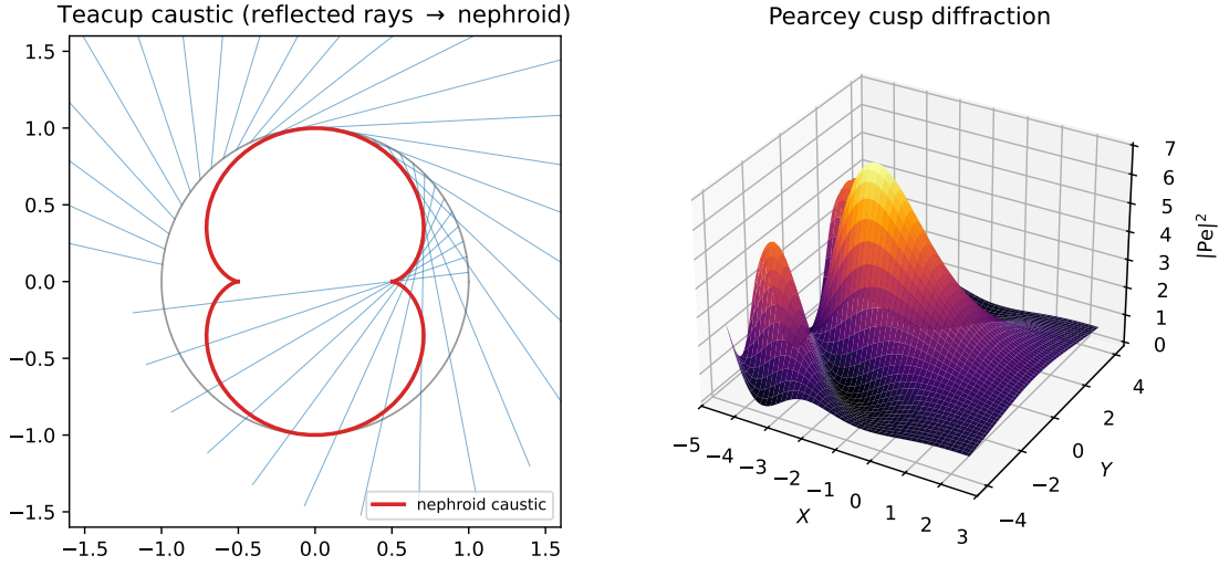
FIGURE 25. The cusp caustic. Left: the everyday teacup caustic—parallel rays reflected inside a circle have a nephroid envelope. Right: the universal Pearcey diffraction |\text{Pe}(X, Y)|^2 of the cusp, bright inside the cusp and dark in the shadow.
