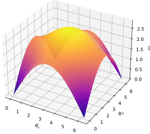
FIGURE 23. Dispersion surface \omega(\theta_x, \theta_y) = 2\sqrt{\sin^2(\theta_x/2) + \sin^2(\theta_y/2)} of the block-circulant Laplacian on the 2-torus: zero at the corners, band top 2\sqrt{2} at the centre.
