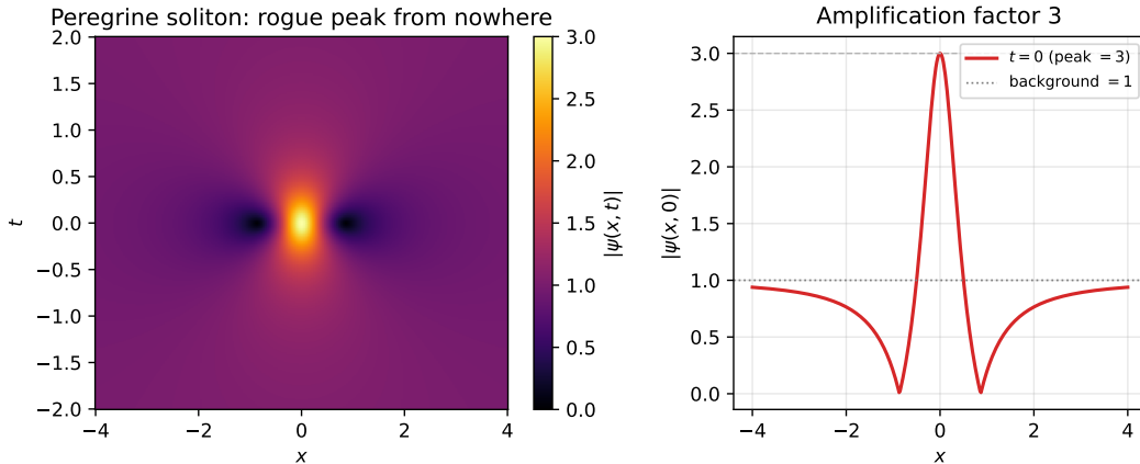
FIGURE 15. Peregrine soliton (26) of the focusing NLS (25): a rogue peak localized in space and time (left), with the threefold amplification over the unit background at t = 0 (right).
