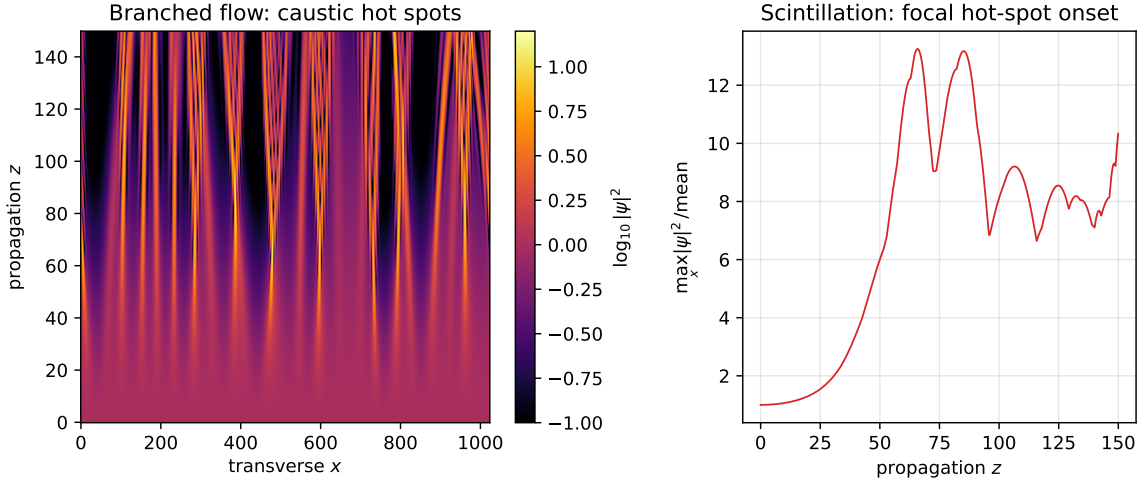
FIGURE 28. Branched flow of a wave in a weak random current (paraxial model). Left: a uniform incident wave ( z = 0 ) develops bright caustic filaments and focal hot spots as it propagates. Right: the scintillation index rises from 1 to \sim 13 at the first focal distance—the linear, refractive route to a rogue hot spot.
