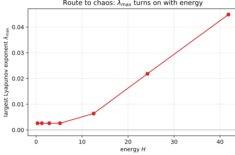
FIGURE 20. Route to chaos. The maximal Lyapunov exponent of the FPUT- \beta ring is \approx 0 at low energy (regular, the recurrence regime) and turns on past an energy threshold, reaching \lambda_{\max} \approx 0.05 in the chaotic regime.
