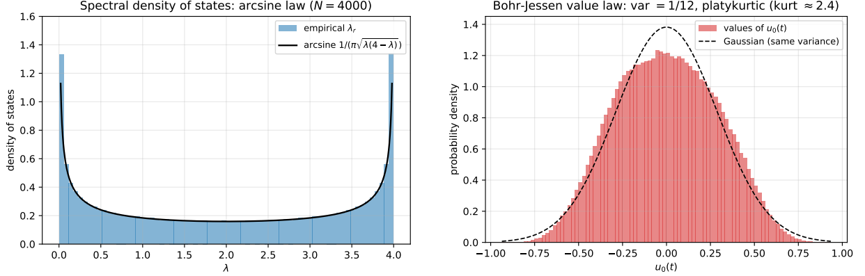
FIGURE 12. Left: spectral density of states converges to the arcsine law (22). Right: the Bohr–Jessen value law of u_0(t) —symmetric, variance (N^2 - 1)/(12N^2) \rightarrow 1/12 , platykurtic (flatter than the Gaussian of equal variance, dashed).
