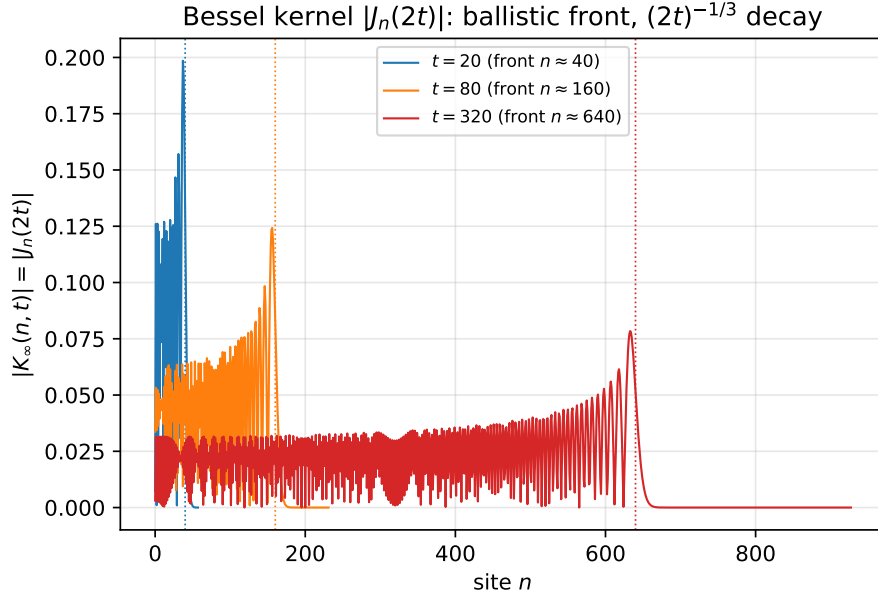
FIGURE 6. Infinite-chain Schrödinger kernel |K_\infty(n, t)| = |J_n(2t)| : a ballistic front at n \approx 2t (dotted) whose height decays as (2t)^{-1/3} . On the ring this kernel is periodized, (15); the effect is intrinsically finite-size.
