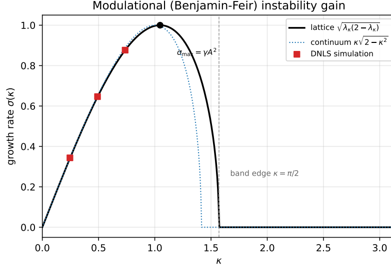
FIGURE 17. Modulational (Benjamin-Feir) instability gain (27) of the plane wave under the DNLS (24): lattice rate (solid), continuum approximation (dotted) and simulated growth rates (squares), with unstable band edge \kappa = \pi/2 and maximal rate \sigma_{\max} = \gamma A^2 .
