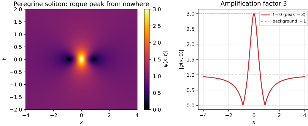
FIGURE 16. Peregrine soliton (26) of the focusing NLS (25): a rogue peak localized in space and time (left), with the threefold amplification over the unit background at t = 0 (right).
