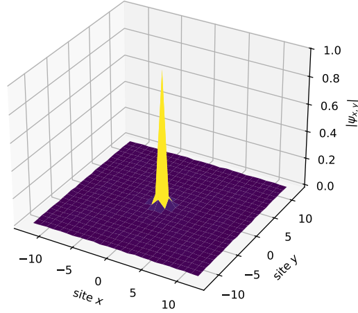
FIGURE 23. Two-dimensional discrete breather: a single-site seed under the 2D DNLS self-traps into a persistent localized hump above the 2D band top ( \gamma \approx 8 ). Nonlinearity restores a large localized amplitude in 2D, where the linear large wave is bounded.
