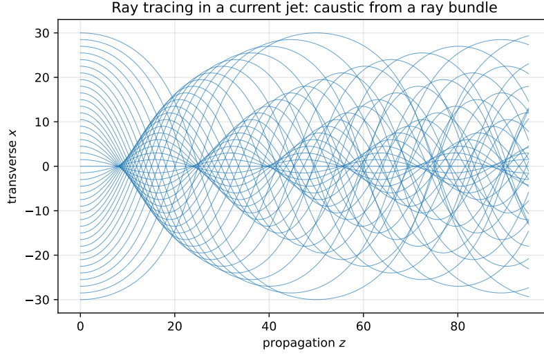
FIGURE 25. Ray tracing in a current jet. A bundle of parallel rays is refracted toward the jet, crosses on a caustic (the fold near z \approx 8 , then re-focusing), where the ray density and the linear amplitude concentrate.
