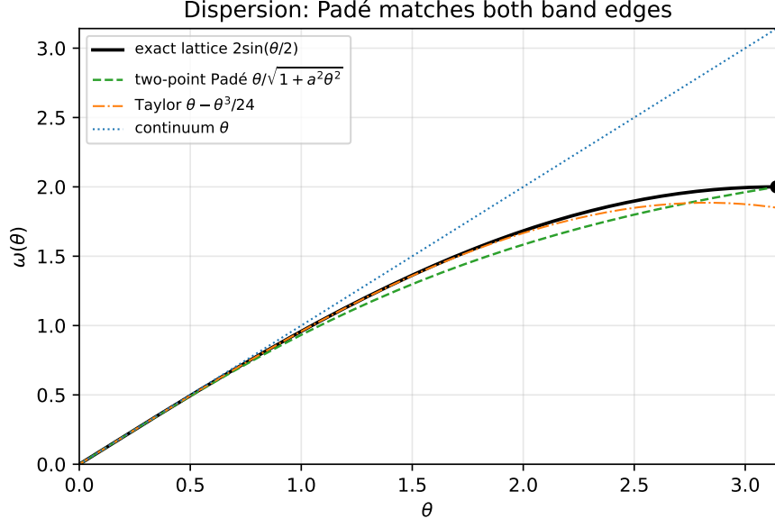
FIGURE 9. Dispersion relations. The exact lattice branch 2\sin(\theta/2) is matched at both ends by the two-point Padé (21), whereas the continuum \theta and the Taylor truncation \theta - \theta^3/24 diverge at the band edge \theta = \pi ( \bullet , \omega = 2 ).
