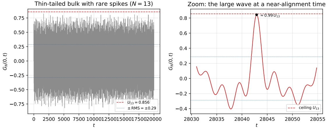
FIGURE 12. What the large wave looks like in time ( N = 13 , prime). Left: the node-0 response G_N(0, t) oscillates within the thin band \pm \text{RMS} ( \text{RMS} \approx 0.29 ) but throws rare spikes toward the ceiling U_{13} = 0.856 . Right: a zoom on the largest near-alignment spike, reaching \approx 0.99 U_N —the large wave forming as the modal phases briefly align ( verify_thesis_peaks.py ).
