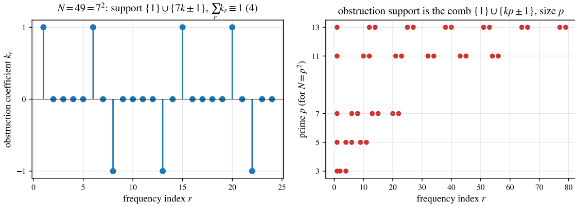
FIGURE 11. The composite obstruction for N = p^2 (Observation 24, exact/gap/prime_square.g). Left: the GAP-computed minimal mod-4 obstruction at N = 49 ( p = 7 )—coefficients \pm 1 on the comb \{1, 6, 8, 13, 15, 20, 22\} = \{1\} \cup \{7k \pm 1\} . Right: the support comb \{1\} \cup \{kp \pm 1\} for p = 3, 5, 7, 11, 13 , of size p .
