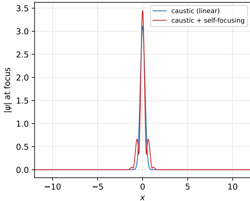
Focal profile: nonlinearity sharpens the peak
