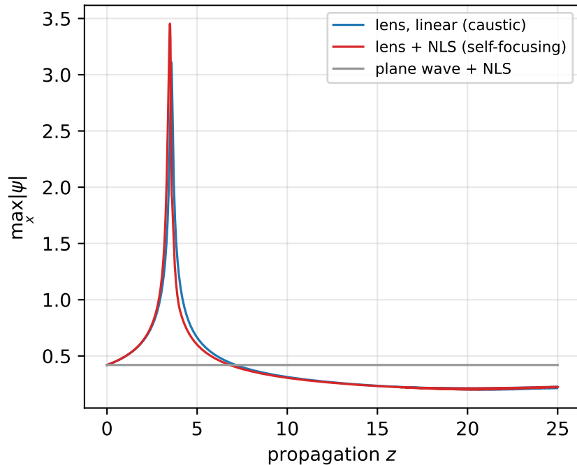
Caustic seeds self-focusing
