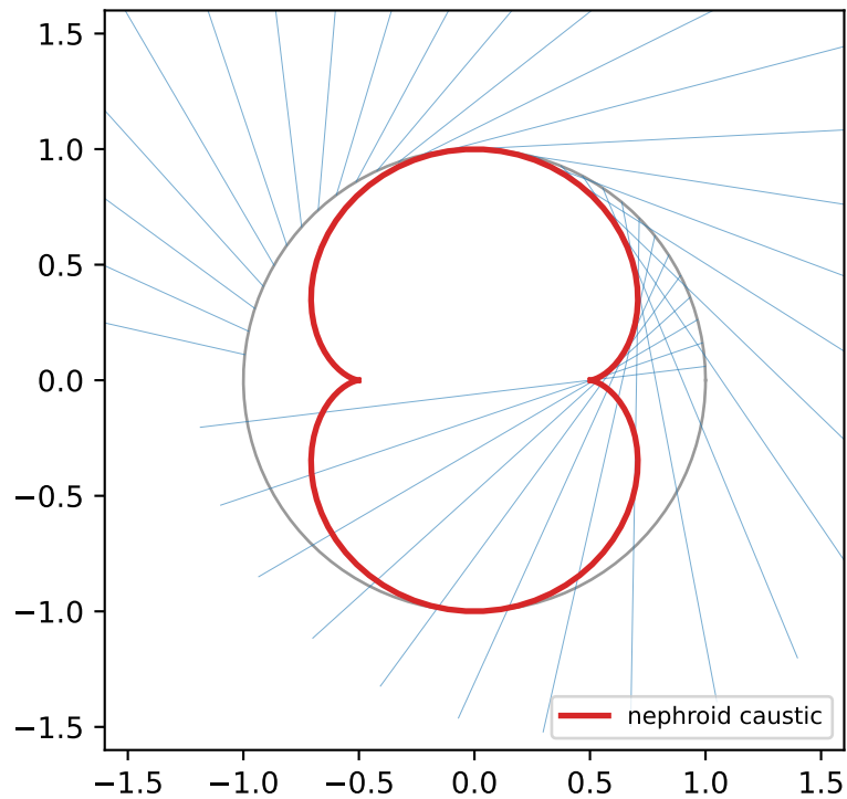
Teacup caustic (reflected rays \rightarrow nephroid)
