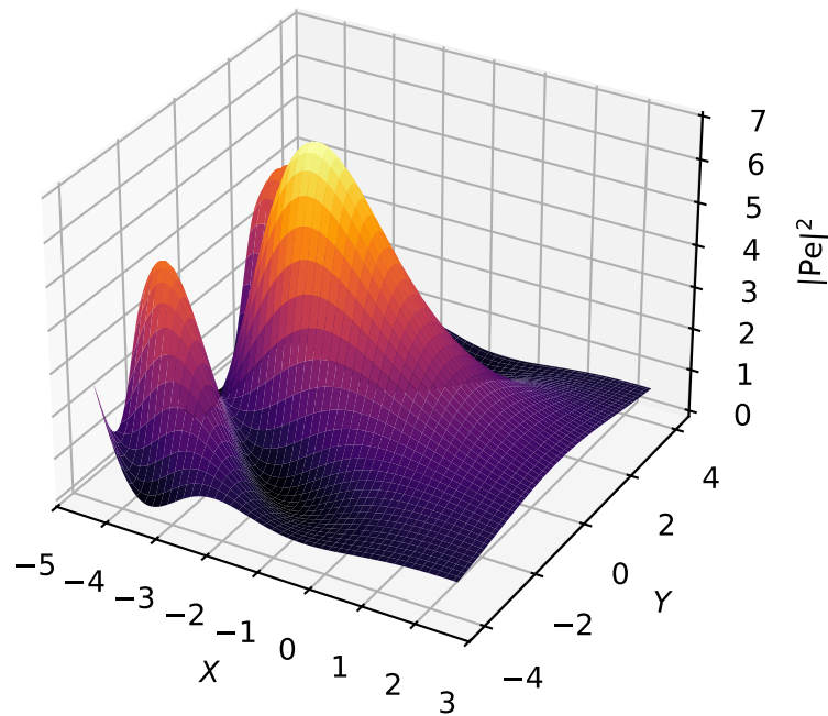
Pearcey cusp diffraction
