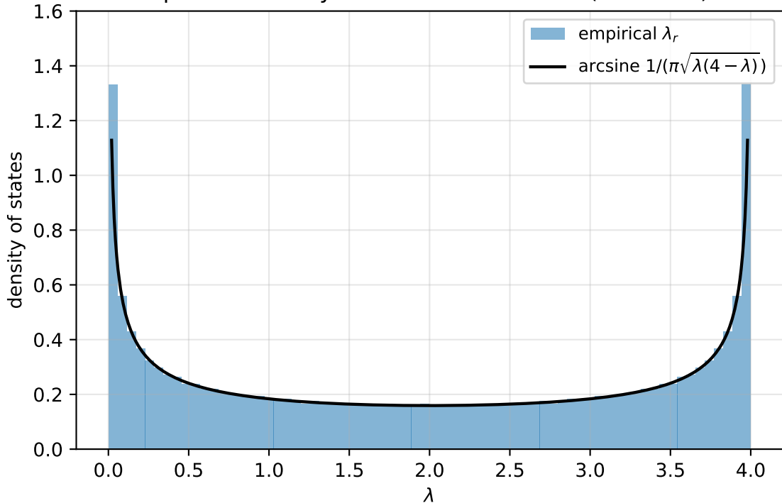
Spectral density of states: arcsine law ( N = 4000 )
