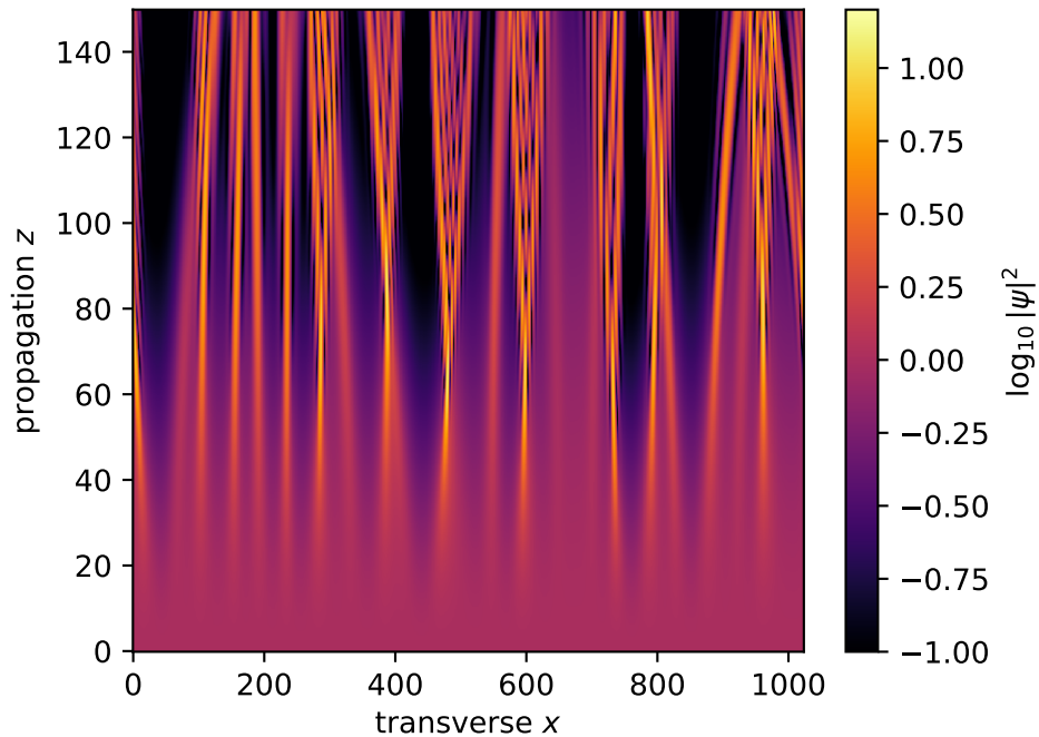
Branched flow: caustic hot spots
