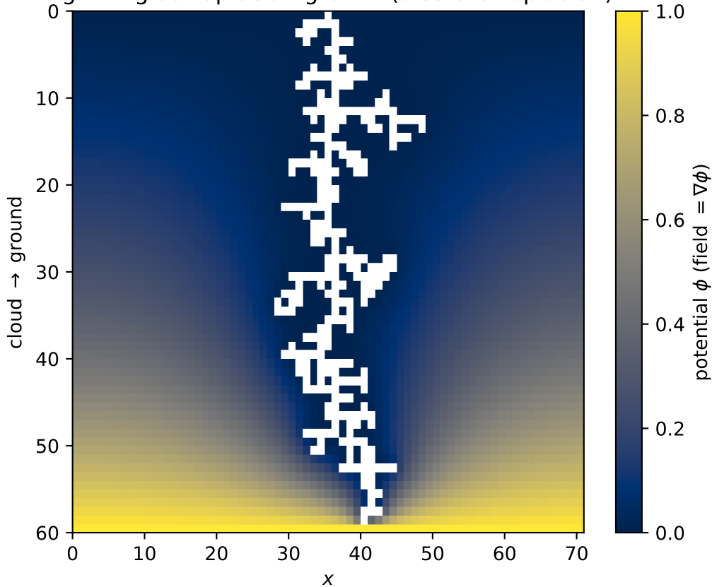
Lightning as Laplacian growth (discrete Laplacian)
