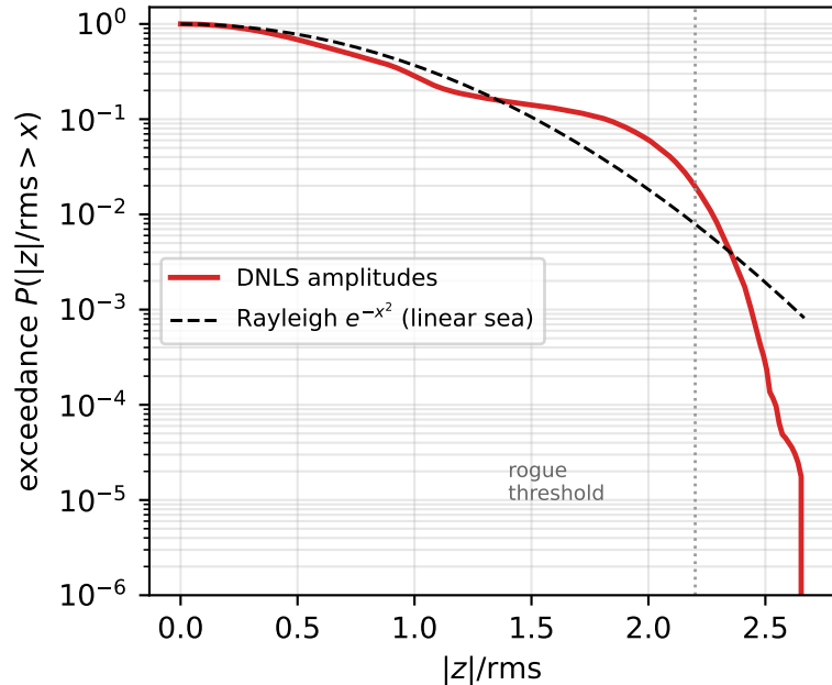
Heavy tail above the linear prediction
