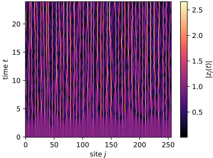
DNLS on the ring ( N = 256 ): rogue spikes
