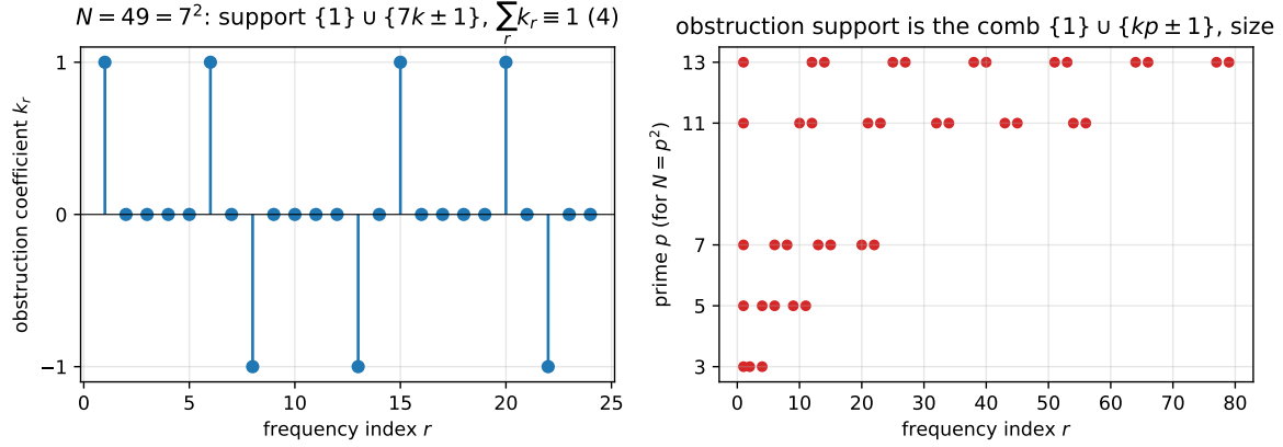
FIGURE 11. The composite obstruction for N = p^2 (Observation 17, exact/gap/prime_square.g ). Left: the GAP-computed minimal mod-4 obstruction at N = 49 ( p = 7 )—coefficients \pm 1 on the comb \{1, 6, 8, 13, 15, 20, 22\} = \{1\} \cup \{7k \pm 1\} . Right: the support comb \{1\} \cup \{kp \pm 1\} for p = 3, 5, 7, 11, 13 , of size p .
