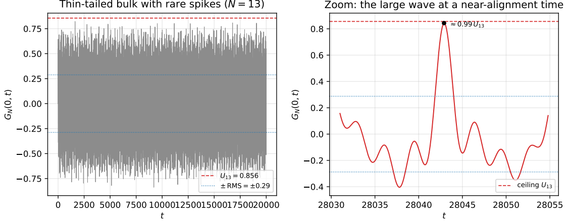
FIGURE 12. What the large wave looks like in time ( N = 13 , prime). Left: the node-0 response G_N(0, t) oscillates within the thin band \pm\text{RMS} ( \text{RMS} \approx 0.29 ) but throws rare spikes toward the ceiling U_{13} = 0.856 . Right: a zoom on the largest near-alignment spike, reaching \approx 0.99 U_N —the large wave forming as the modal phases briefly align ( verify_thesis_peaks.py ).
