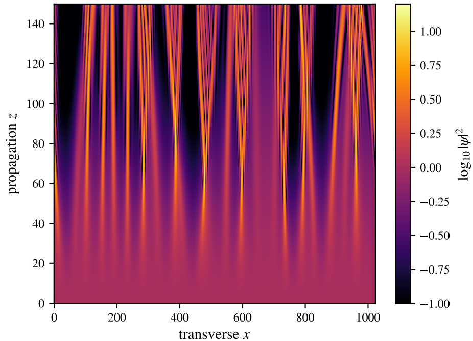
Branched flow: caustic hot spots
