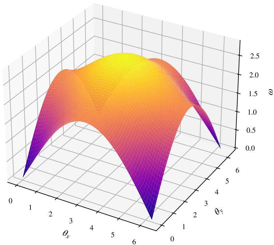
Dispersion surface \omega(\theta_x, \theta_y) on the 2-torus
