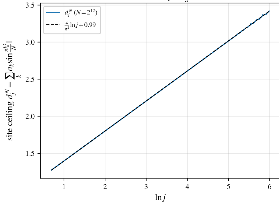
Theorem 2: d_j^N \sim \frac{4}{\pi^2} \ln j
