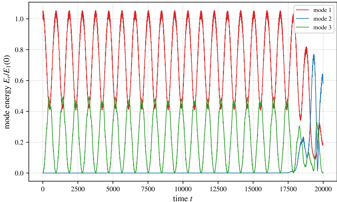
FPUT- \beta recurrence ( N=32 ): energy returns to mode 1
